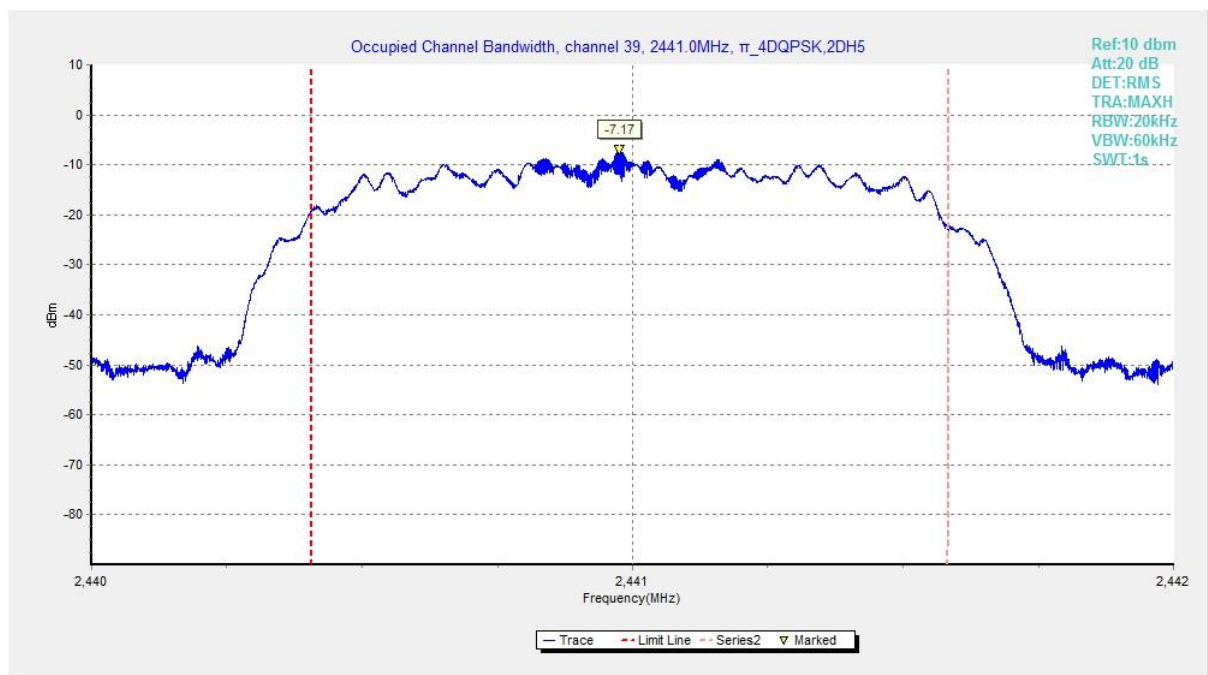
Fig. 110 Occupied Bandwidth ( \pi /4 DQPSK, Ch 39)
