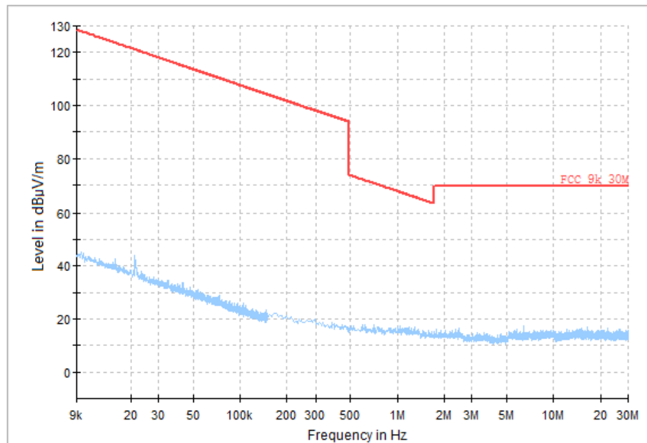
Fig. 75 Radiated Spurious Emission (All Channels, 9kHz ~ 30MHz)
