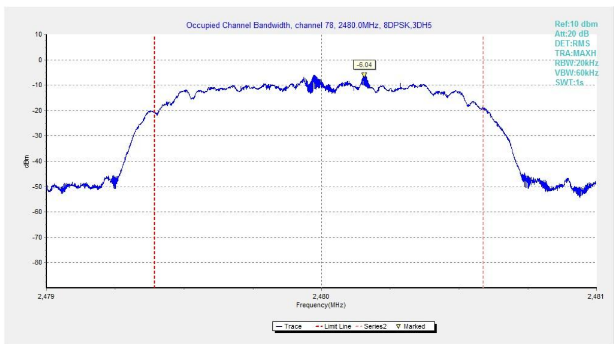
Fig. 114 Occupied Bandwidth (8DPSK, Ch 78)
