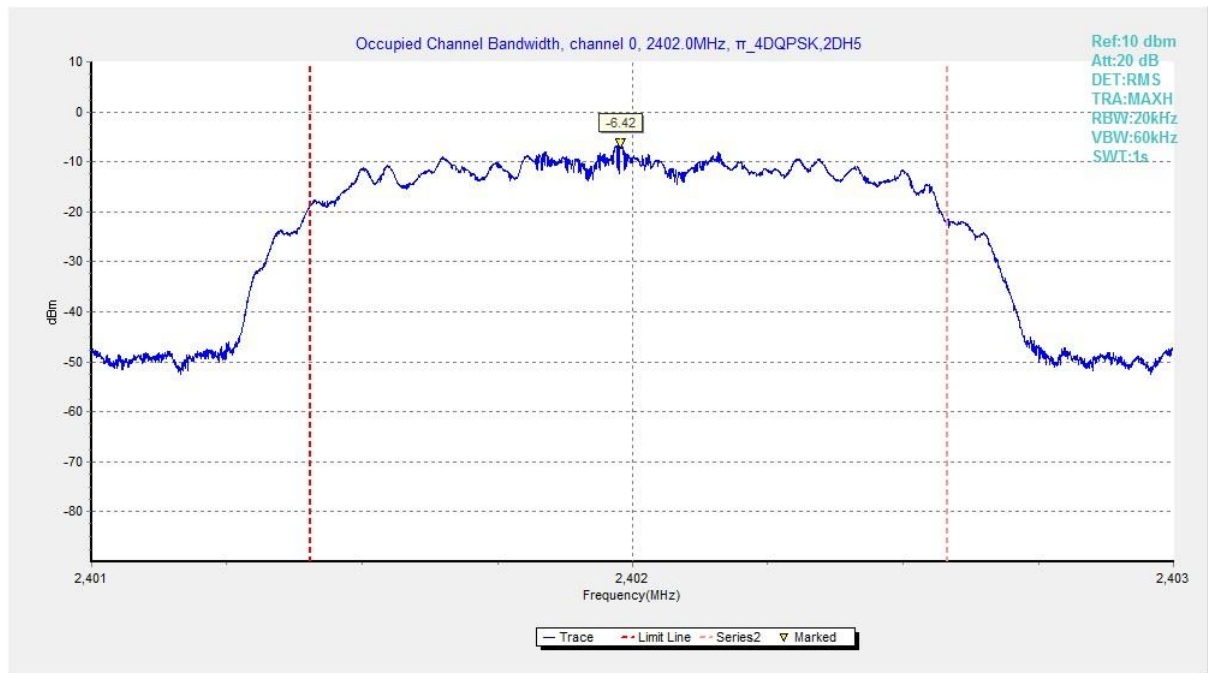
Fig. 109 Occupied Bandwidth ( \pi /4 DQPSK, Ch 0)
