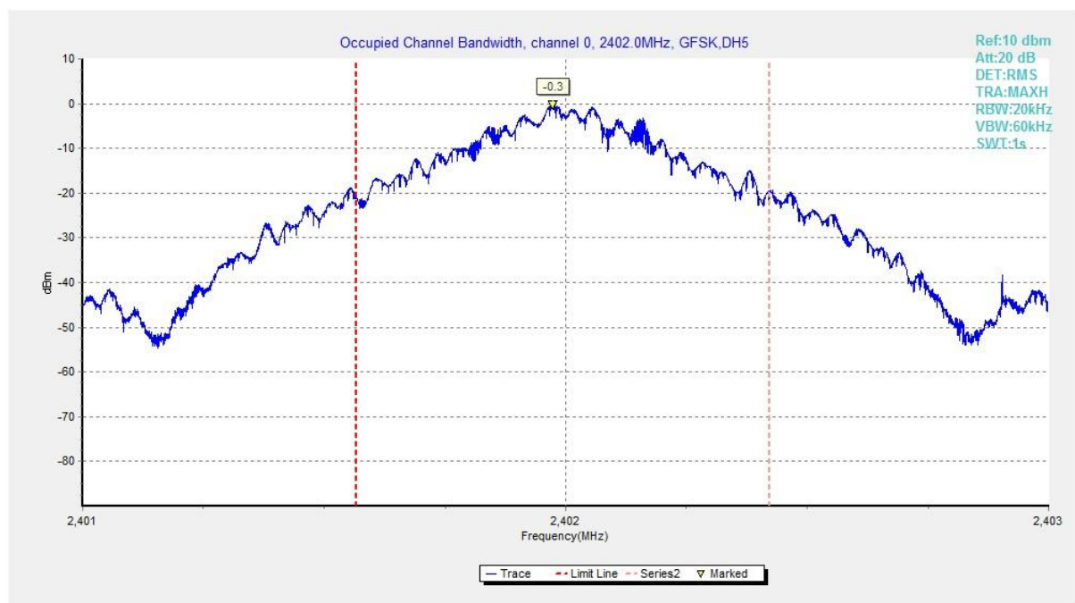
Fig. 106 Occupied Bandwidth (GFSK, Ch 0)
