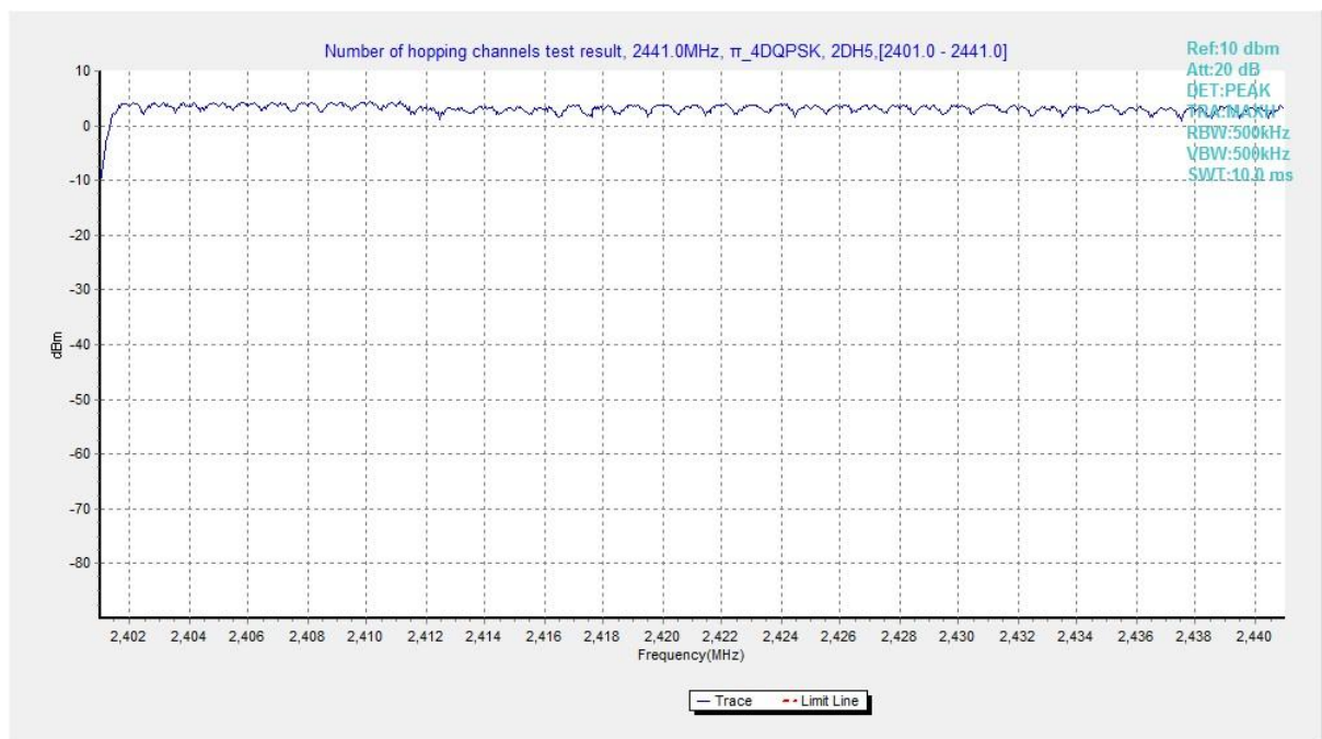
Fig. 95 Hopping channel ch0~39 ( \pi/4 DQPSK, Ch39)
