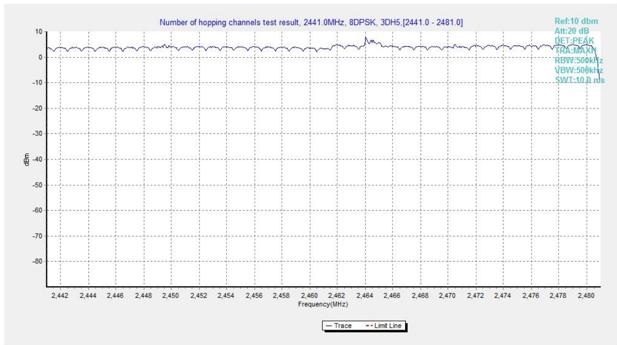
Fig. 98 Hopping channel ch40~78 (8DPSK, Ch39)
