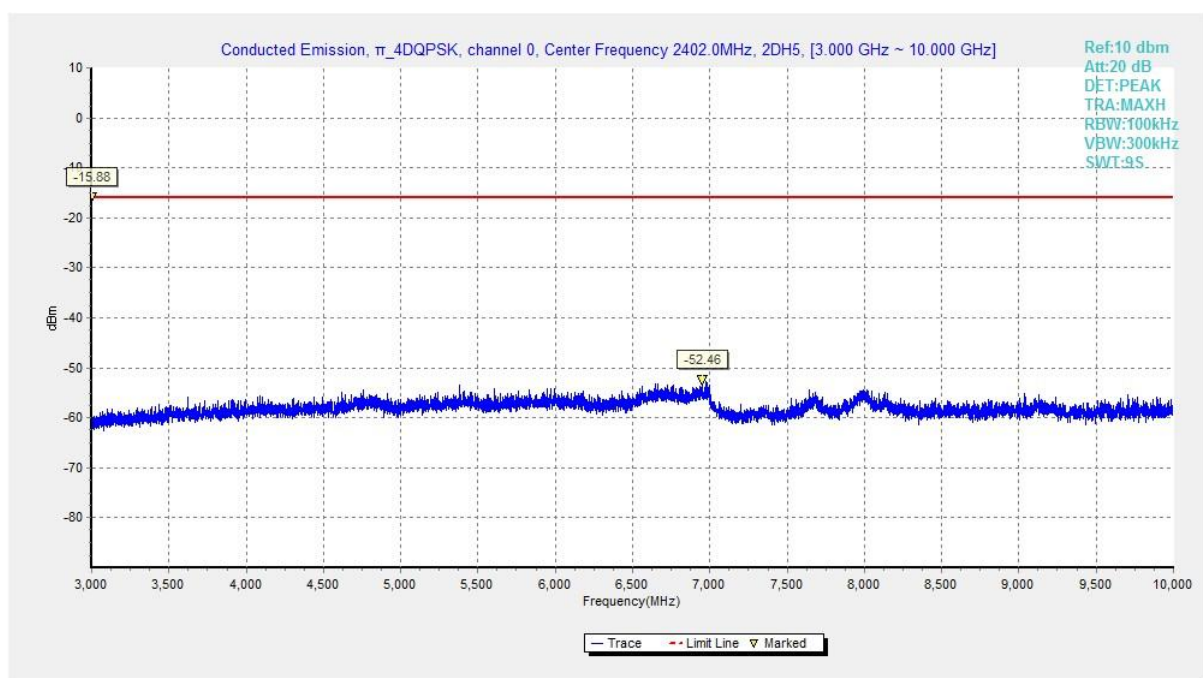
Fig. 33 Conducted Spurious Emission ( \pi/4 DQPSK, Ch0, 3GHz-10 GHz)
