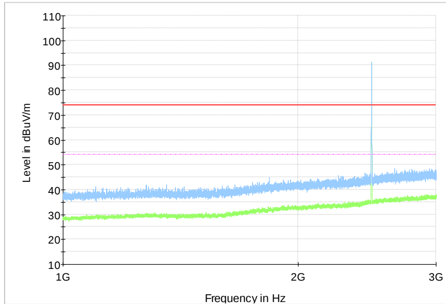
Fig. 55 Radiated Spurious Emission (GFSK, Ch78, 1GHz ~ 3GHz)
