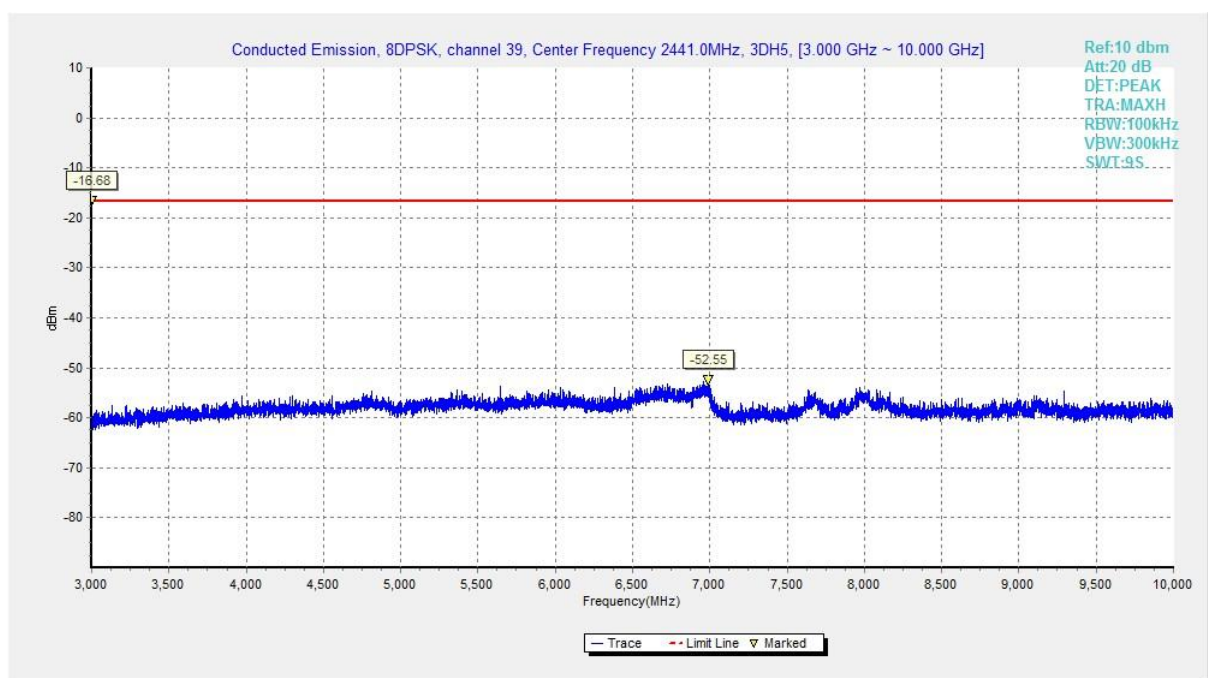
Fig. 45 Conducted Spurious Emission (8DPSK, Ch39, 3GHz-10 GHz)
