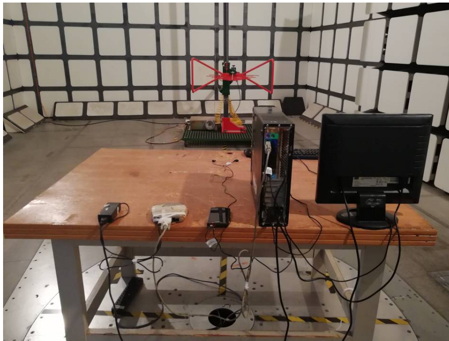
Radiated Emissions – Rear View (Below 1 GHz, Downloading Mode)
