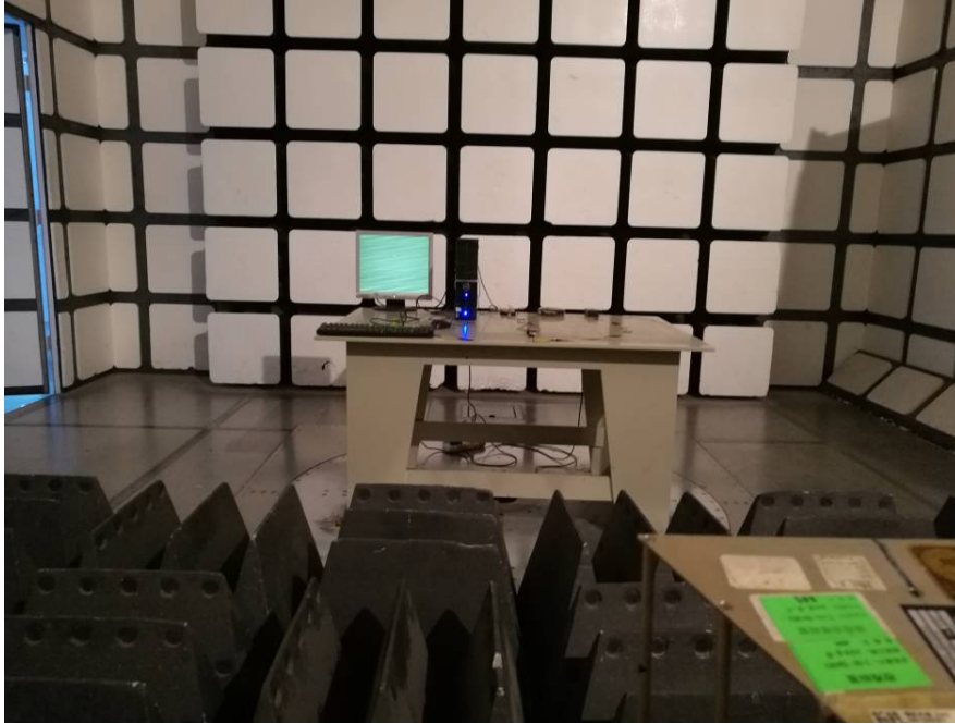
Radiated Emissions – Front View (Above 1 GHz, Downloading Mode)
