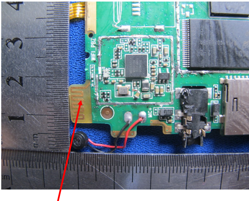
Photo 12 Appearance of PCB
