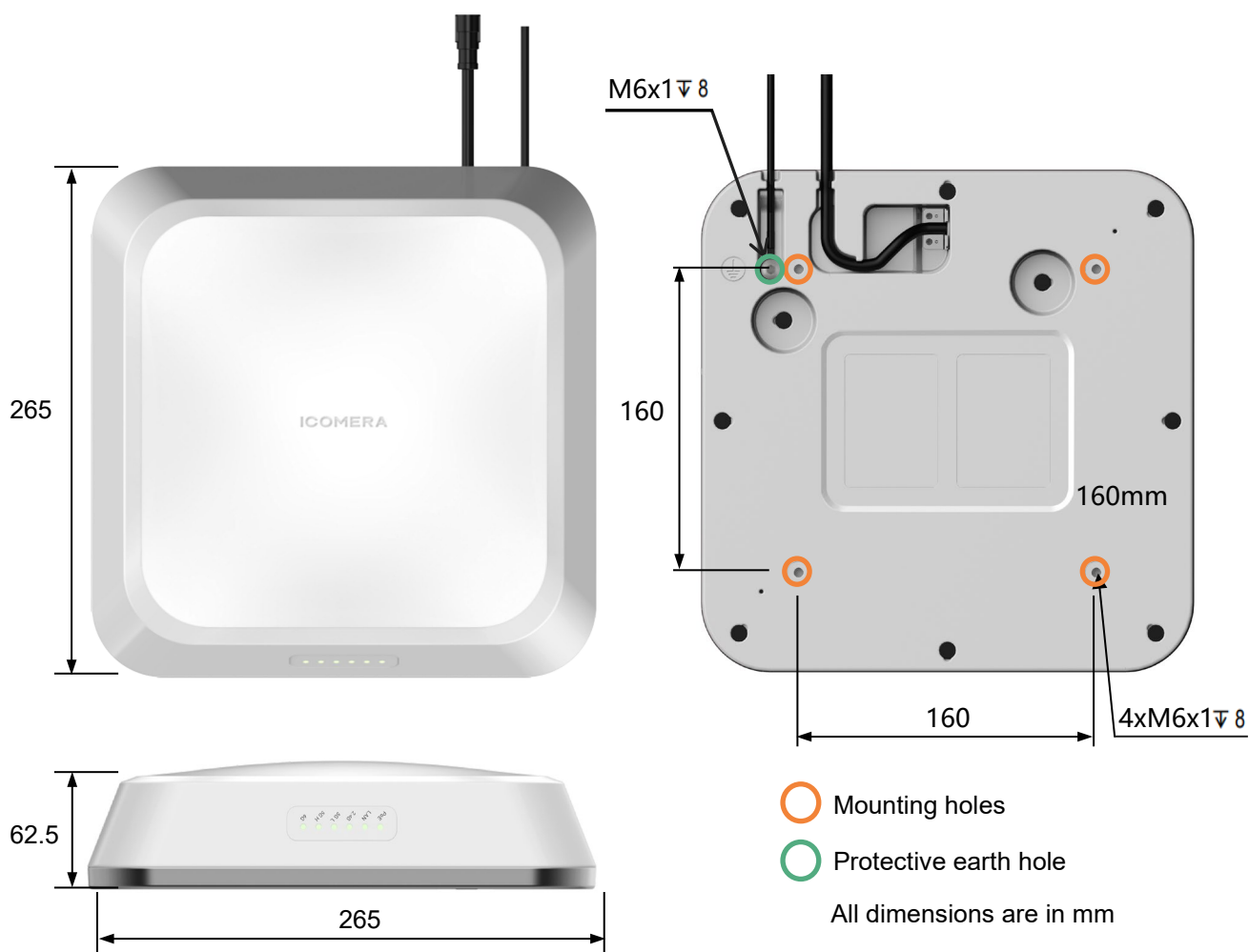
Figure 4. A2-i dimensions.
