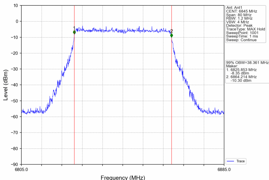
802.11ax(HEW40)_HCH_6845MHz_RU484_Left_Ant1_NTNV
