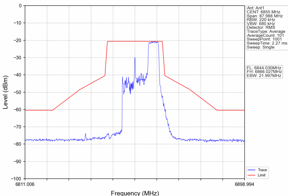
802.11ax(HEW20)_HCH_6855MHz_RU52+26_Right_Ant1_NTNV
