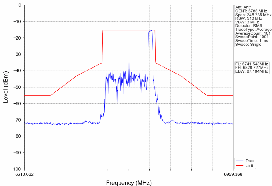
802.11ax(HEW80)_HCH_6785MHz_RU52+26_Right_Ant1_NTNV
