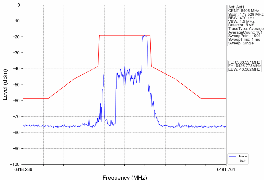
802.11ax(HEW40)_HCH_6405MHz_RU52_Right_Ant1_NTNV
