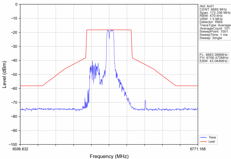
802.11ax(HEW40)_MCH_6685MHz_RU52+26_Mid_Ant1_NTNV
