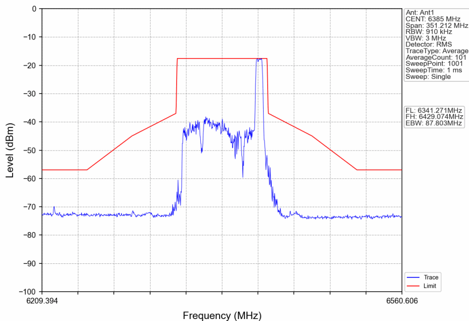
802.11ax(HEW80)_HCH_6385MHz_RU52+26_Right_Ant1_NTNV
