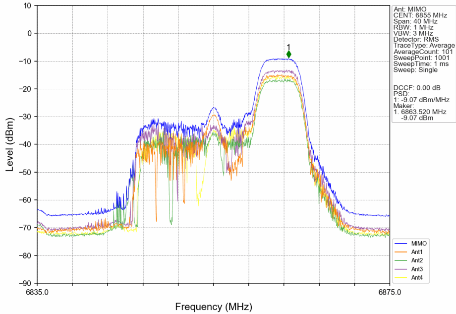
802.11ax(HEW20)_HCH_6855MHz_RU52+26_Right_MIMO_NTNV
