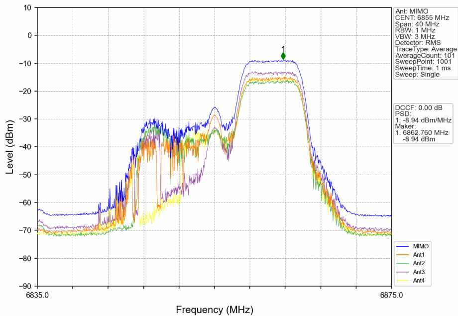
802.11ax(HEW20)_HCH_6855MHz_RU52+26_Right_MIMO_NTNV
