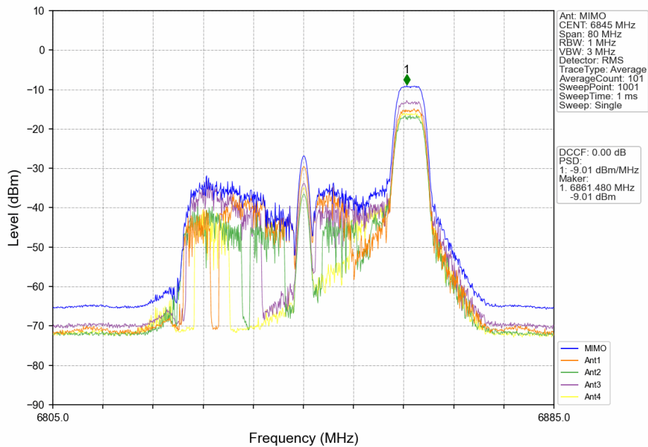
802.11ax(HEW40)_HCH_6845MHz_RU52_Right_MIMO_NTNV
