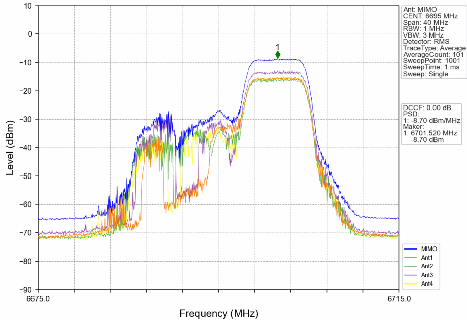
802.11ax(HEW20)_MCH_6695MHz_RU242_Left_MIMO_NTNV
