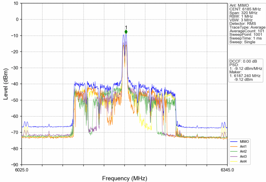
802.11ax(HEW160)_MCH_6185MHz_RU52+26_Mid_MIMO_NTNV
