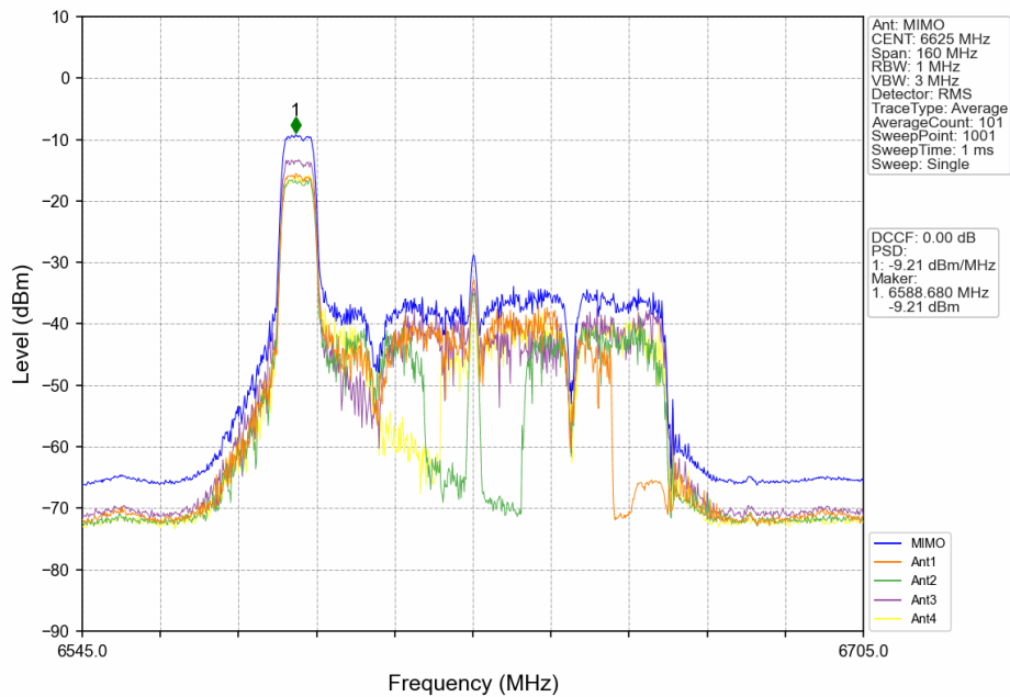
802.11ax(HEW80)_LCH_6625MHz_RU52+26_Left_MIMO_NTNV
