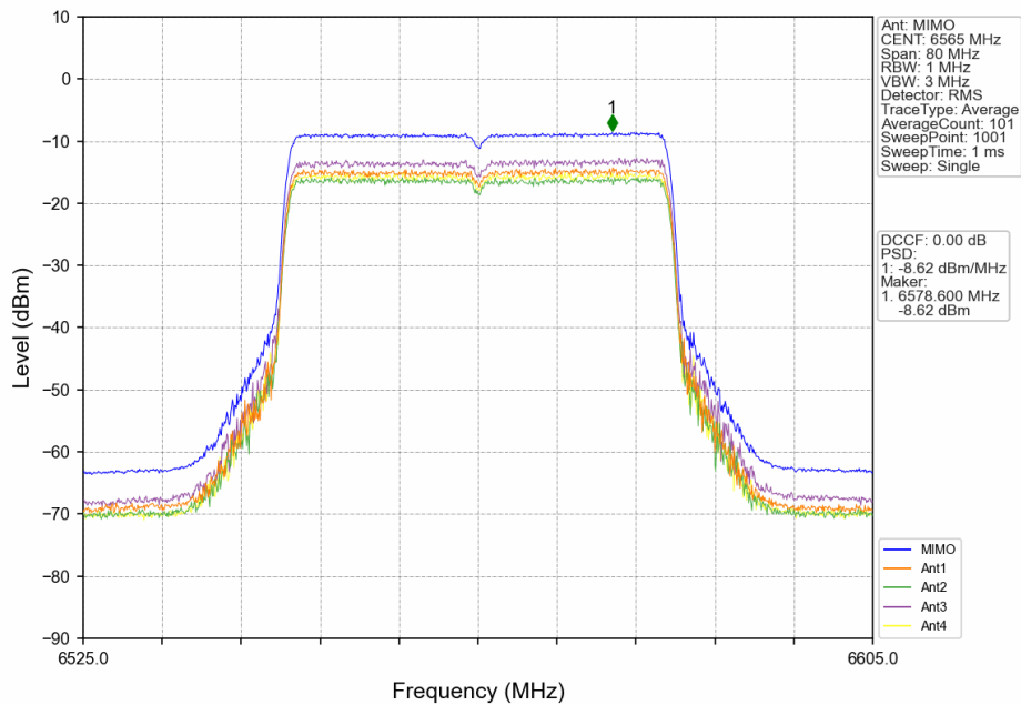
802.11ax(HEW40)_LCH_6565MHz_RU484_Left_MIMO_NTNV
