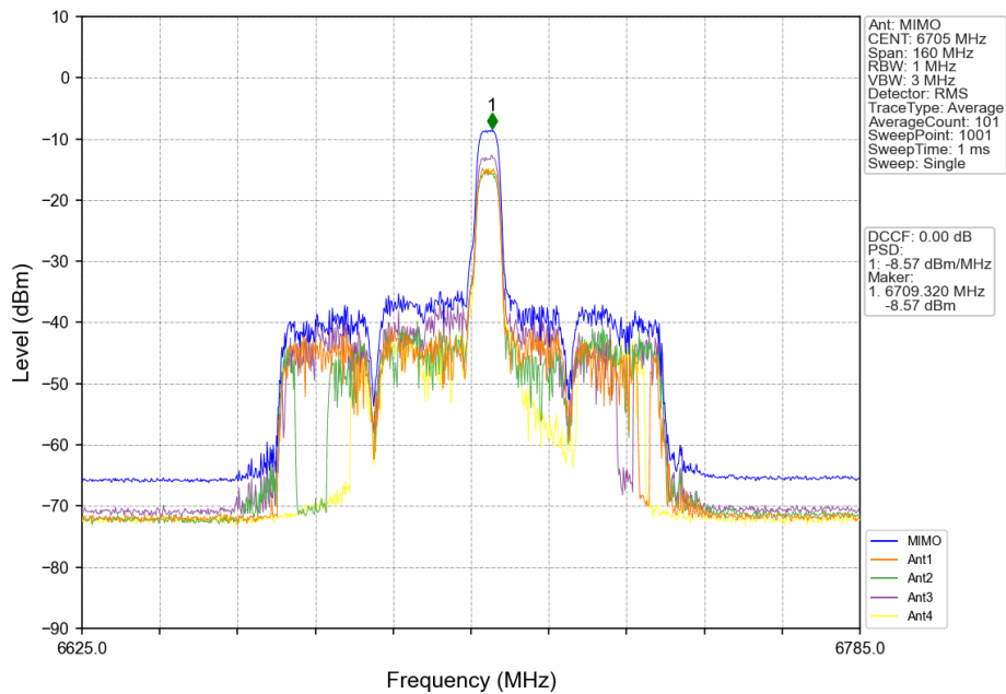
802.11ax(HEW80)_MCH_6705MHz_RU52_Mid_MIMO_NTNV
