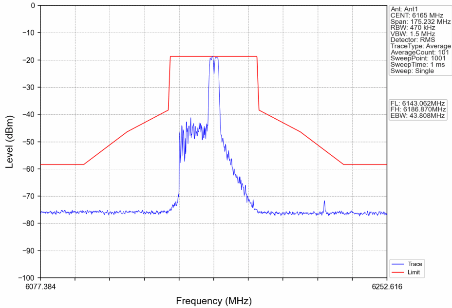
802.11ax(HEW40)_MCH_6165MHz_RU52+26_Mid_Ant1_NTNV
