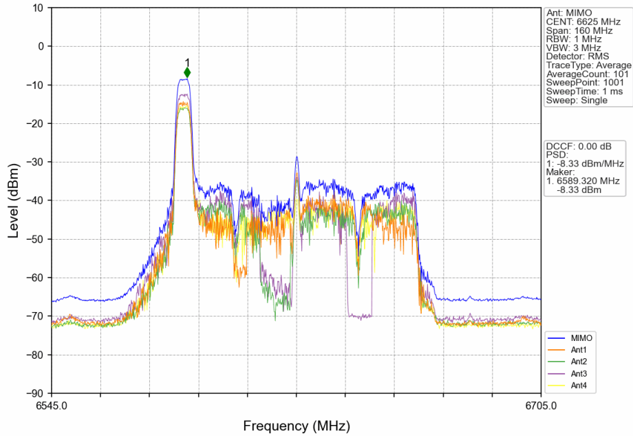
802.11ax(HEW80)_LCH_6625MHz_RU52+26_Left_MIMO_NTNV
