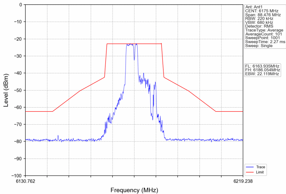
802.11ax(HEW20)_MCH_6175MHz_RU52_Mid_Ant1_NTNV
