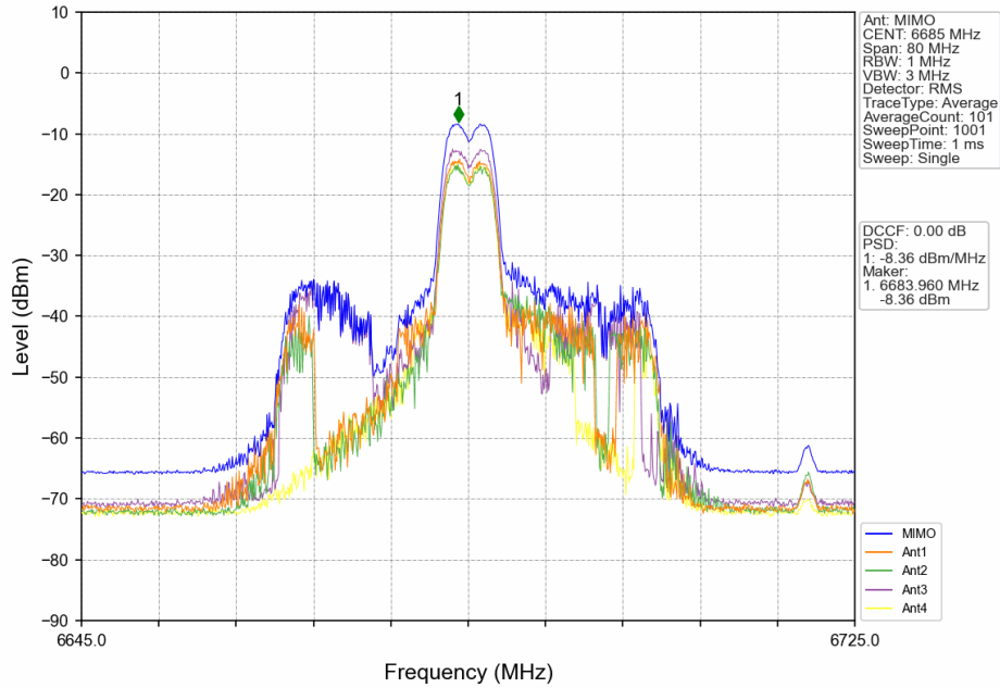
802.11ax(HEW40)_MCH_6685MHz_RU52+26_Mid_MIMO_NTNV
