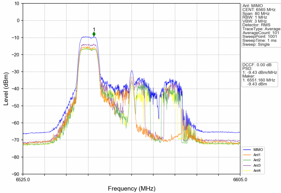
802.11ax(HEW40)_LCH_6565MHz_RU484_Left_MIMO_NTNV
