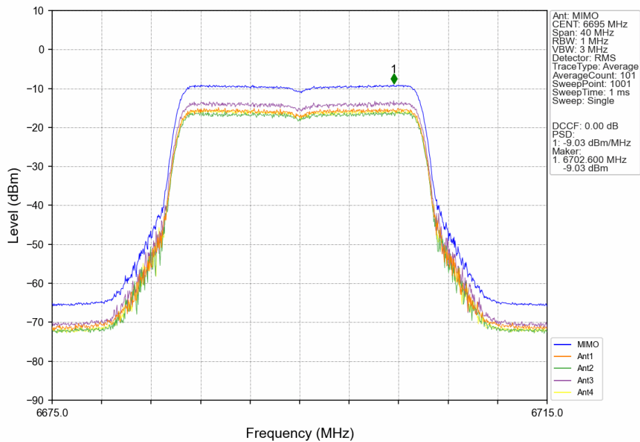
802.11ax(HEW20)_MCH_6695MHz_RU242_Left_MIMO_NTNV
