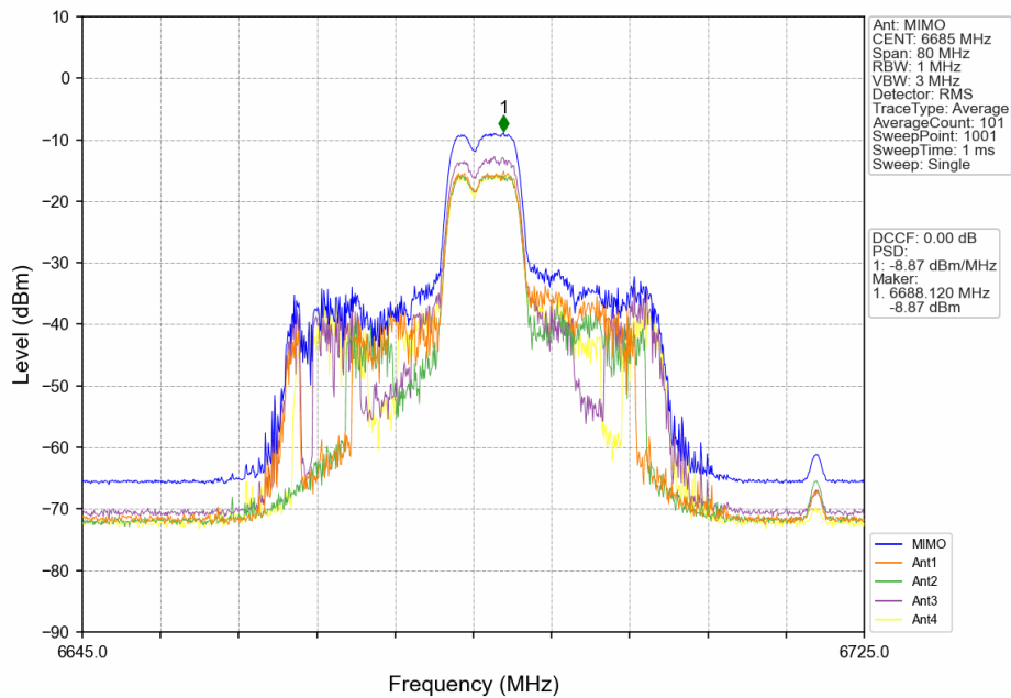
802.11ax(HEW40)_MCH_6685MHz_RU52+26_Mid_MIMO_NTNV
