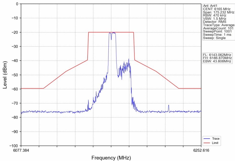
802.11ax(HEW40)_MCH_6165MHz_RU52+26_Mid_Ant1_NTNV
