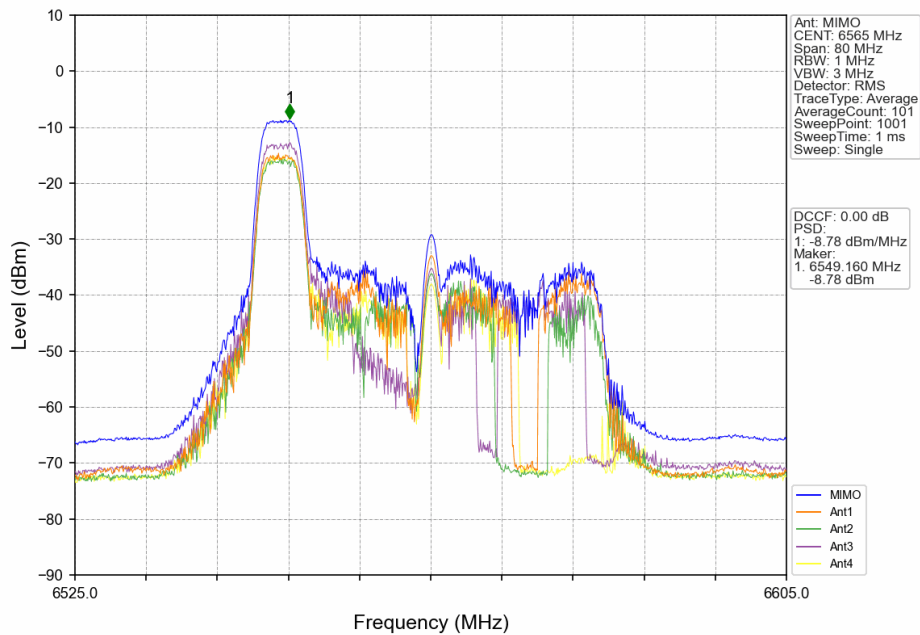
802.11ax(HEW40)_LCH_6565MHz_RU52_Left_MIMO_NTNV
