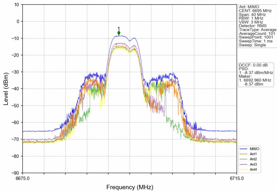
802.11ax(HEW20)_MCH_6695MHz_RU52_Mid_MIMO_NTNV
