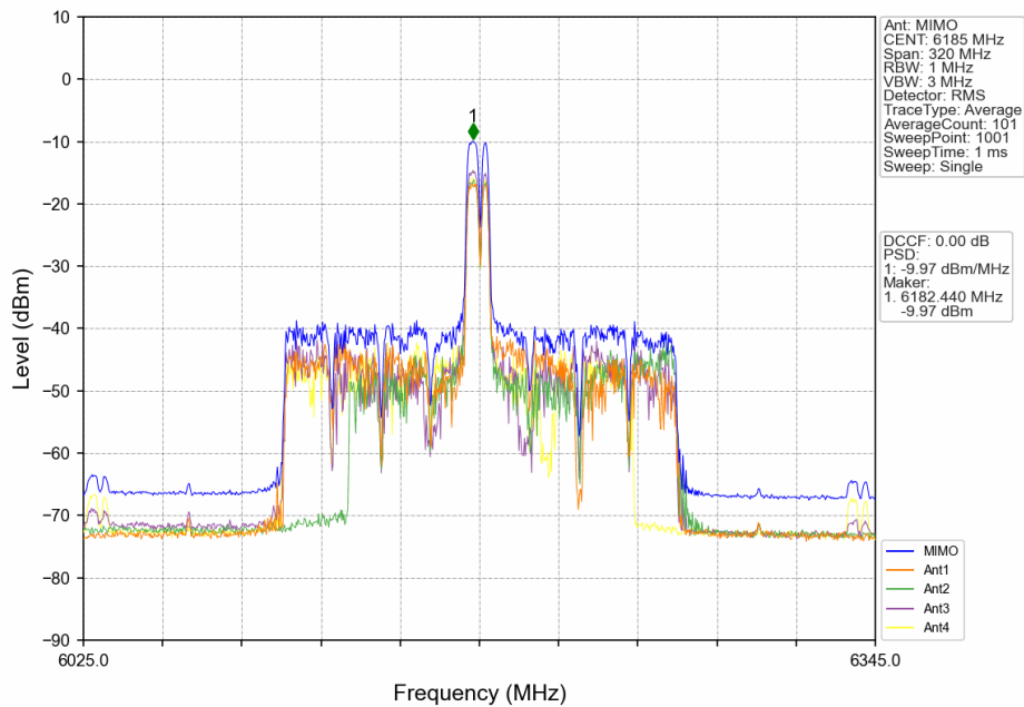
802.11ax(HEW160)_MCH_6185MHz_RU52+26_Mid_MIMO_NTNV
