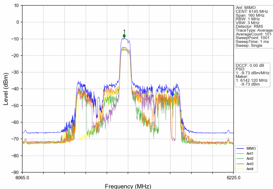
802.11ax(HEW80)_MCH_6145MHz_RU996_Left_MIMO_NTNV
