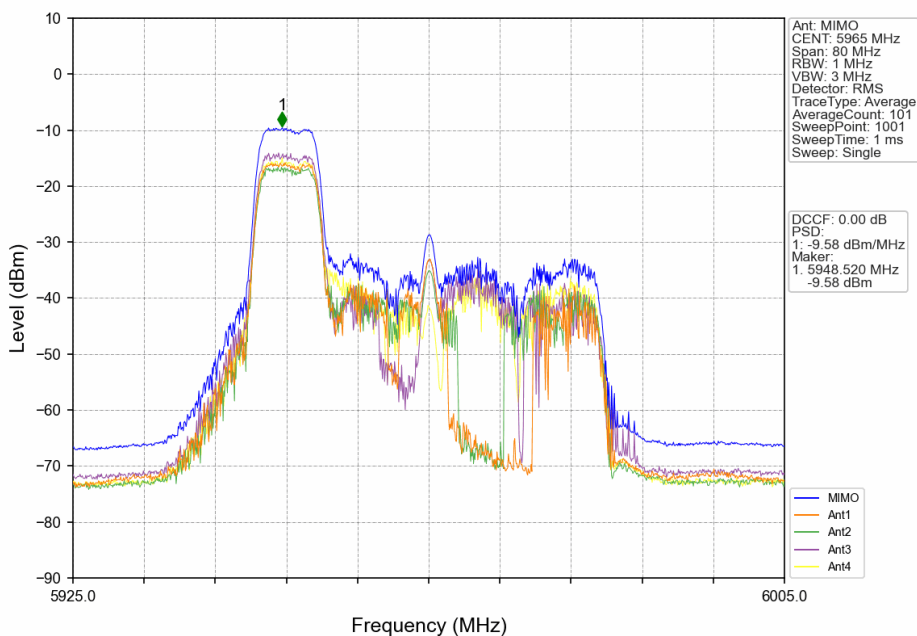
802.11ax(HEW40)_LCH_5965MHz_RU484_Left_MIMO_NTNV
