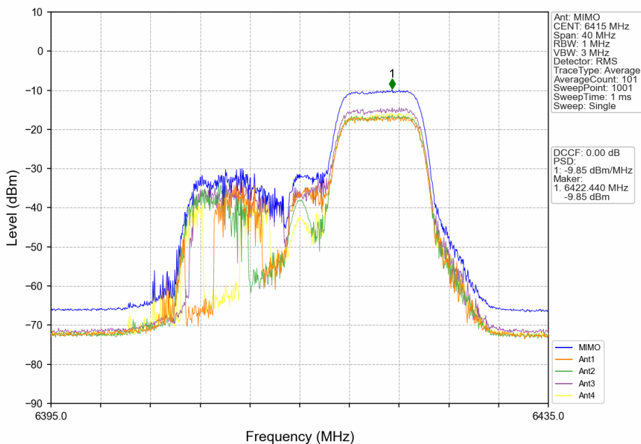
802.11ax(HEW20)_HCH_6415MHz_RU52+26_Right_MIMO_NTNV
