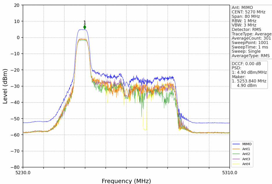
802.11ax(HEW40)_LCH_5270MHz_RU52_Left_MIMO_NTNV
