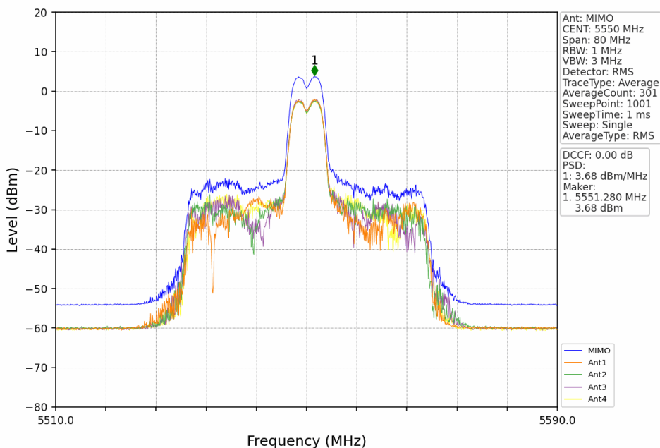
802.11ax(HEW40)_MCH_5550MHz_RU52_Mid_MIMO_NTNV
