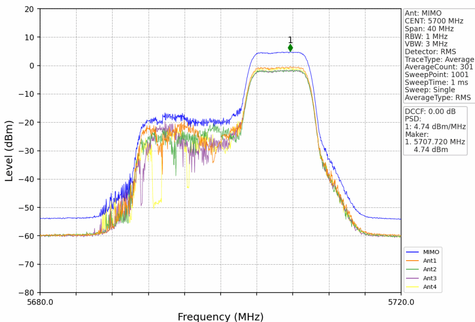
802.11ax(HEW20)_HCH_5700MHz_RU52_Right_MIMO_NTNV
