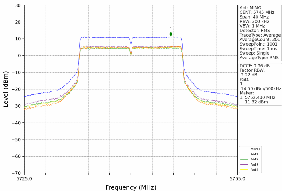
802.11ax(HEW20)_LCH_5745MHz_RU242_Left_MIMO_NTNV
