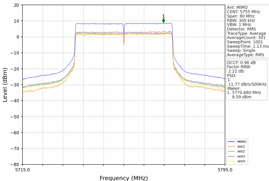
802.11ax(HEW40)_LCH_5755MHz_RU484_Left_MIMO_NTNV
