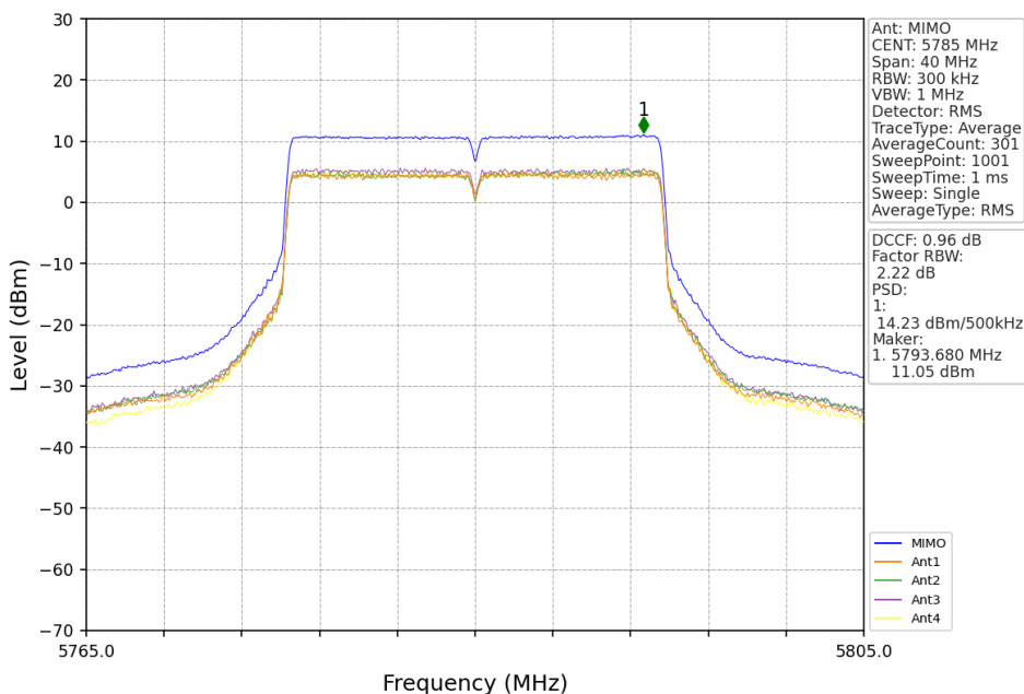
802.11ax(HEW20)_MCH_5785MHz_RU242_Left_MIMO_NTNV
