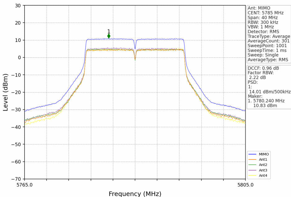
802.11ac(VHT20)_MCH_5785MHz_MIMO_NTNV
