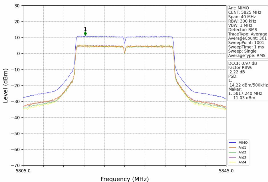
802.11ax(HEW20)_HCH_5825MHz_RU242_Left_MIMO_NTNV
