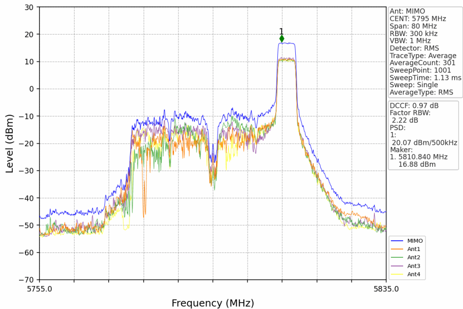
802.11ax(HEW40)_HCH_5795MHz_RU484_Left_MIMO_NTNV
