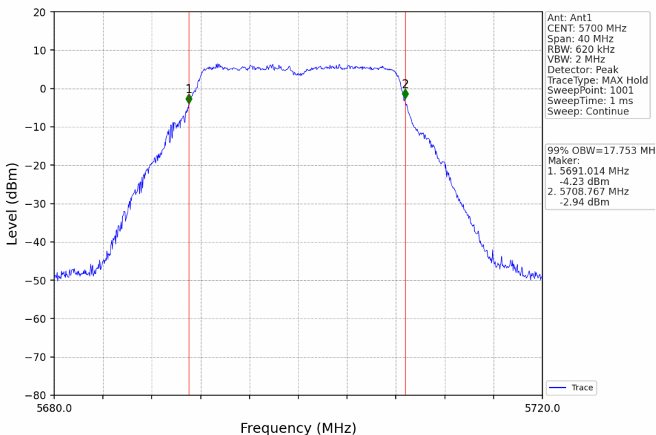
802.11a_HCH_5700MHz_Ant1_NTNV
