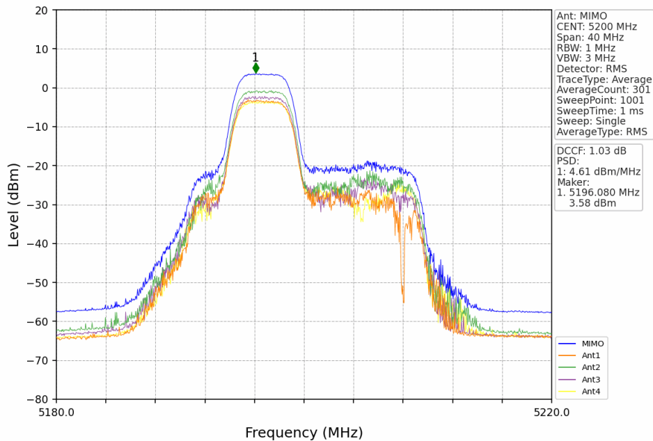
802.11ax(HEW20)_MCH_5200MHz_RU242_Left_MIMO_NTNV
