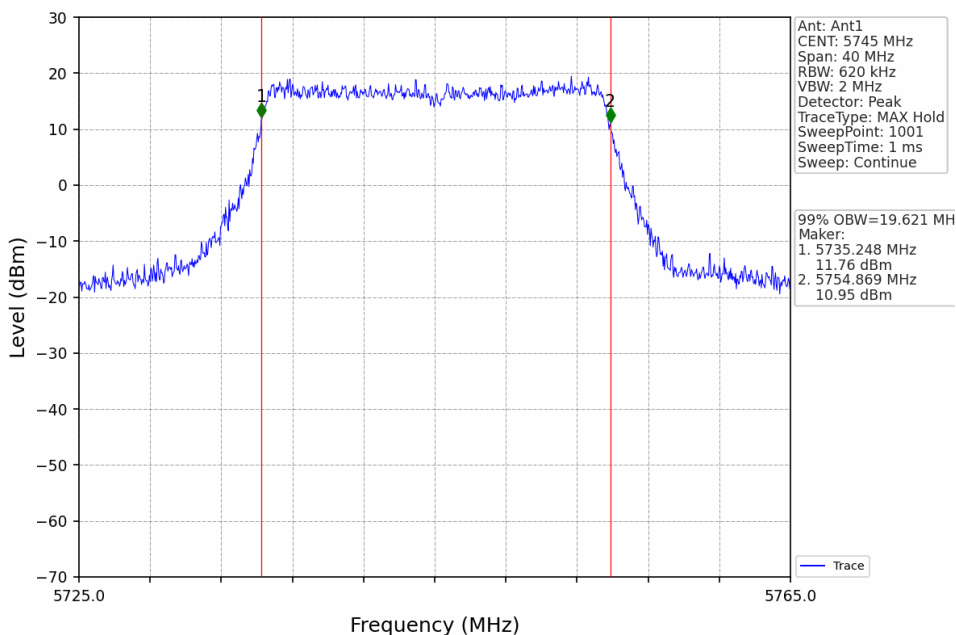
802.11ax(HEW20)_LCH_5745MHz_RU242_Left_Ant1_NTNV
