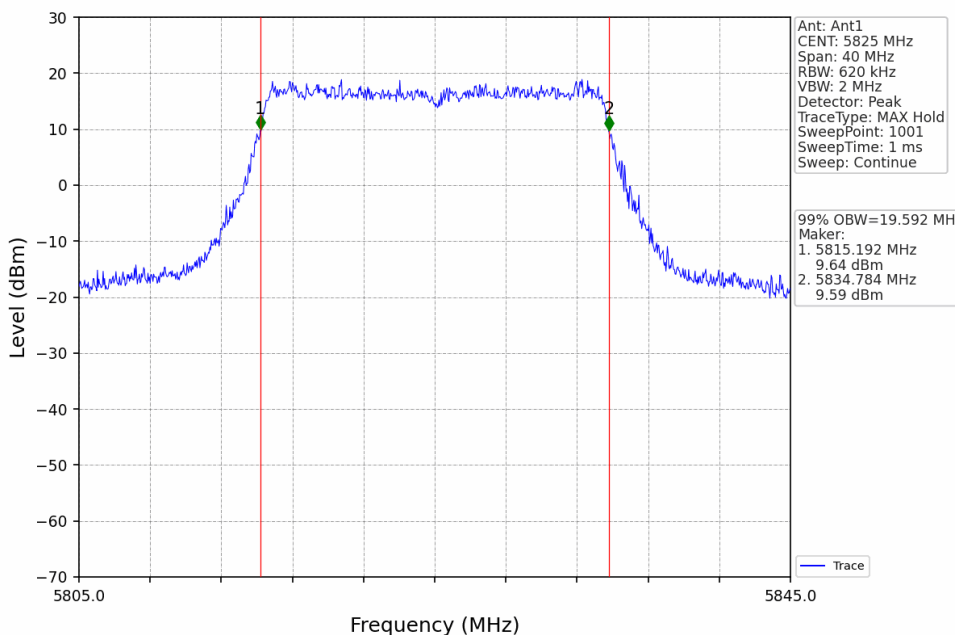
802.11ax(HEW20)_HCH_5825MHz_RU242_Left_Ant1_NTNV
