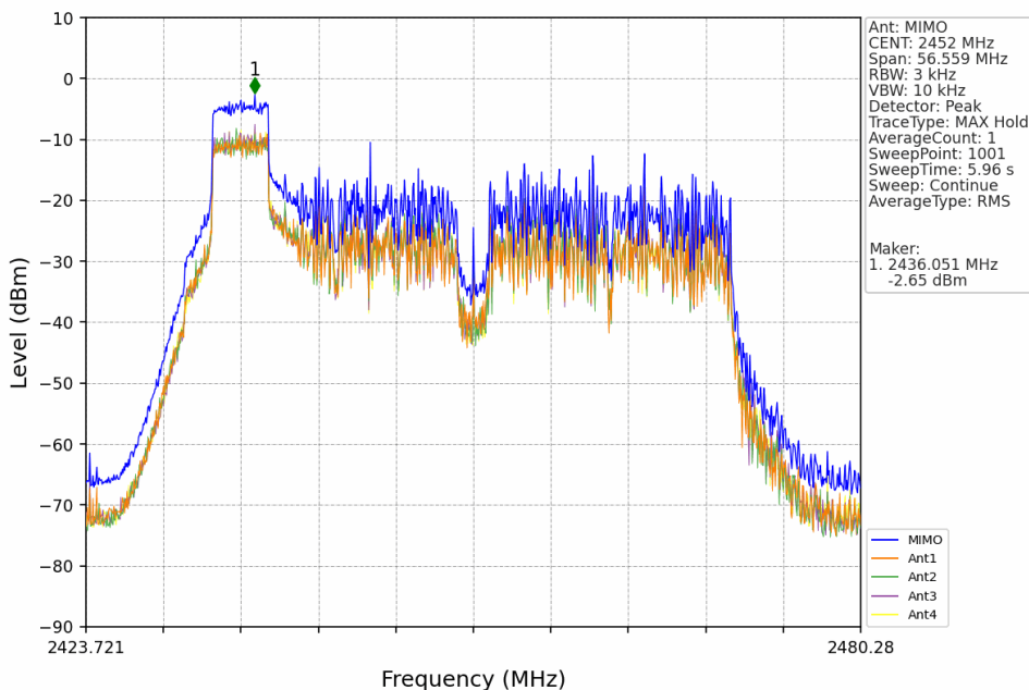
802.11ax(HEW40)_HCH_2452MHz_RU52_Mid_MIMO_NTNV
