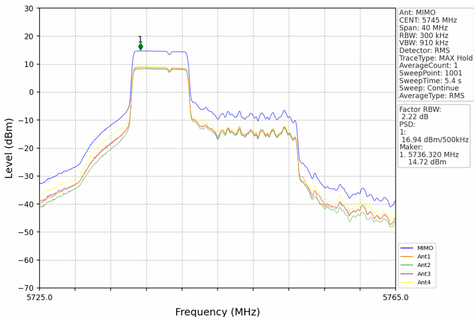
802.11ax(HEW20) LCH 5745MHz RU52+26 Left MIMO NTN
