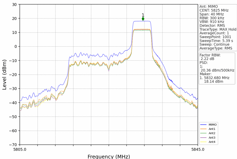
802.11ax(HEW20) HCH 5825MHz RU52+26 Right MIMO NTN
