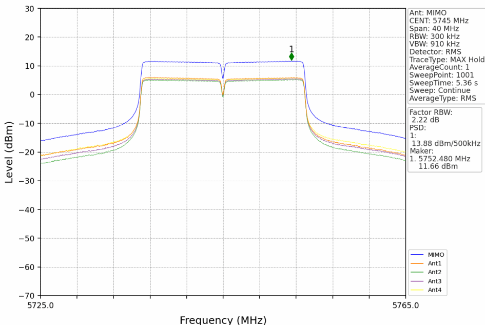
802.11n(HT20)_LCH_5745MHz_MIMO_NTNV
