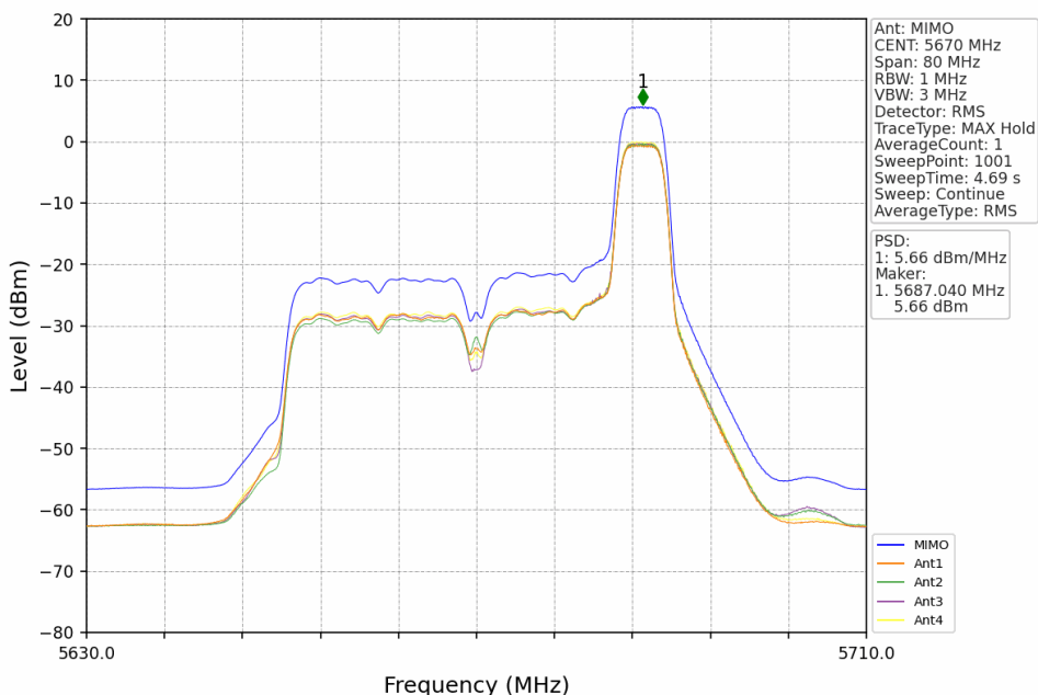
802.11be(EHT40)_HCH_5670MHz_RU52+26_Right_MIMO_NTNV
