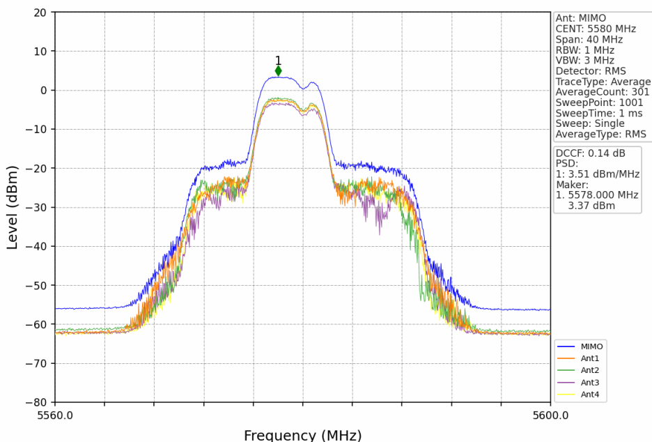
802.11be(EHT20)_MCH_5580MHz_RU52+26_Mid_MIMO_NTNV
