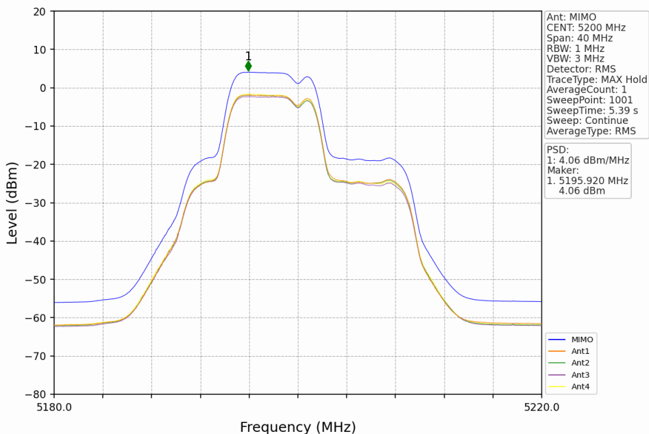
802.11be(EHT20)_MCH_5200MHz_RU52+26_Mid_MIMO_NTNV
