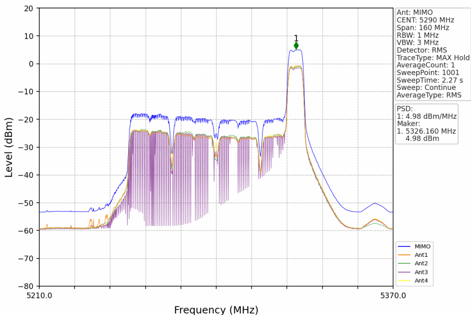
802.11ax(HEW80) MCH 5290MHz RU52+26 Right MIMO NTNV
