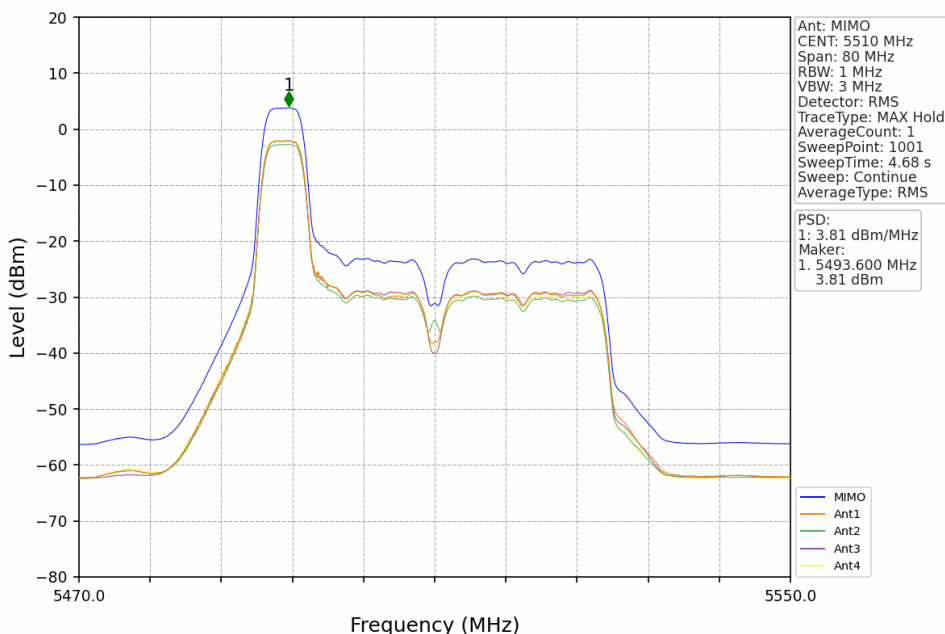
802.11ax(HEW40) LCH 5510MHz RU52+26 Left MIMO NTN
