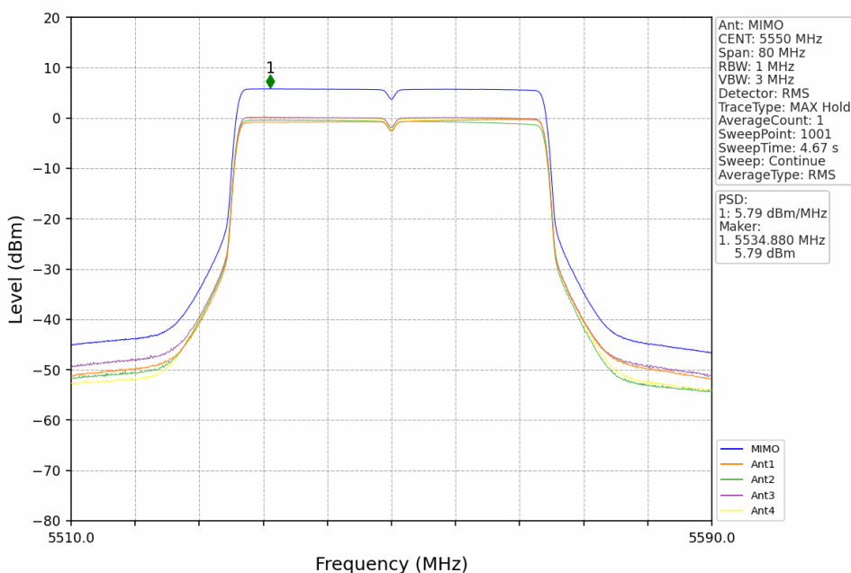
802.11ax(HEW40) MCH 5550MHz RU484 Left MIMO NTN
