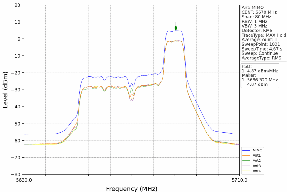
802.11ax(HEW40) HCH 5670MHz RU52+26 Right MIMO NTN
