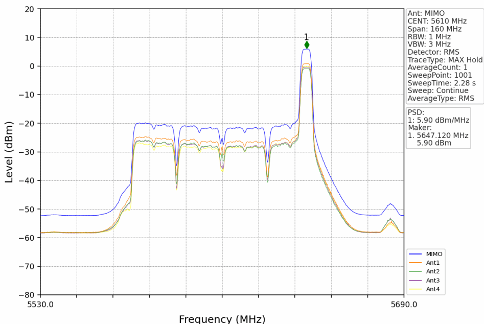
802.11ax(HEW80) HCH 5610MHz RU52+26 Right MIMO NTN
