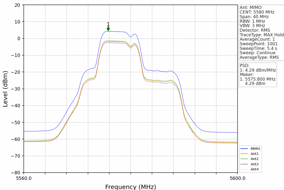
802.11ax(HEW20)_MCH_5580MHz_RU52+26_Mid_MIMO_NTNV
