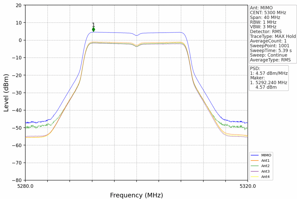
802.11ac(VHT20)_MCH_5300MHz_MIMO_NTNV
