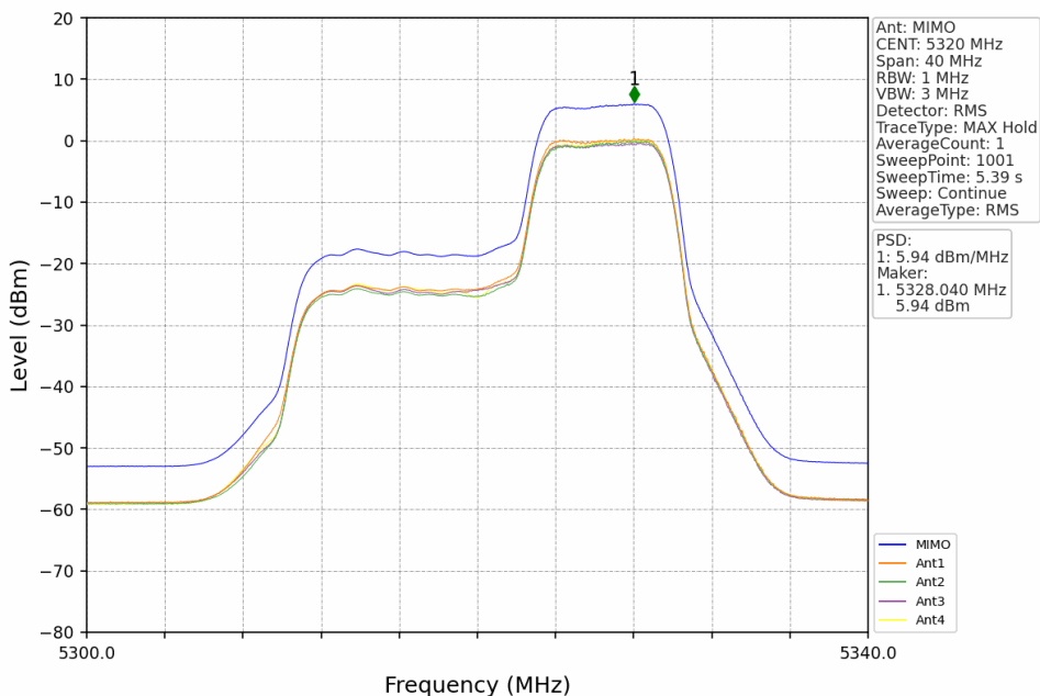
802.11ax(HEW20) HCH 5320MHz RU52+26 Right MIMO NTN
