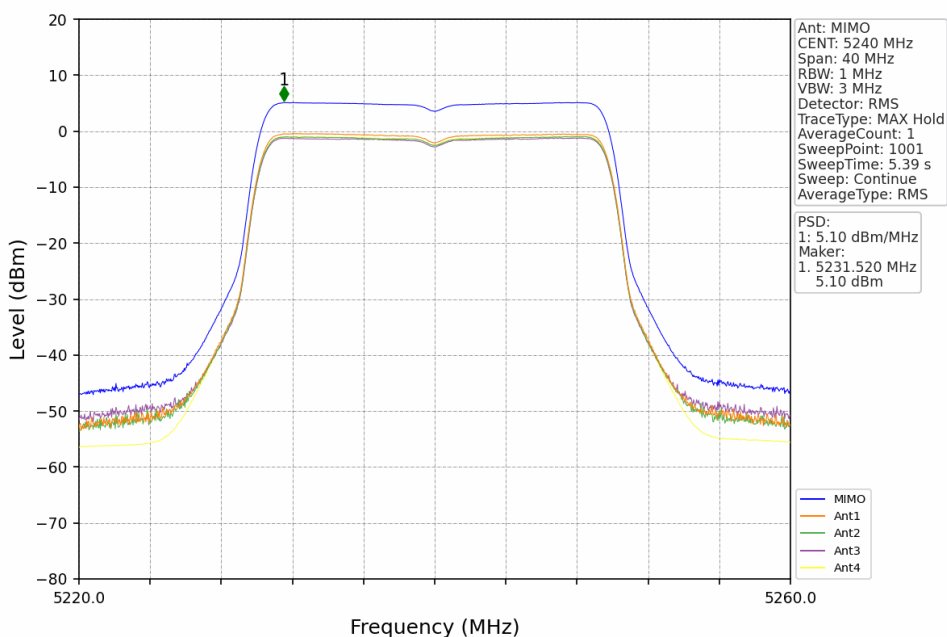
802.11ax(HEW20)_HCH_5240MHz_RU242_Left_MIMO_NTNV
