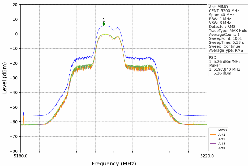
802.11ax(HEW20)_MCH_5200MHz_RU52+26_Mid_MIMO_NTNV
