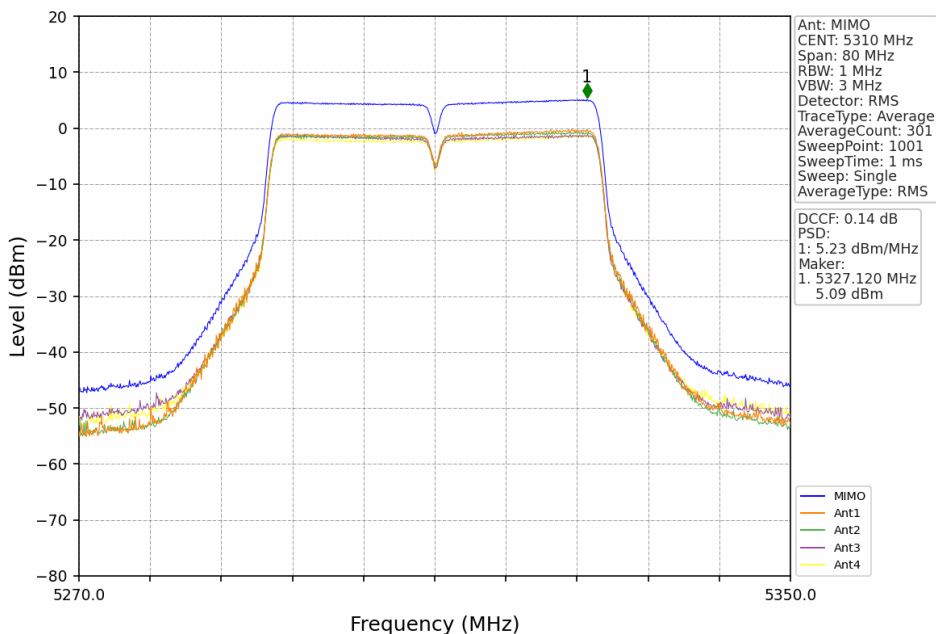
802.11ac(VHT40)_HCH_5310MHz_MIMO_NTNV
