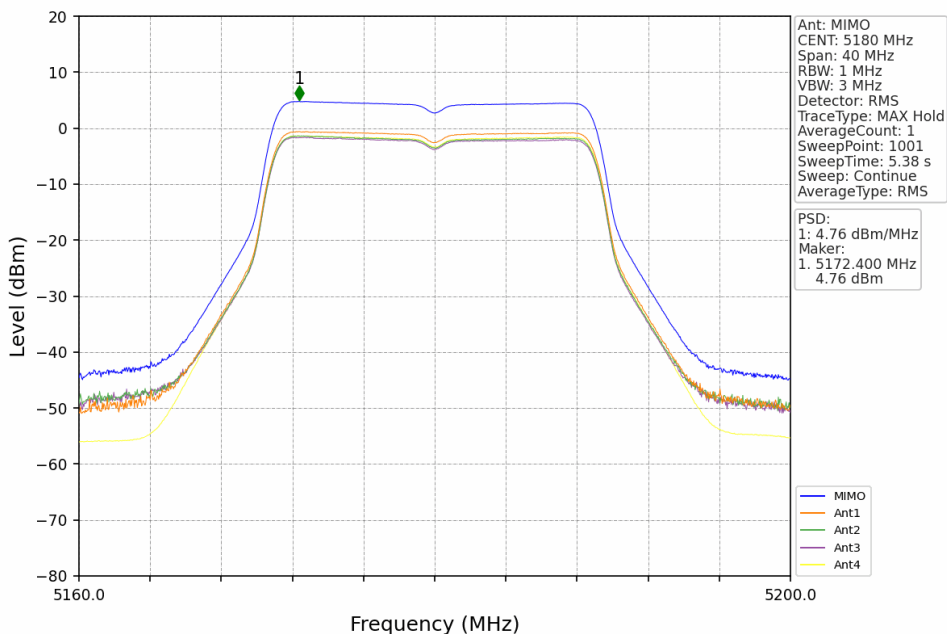
802.11ac(VHT20)_LCH_5180MHz_MIMO_NTNV
