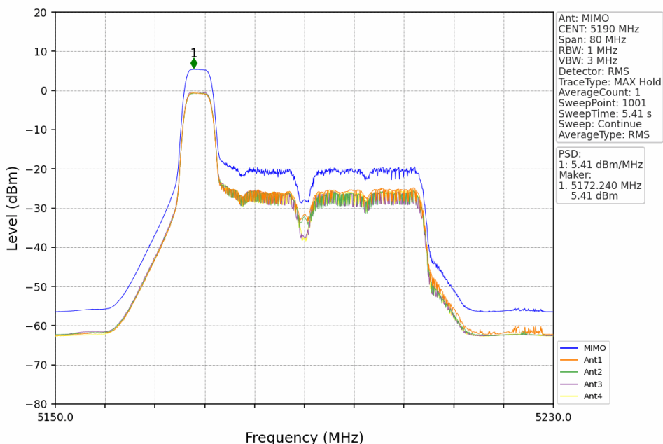
802.11ax(HEW40) LCH 5190MHz RU52+26 Left MIMO NTN
