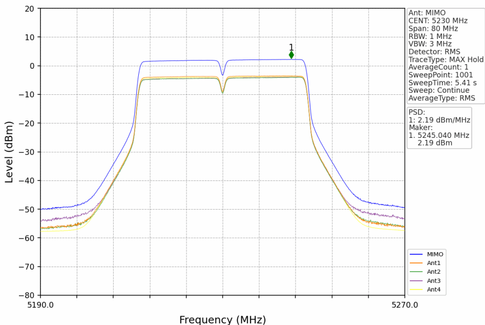
802.11ac(VHT40)_HCH_5230MHz_MIMO_NTNV
