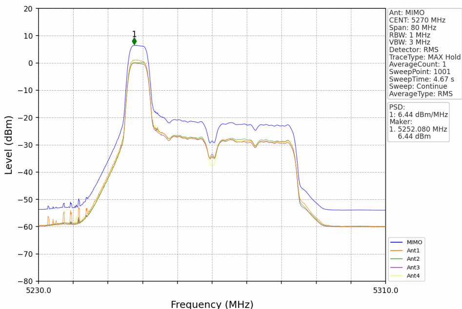
802.11ax(HEW40) LCH 5270MHz RU52+26 Left MIMO NTN
