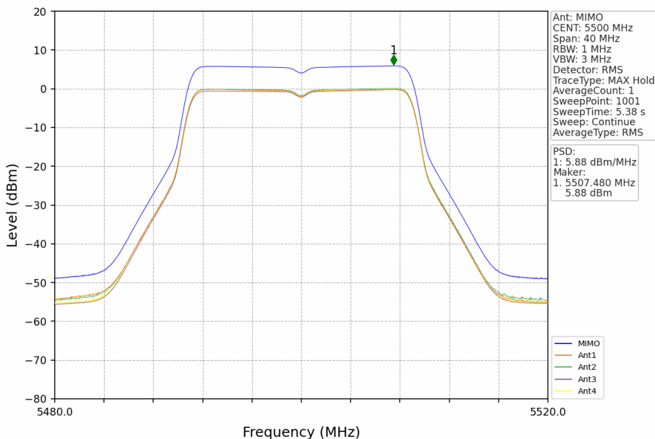
802.11ac(VHT20)_LCH_5500MHz_MIMO_NTNV
