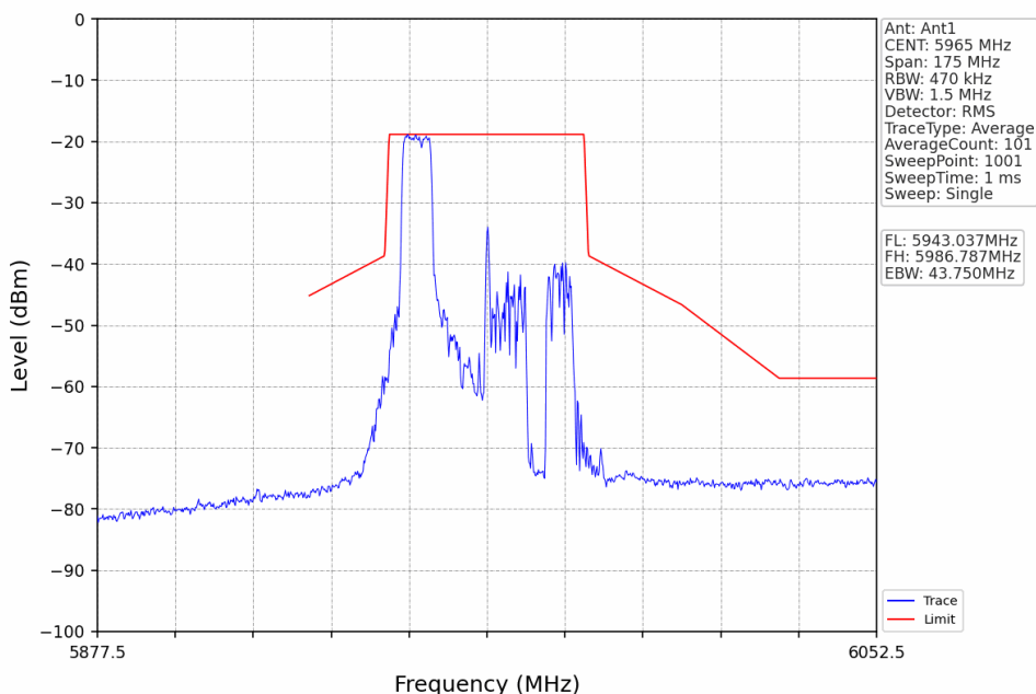
802.11ax(HEW40) LCH_5965MHz RU484 Left Ant1 NTNV
