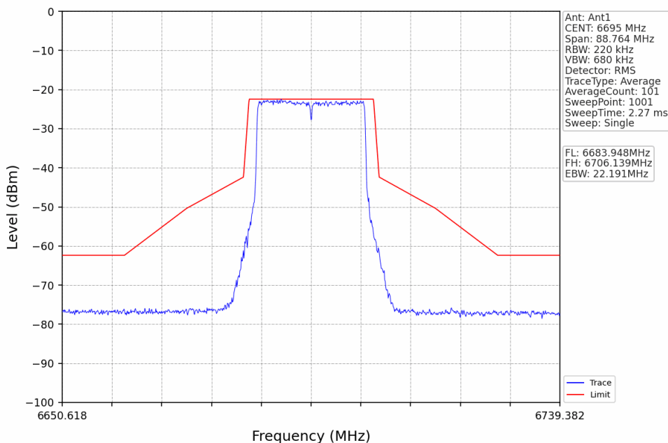
802.11ax(HEW20) MCH 6695MHz RU242 Left_Ant1_NTNV
