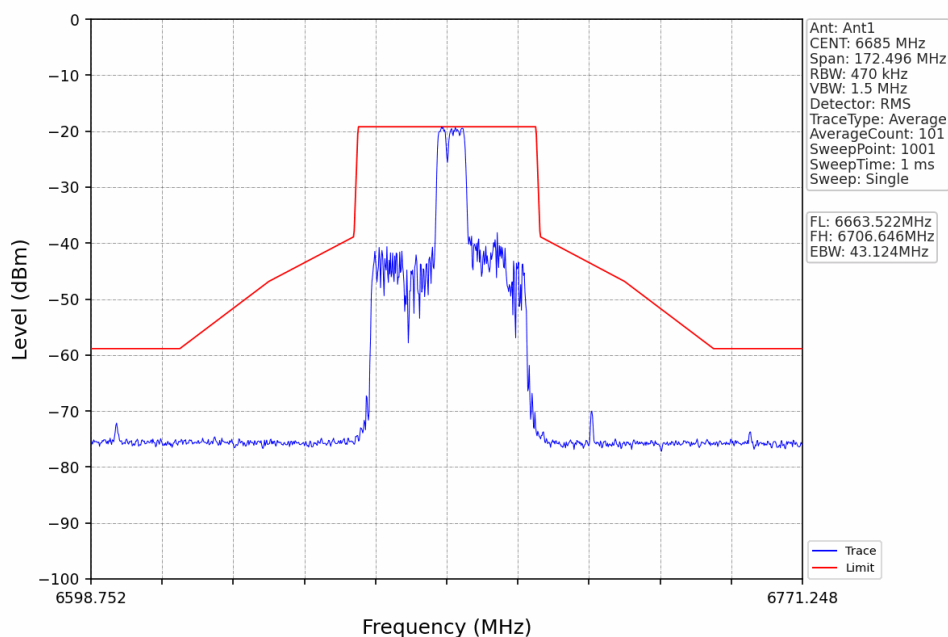
802.11ax(HEW40) MCH 6685MHz RU52+26 Mid Ant1 NTNV
