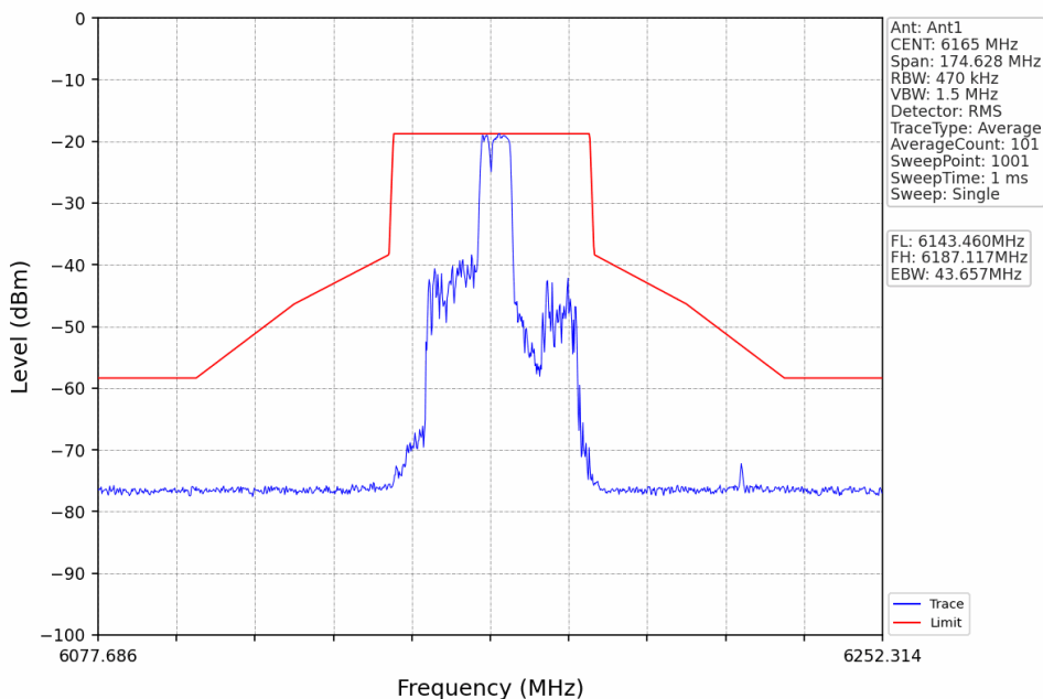
802.11ax(HEW40) MCH 6165MHz RU52+26 Mid Ant1 NTN
