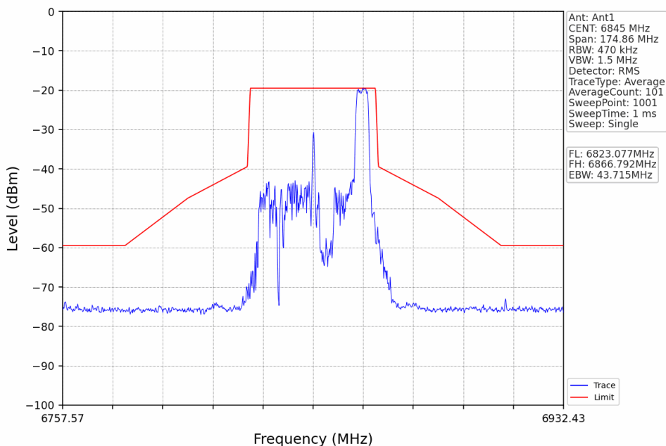
802.11ax(HEW40) HCH 6845MHz RU52 Right Ant1 NTN
