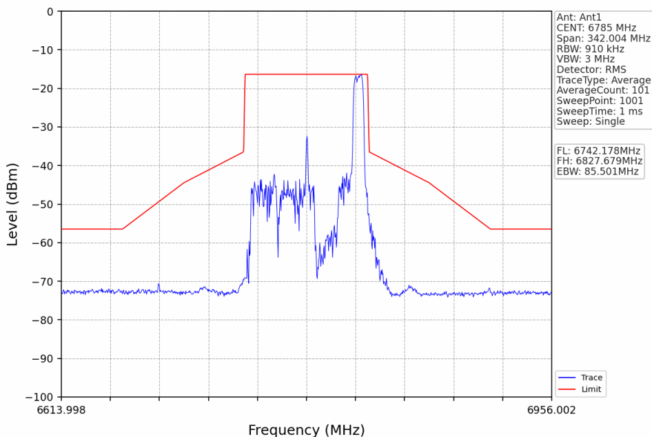
802.11ax(HEW80) HCH 6785MHz RU52+26 Right Ant1 NTN
