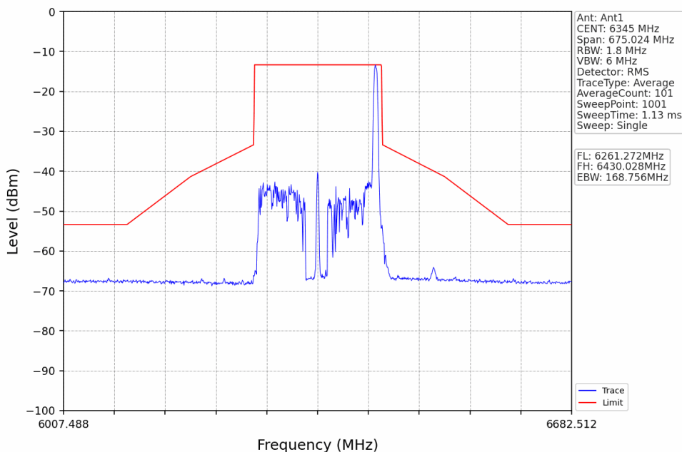
802.11ax(HEW160) HCH 6345MHz RU52 Right Ant1 NTVN
