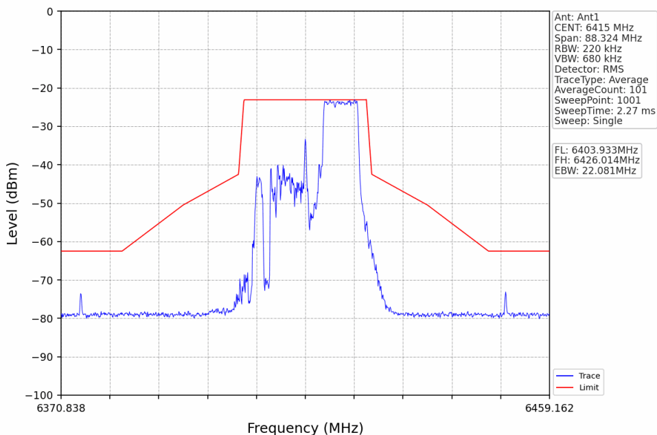
802.11ax(HEW20) HCH 6415MHz RU52+26 Right Ant1 NTN
