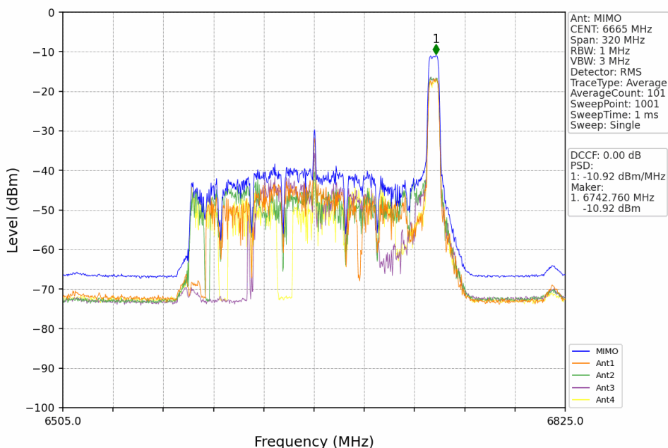
802.11ax(HEW160) MCH 6665MHz 2xRU996 Left MIMO NTN
