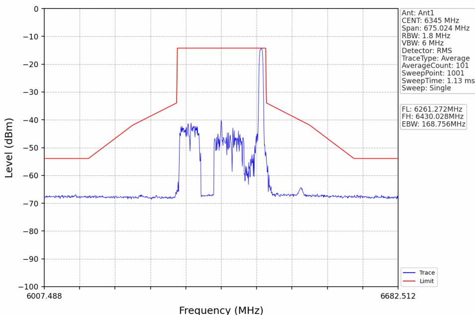
802.11ax(HEW160) HCH 6345MHz 2xRU996 Left Ant1 NTNV
