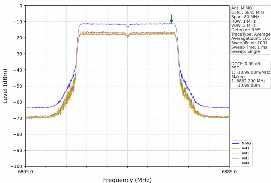
802.11ax(HEW40) HCH 6845MHz RU484 Left MIMO NTN
