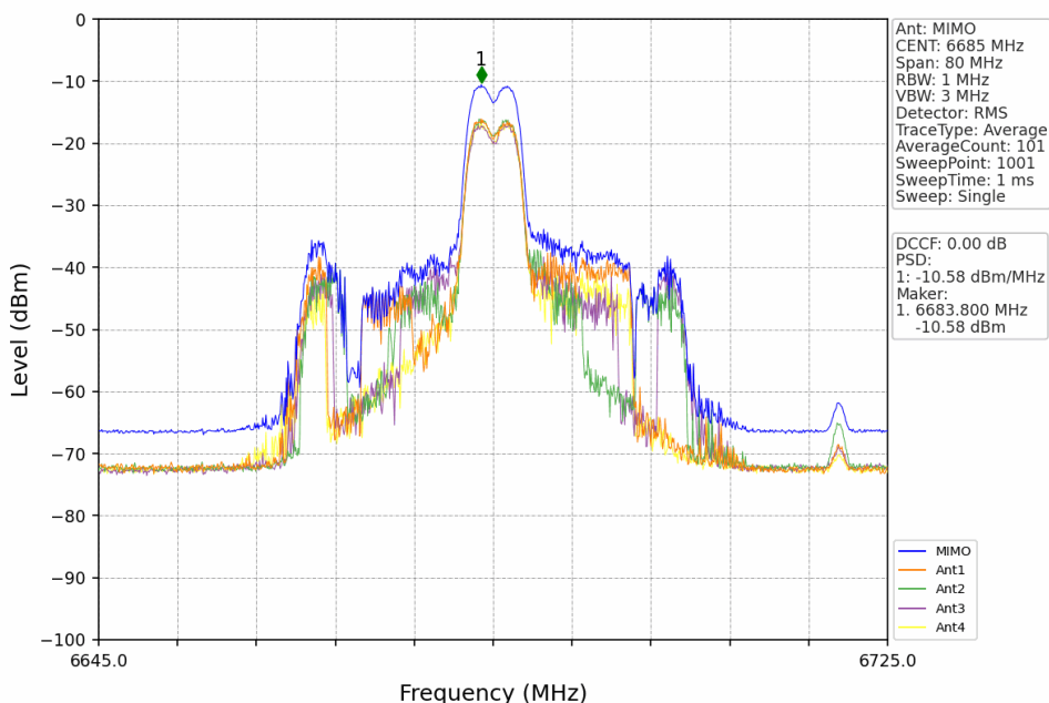
802.11ax(HEW40)_MCH_6685MHz_RU52+26_Mid_MIMO_NTNV
