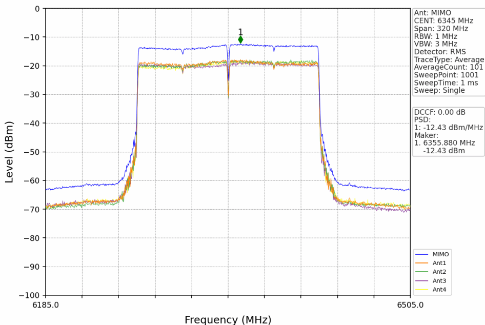
802.11ax(HEW160) HCH 6345MHz 2xRU996 Left MIMO NTN
