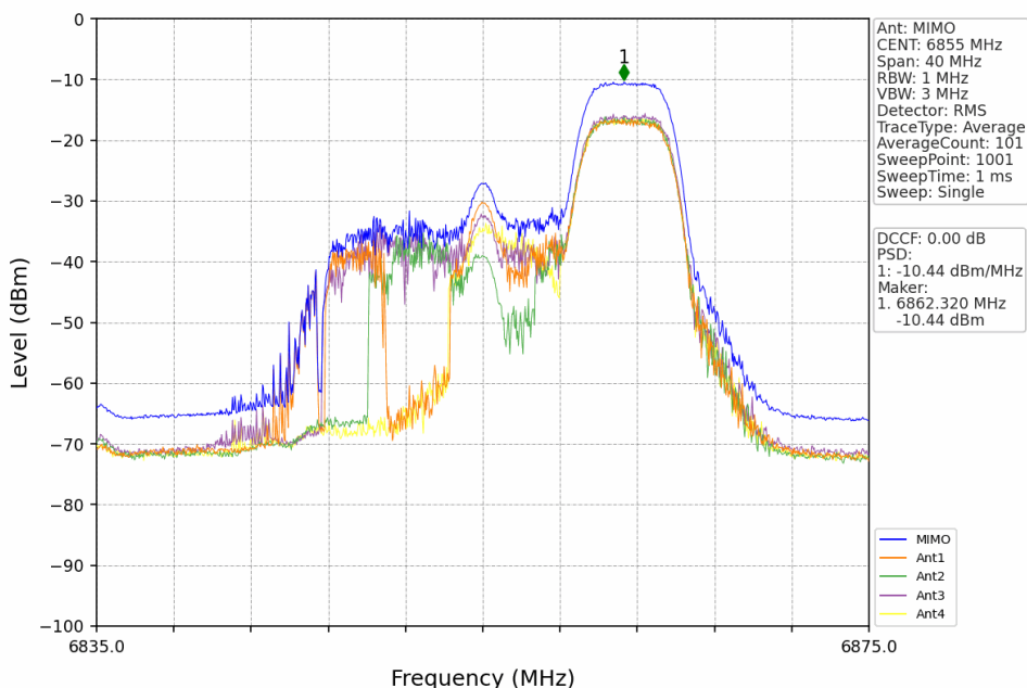
802.11ax(HEW20) HCH 6855MHz RU52+26 Right MIMO NTN
