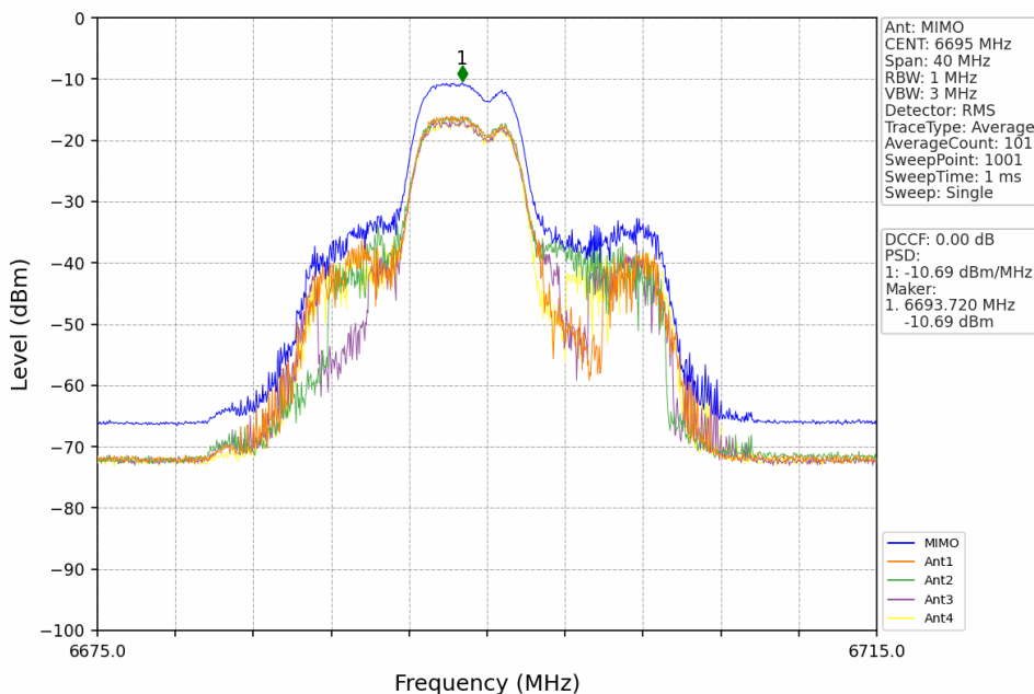
802.11ax(HEW20) MCH 6695MHz RU52 Mid MIMO NTN
