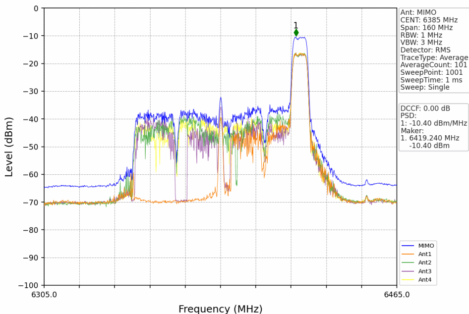
802.11ax(HEW80) HCH 6385MHz RU52+26 Right MIMO NTN
