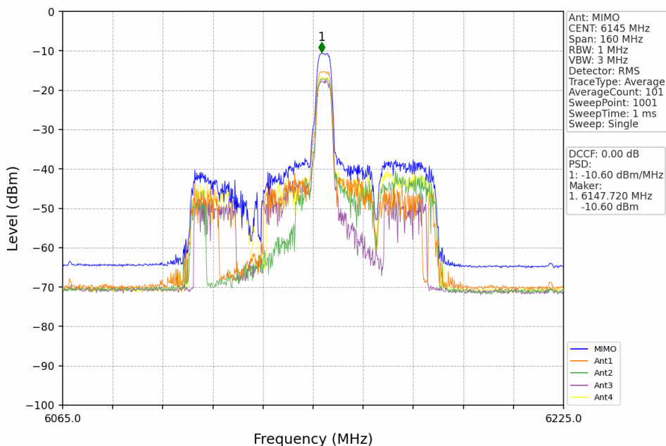
802.11ax(HEW80) MCH 6145MHz RU52 Mid MIMO NTN
