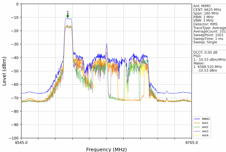
802.11ax(HEW80) LCH_6625MHz RU52+26 Left MIMO NTN
