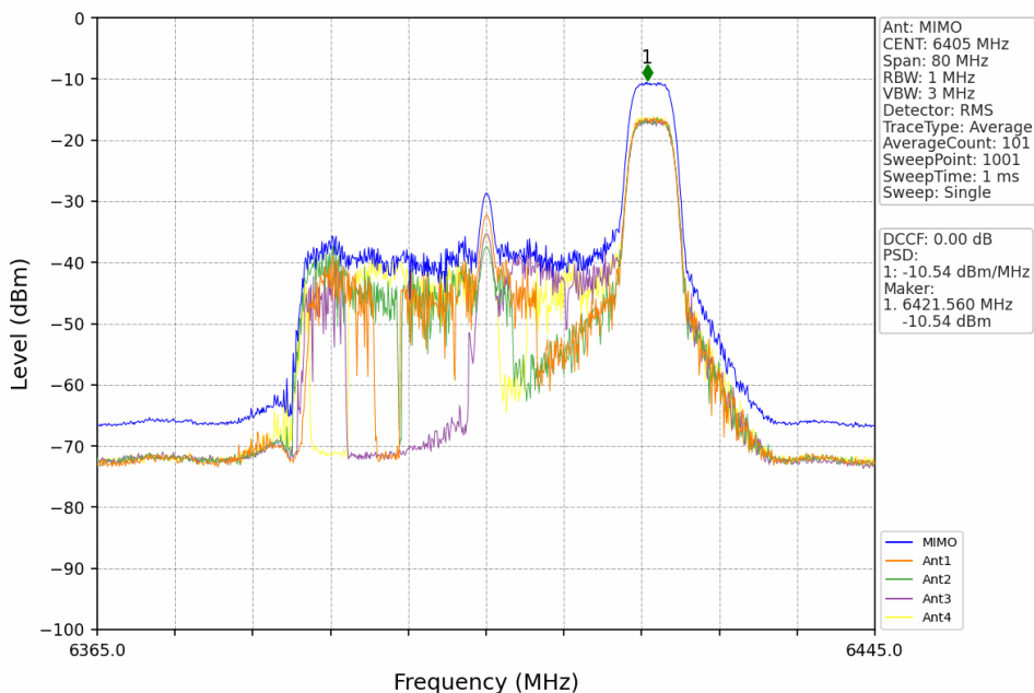
802.11ax(HEW40) HCH 6405MHz RU52 Right MIMO NTN
