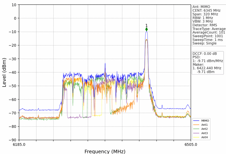
802.11be(EHT160)_HCH_6345MHz_RU52_Right_MIMO_NTNV
