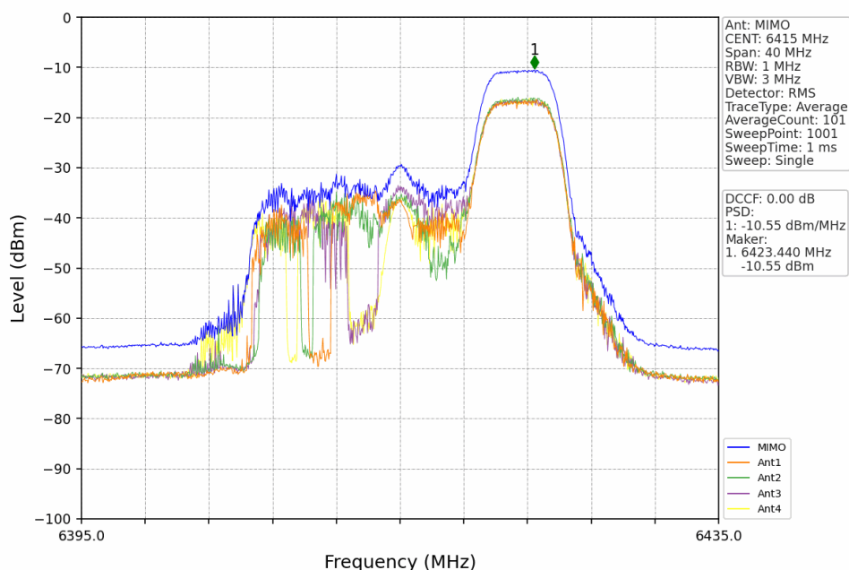
802.11be(EHT20)_HCH_6415MHz_RU52+26_Right_MIMO_NTNV
