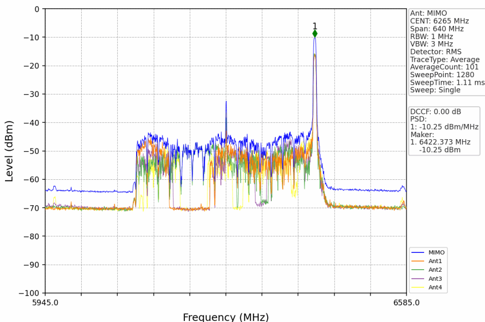
802.11be(EHT320)_HCH_6265MHz_RU52+26_Right_MIMO_NTNV
