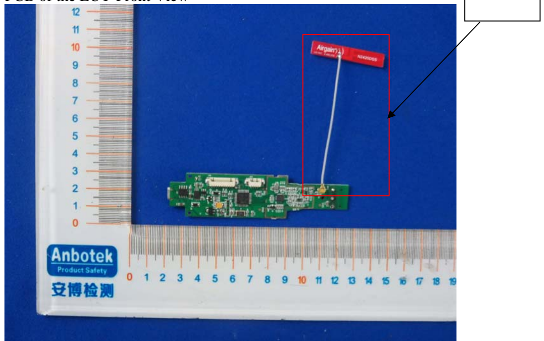
Figure 12 PCB of the EUT-Front View
