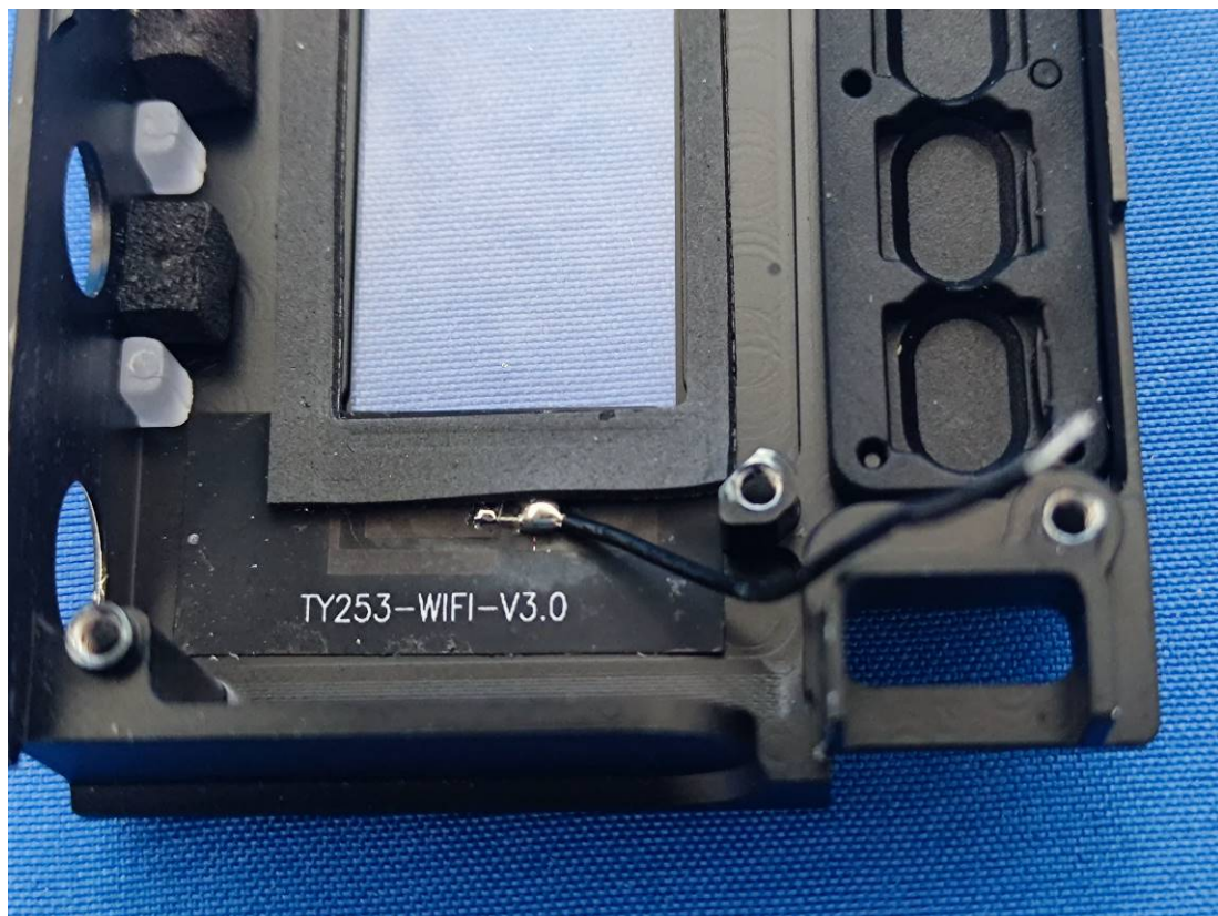
2.4G SRD Antenna
