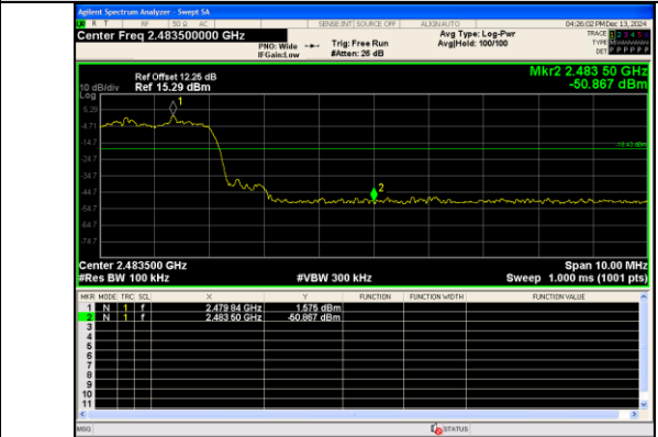
Out Of Band Emission(Right) \pi/4 DQPSK_2-DH5_Channel Hopping
