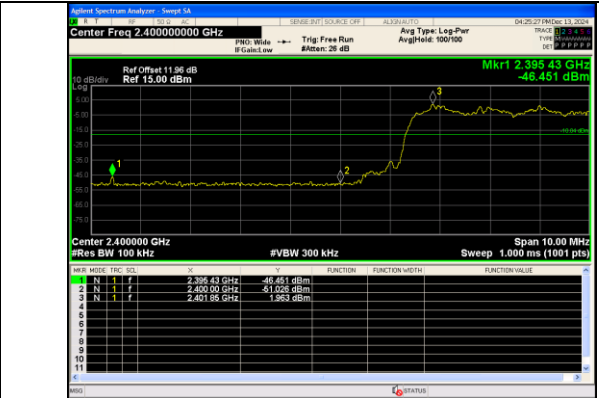
Out Of Band Emission(Left) \pi/4 DQPSK_2-DH5_Channel Hopping
