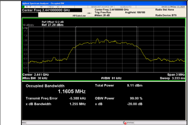
8DPSK 3-DH5 Channel 39
