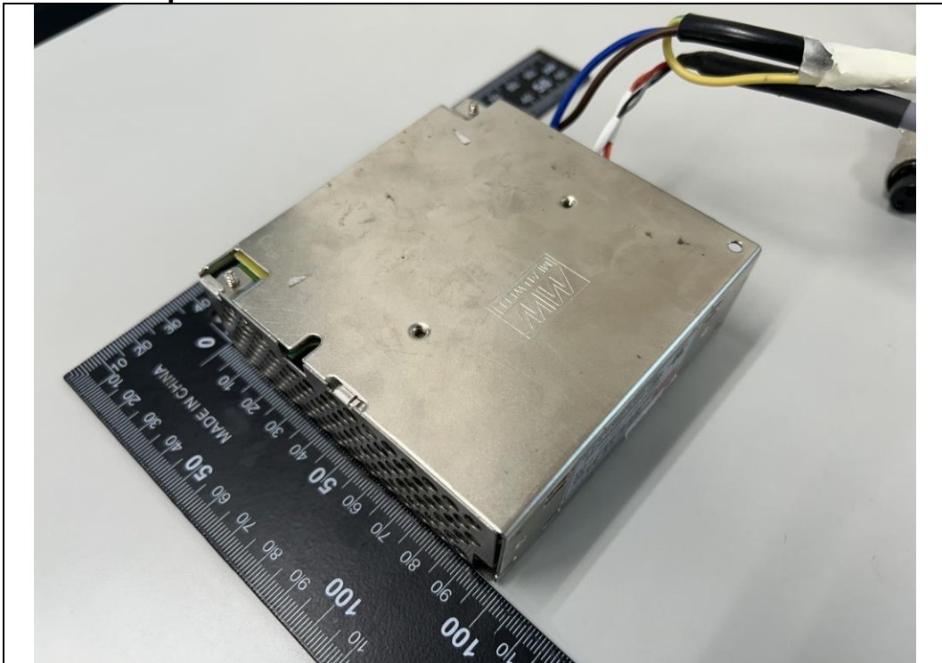
AC/DC Adapter Rear
