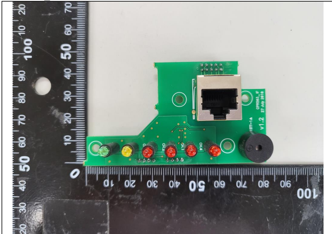
CPR503_IF Front
