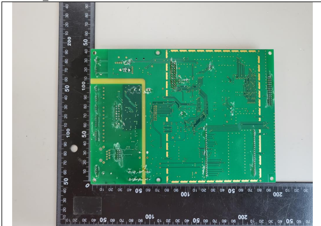
CPR503 Main.brd Rear
