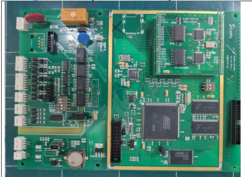
CPR503 Main.brd Front(Removed Shield-can)
