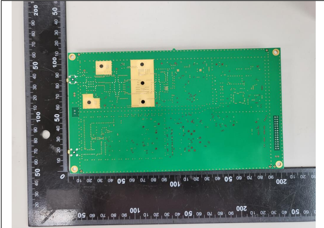
CPR503.RFB Rear
