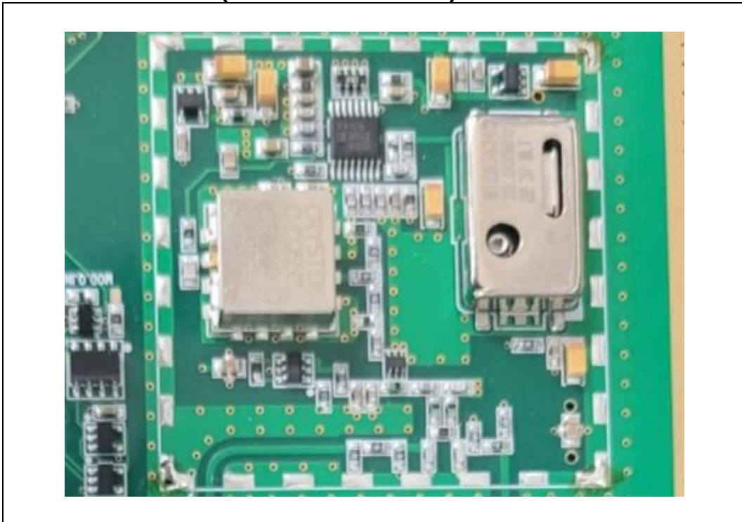
CPR503.RFB Front (Removed Shield-can)
