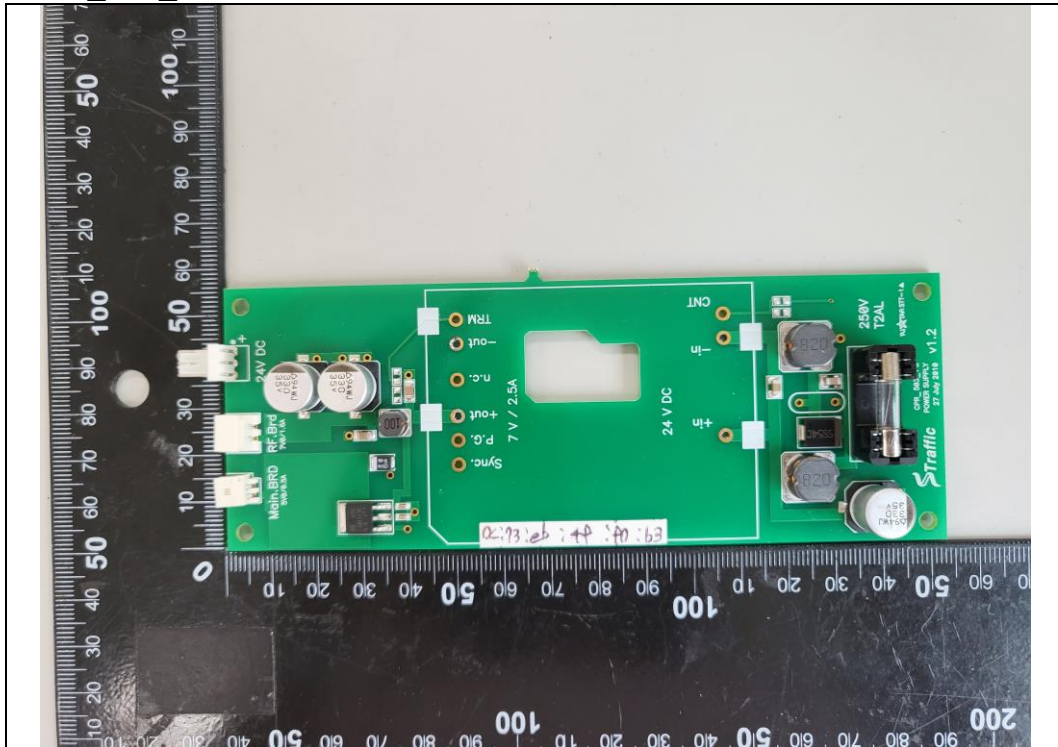
CPR_503 PS Front
