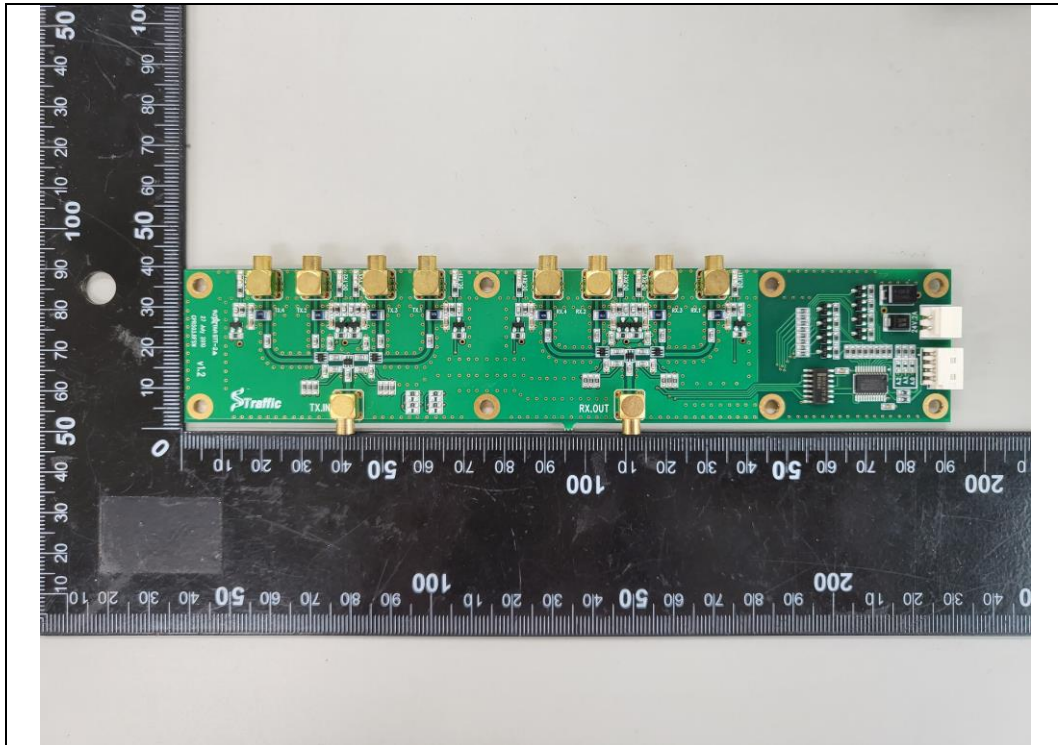
CPR503.RFSW Front
