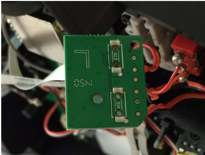
PCB 5 view side 2
