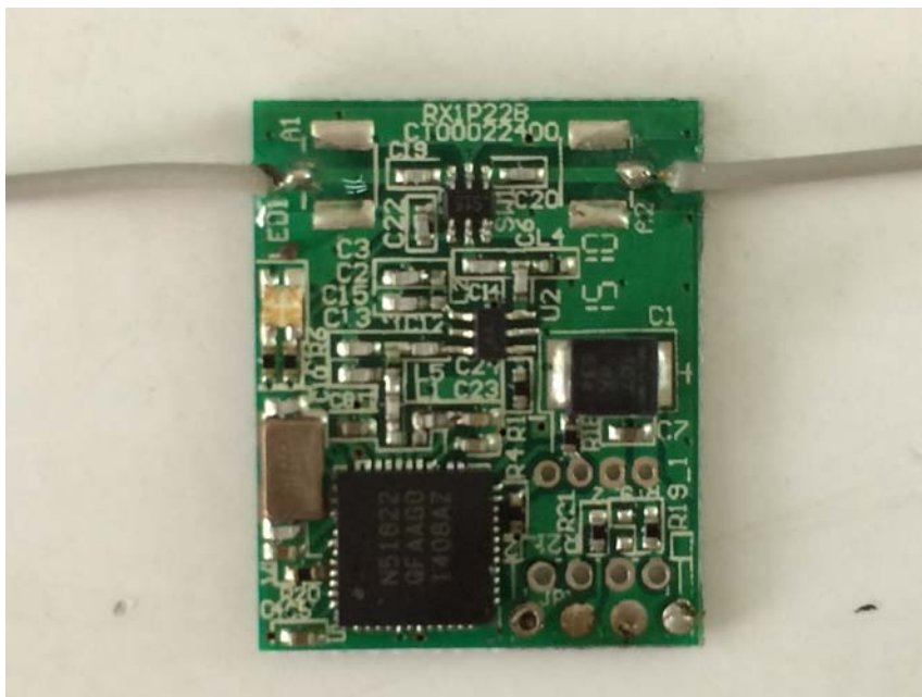
RX Module side 3 view
