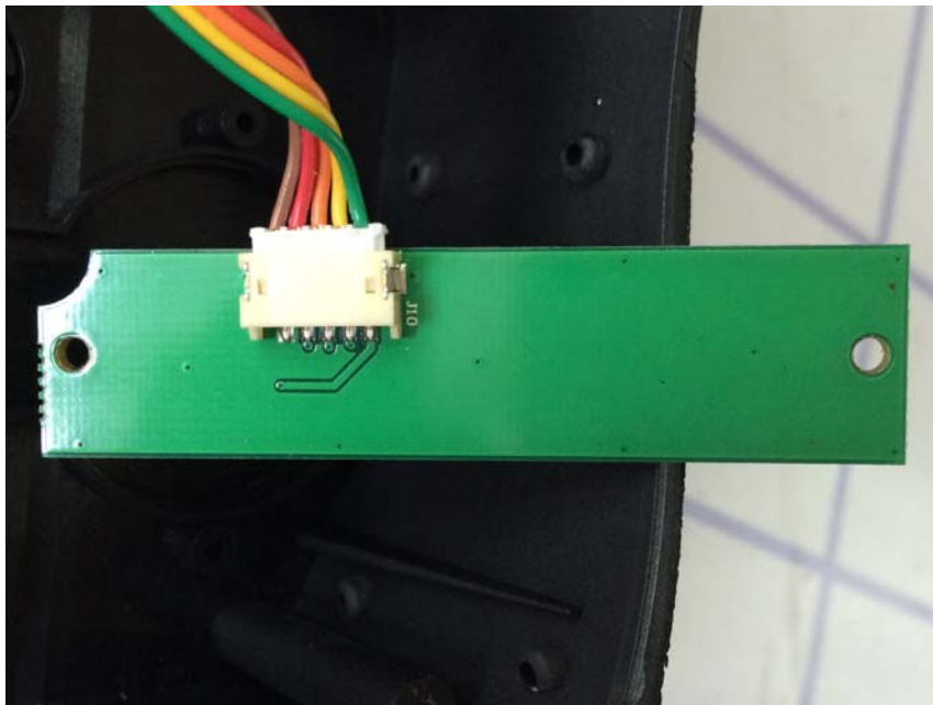
PCB 3 view side 1
