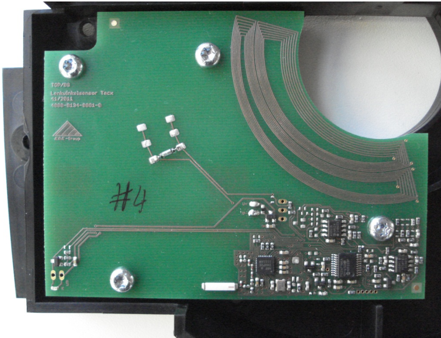
Photograph A3-1: Internal view – Transceiver board
