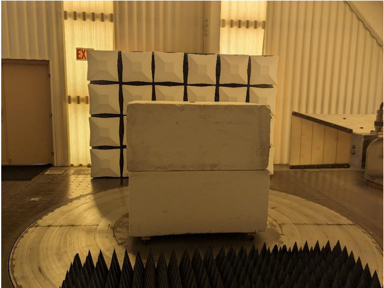
Photograph 3: Front View Radiated Emissions above 1GHz Worst Case Configuration (Laying Flat)
