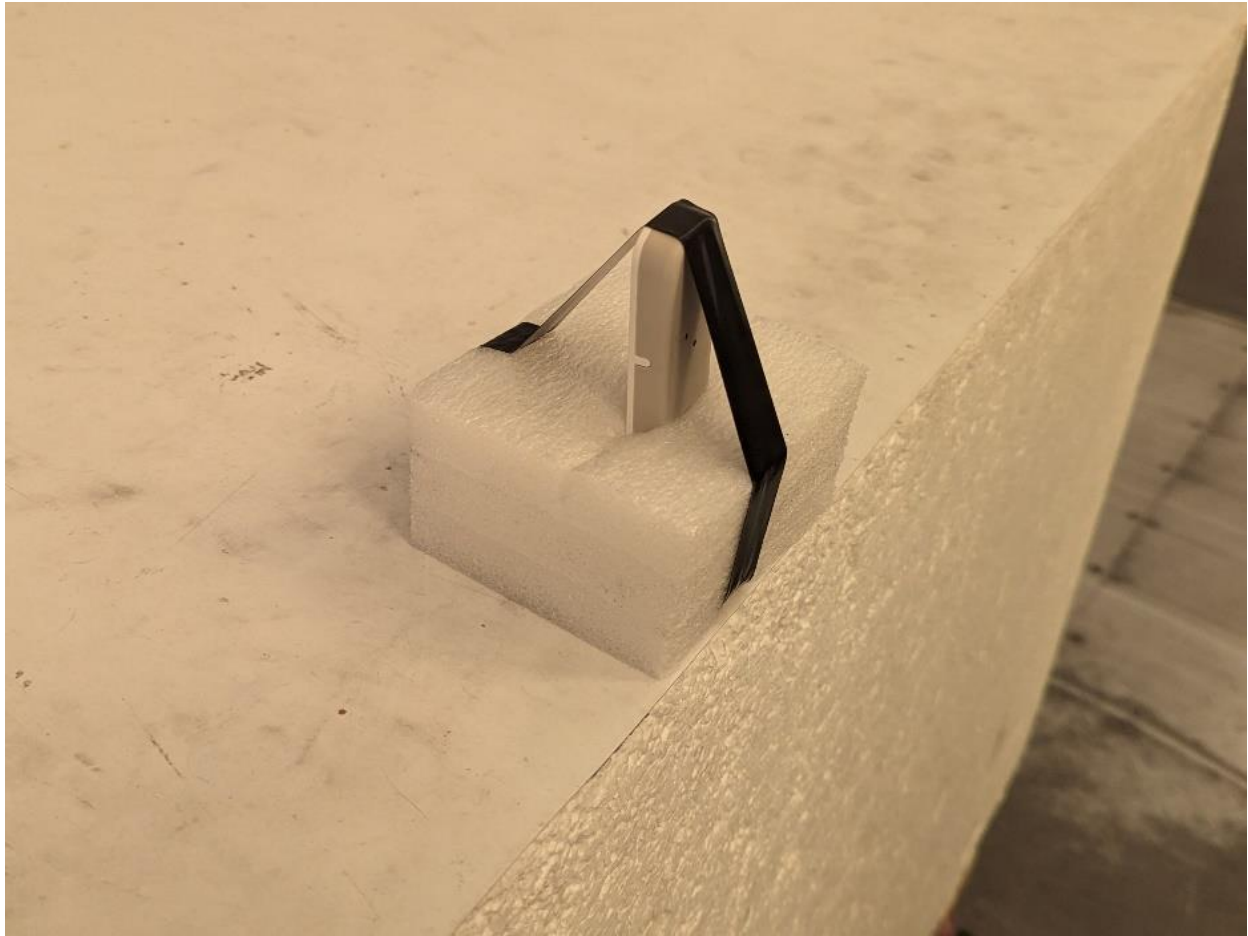
Photograph 5: View of Standing Short Edge Configuration
