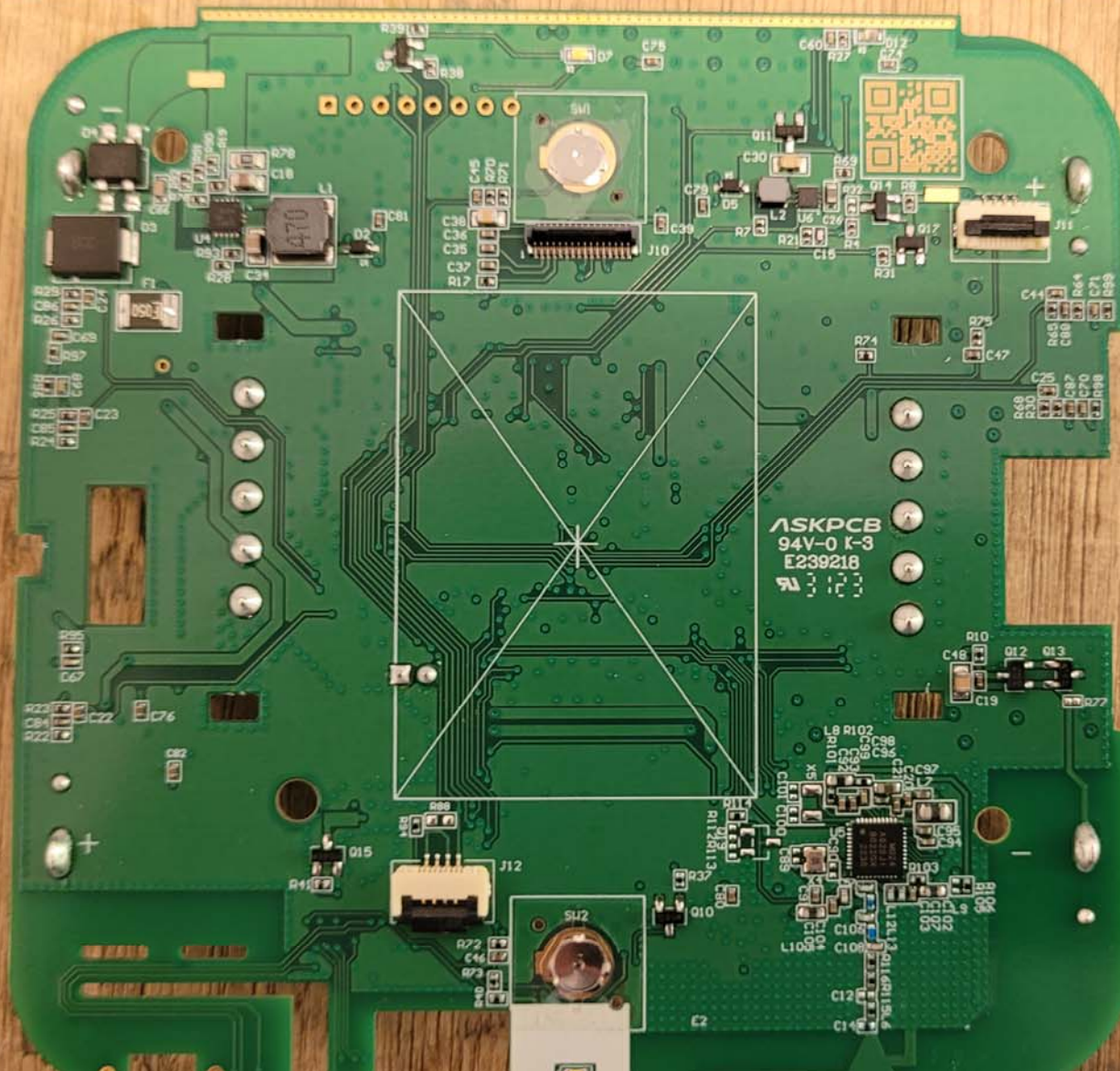
Top View of the PCB - View #2
