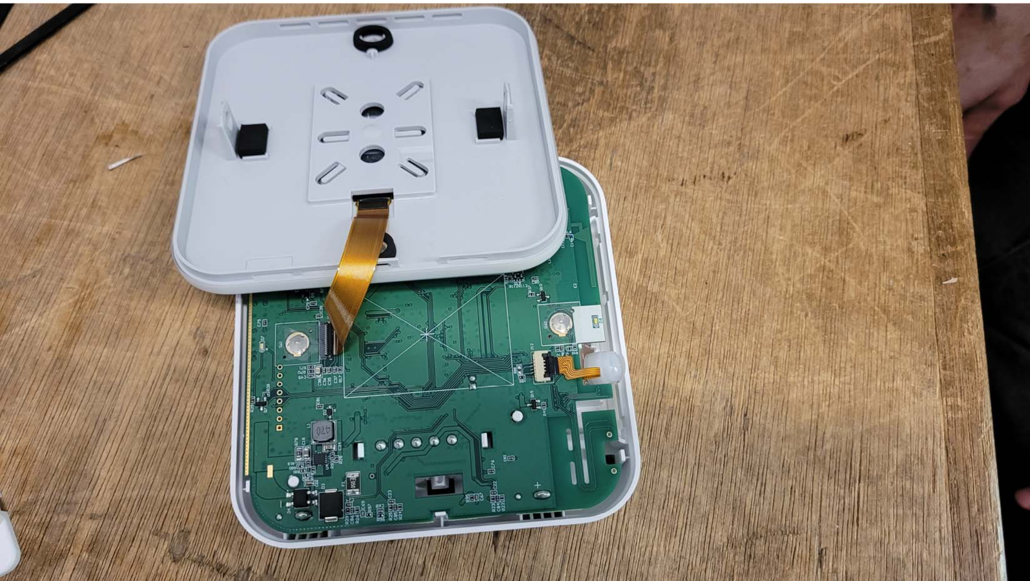
Inside View of the EUT #6
