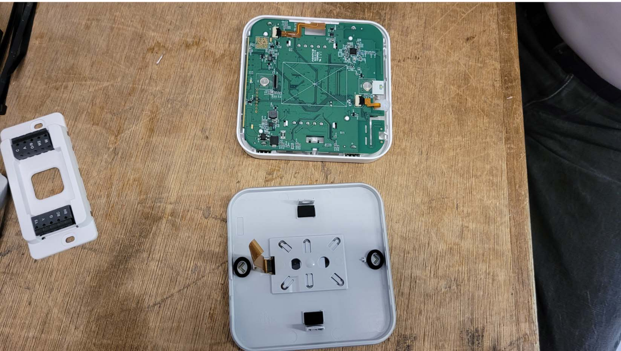
Inside View of the EUT #8
