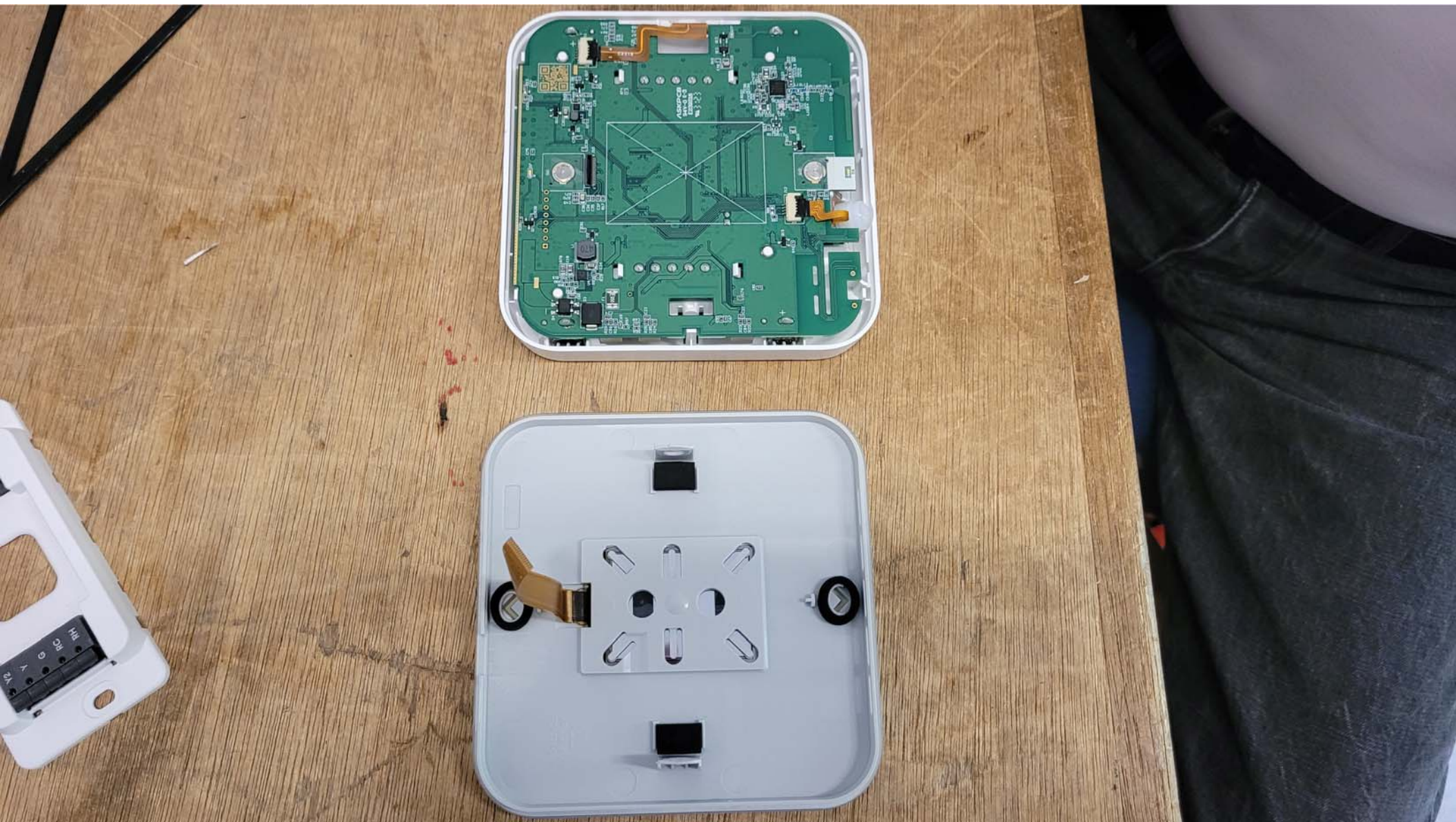
Inside View of the EUT #7
