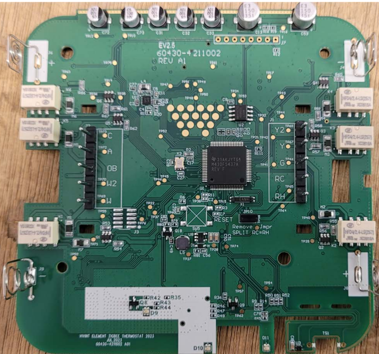
Bottom View of the PCB - View #2
