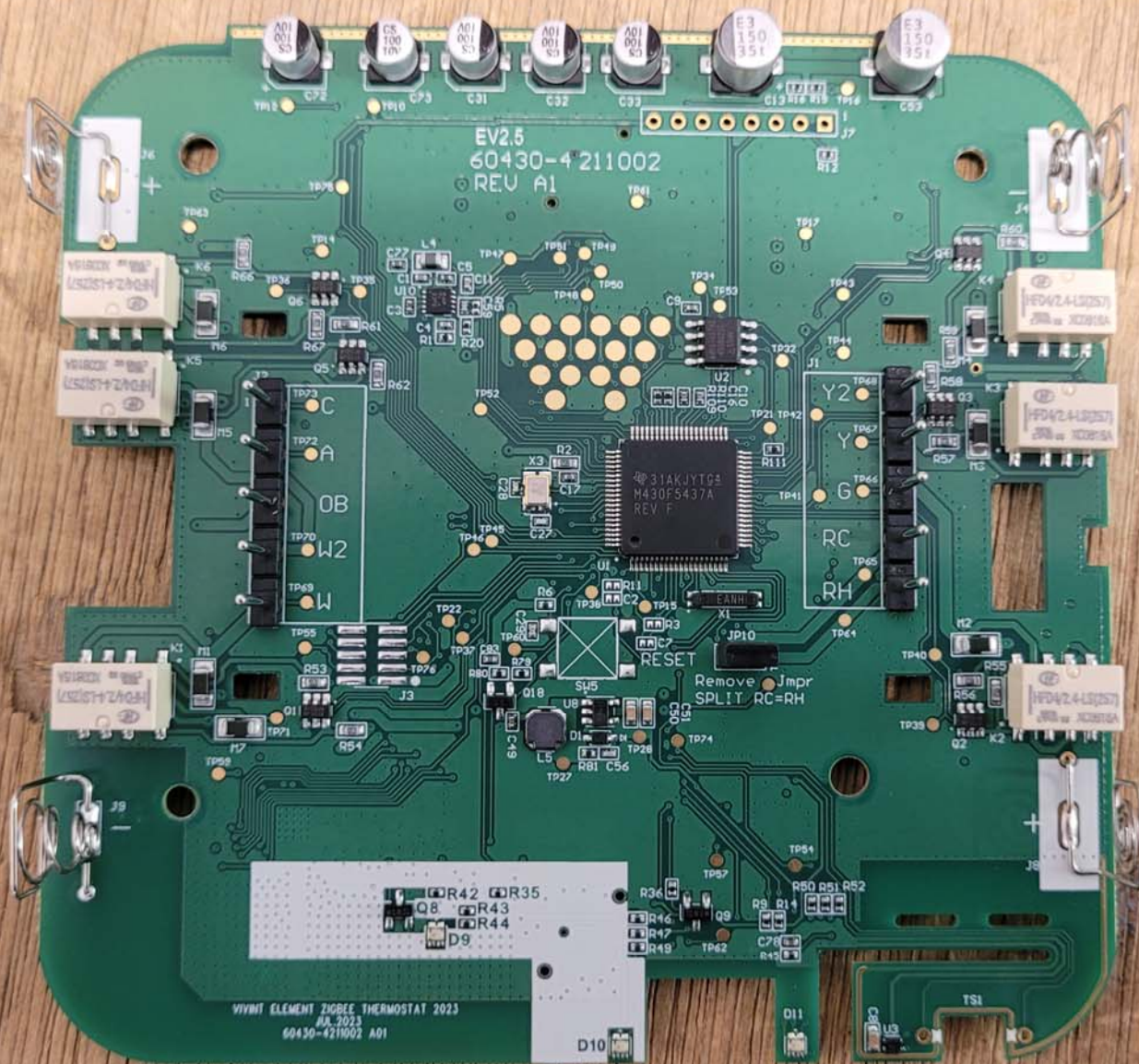
Bottom View of the PCB - View #1
