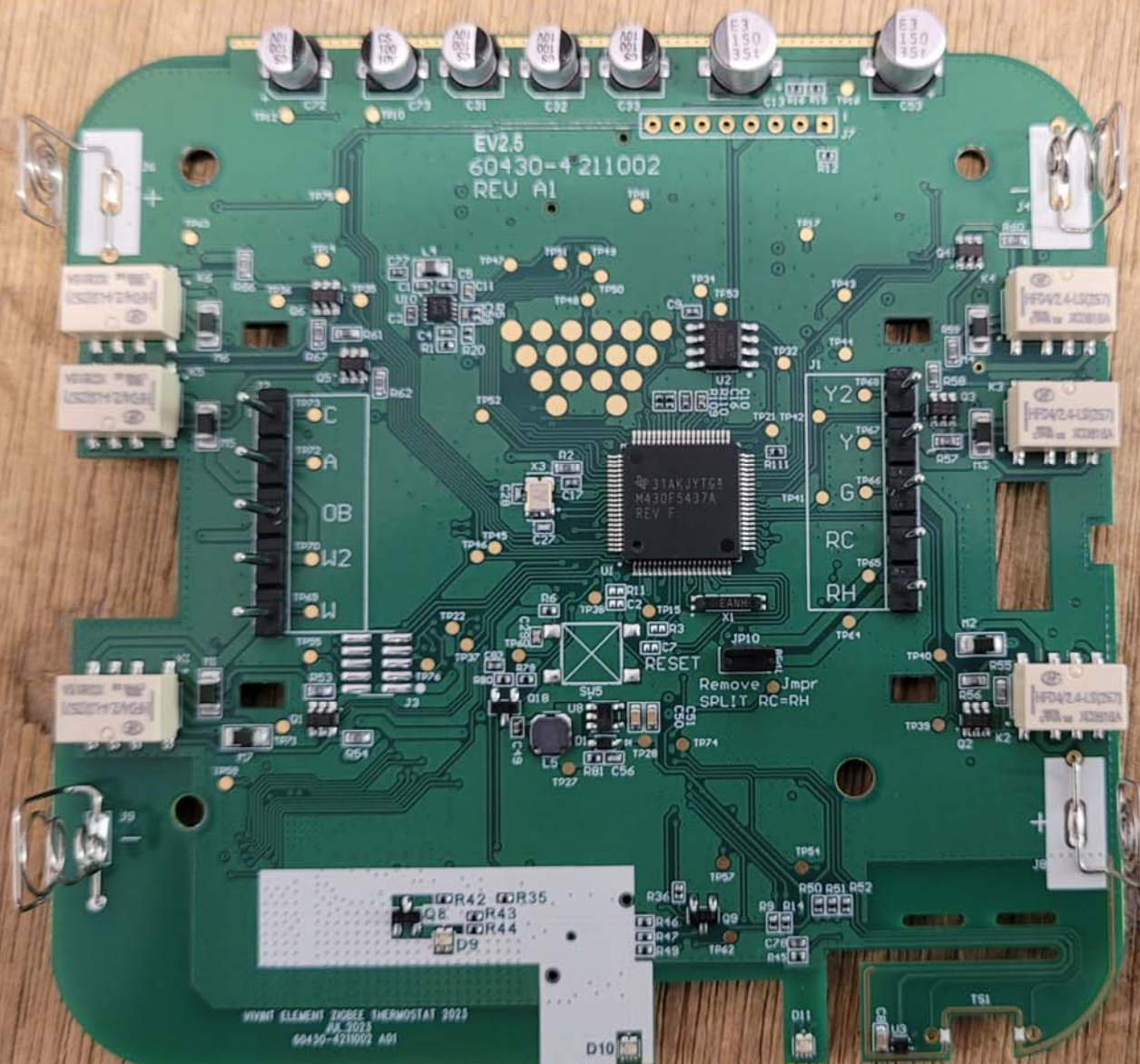
Bottom View of the PCB - View #3
