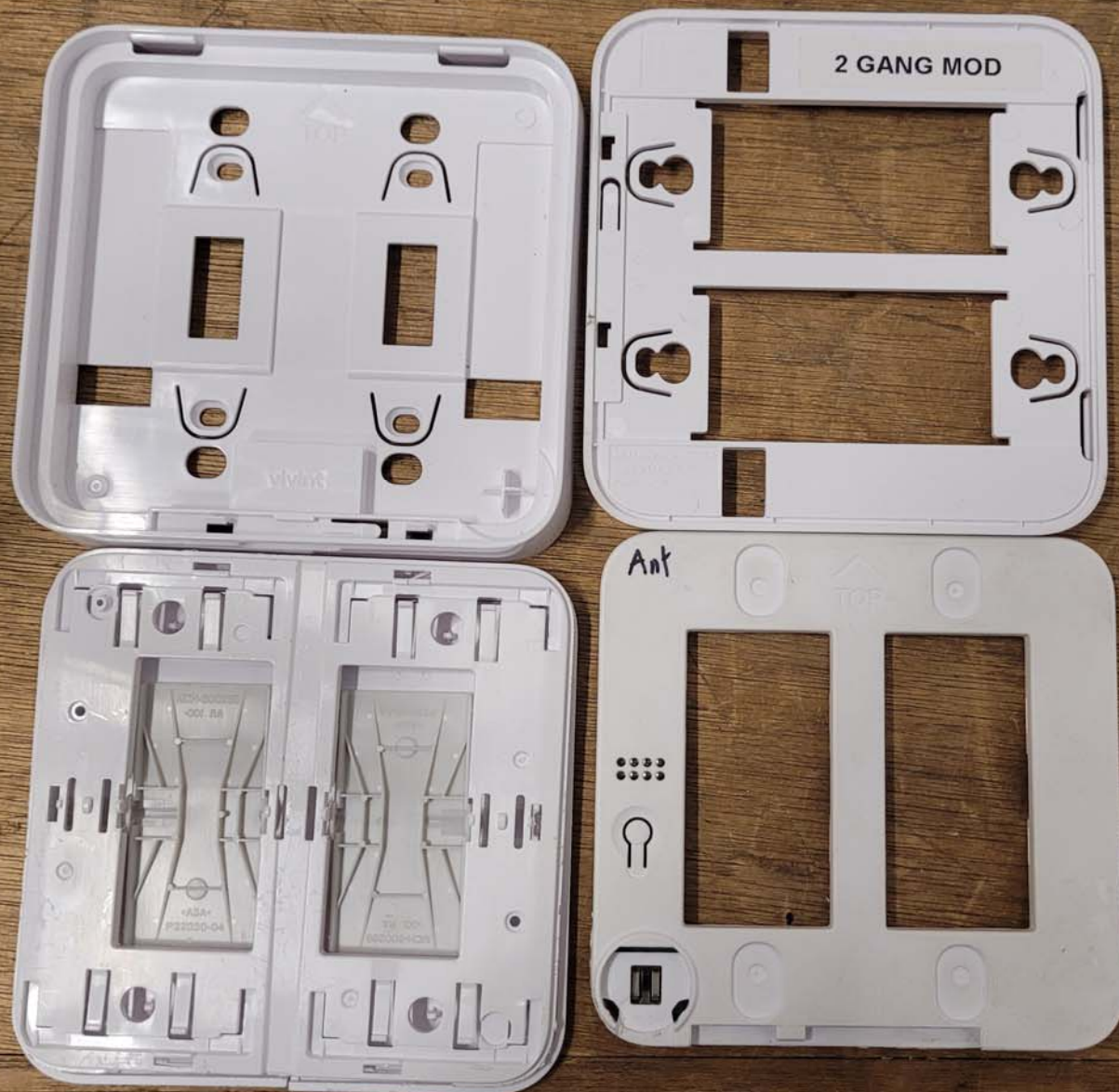
Photo (Bottom Right) showing the external side of the unit where the label will be placed.
