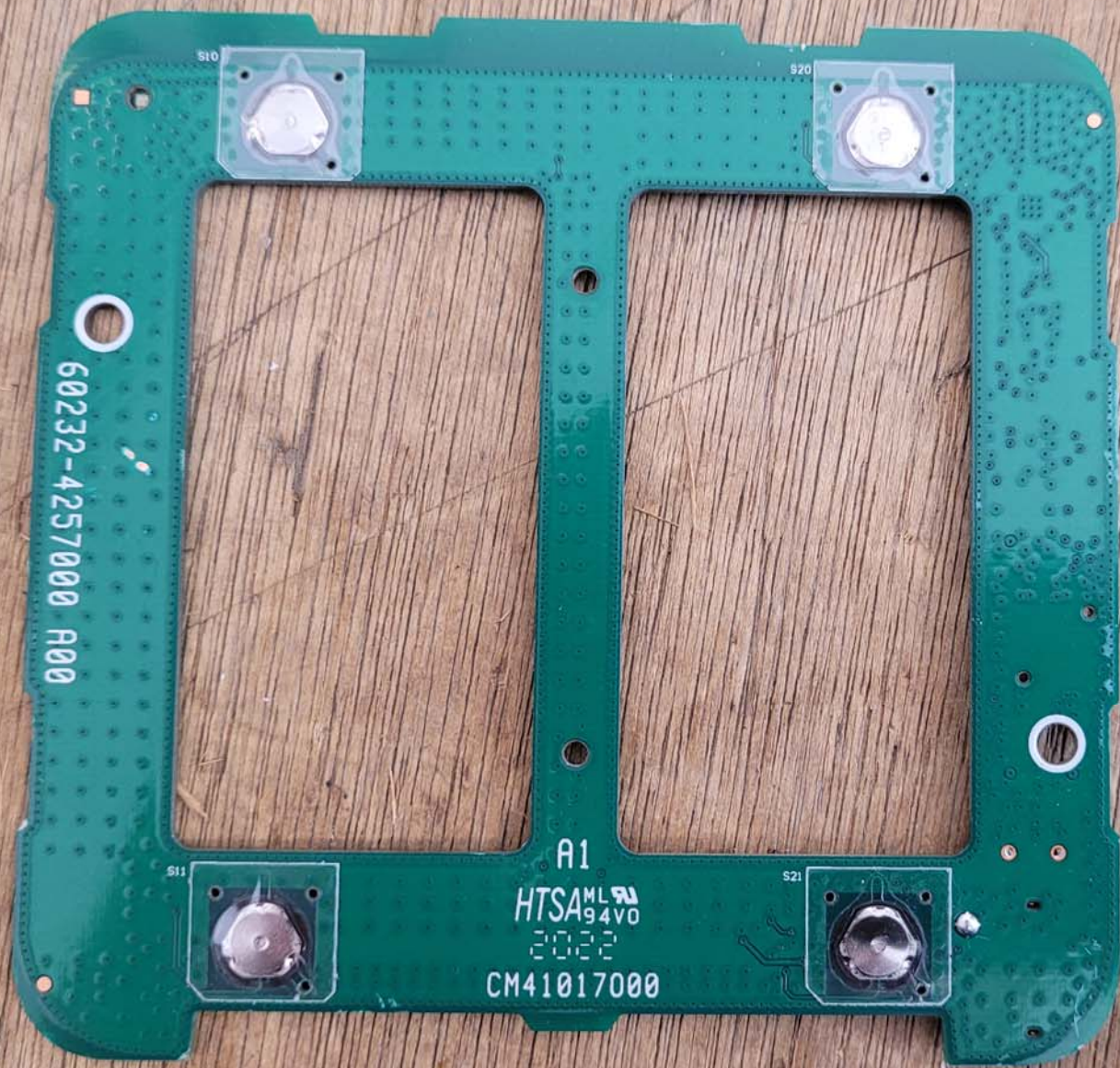
Bottom View of the PCB
