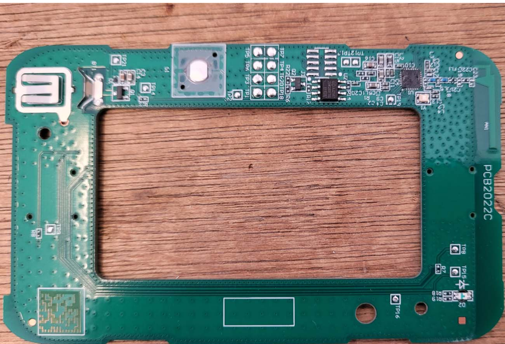
Top View of the PCB
