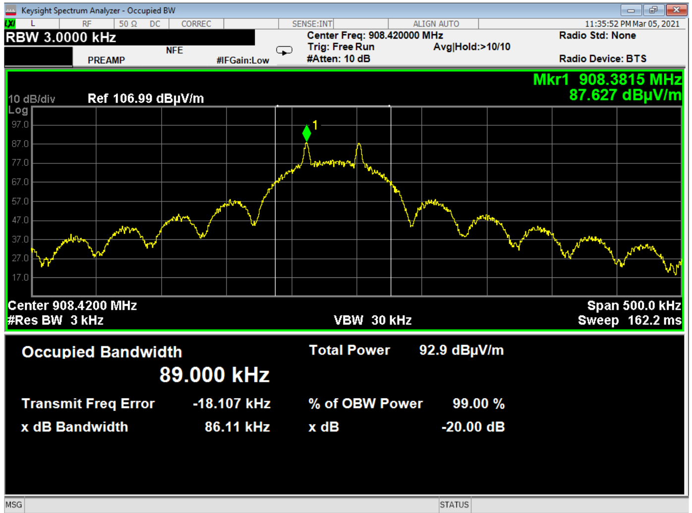
99 Percent Bandwidth Plot – 908.42 MHz
