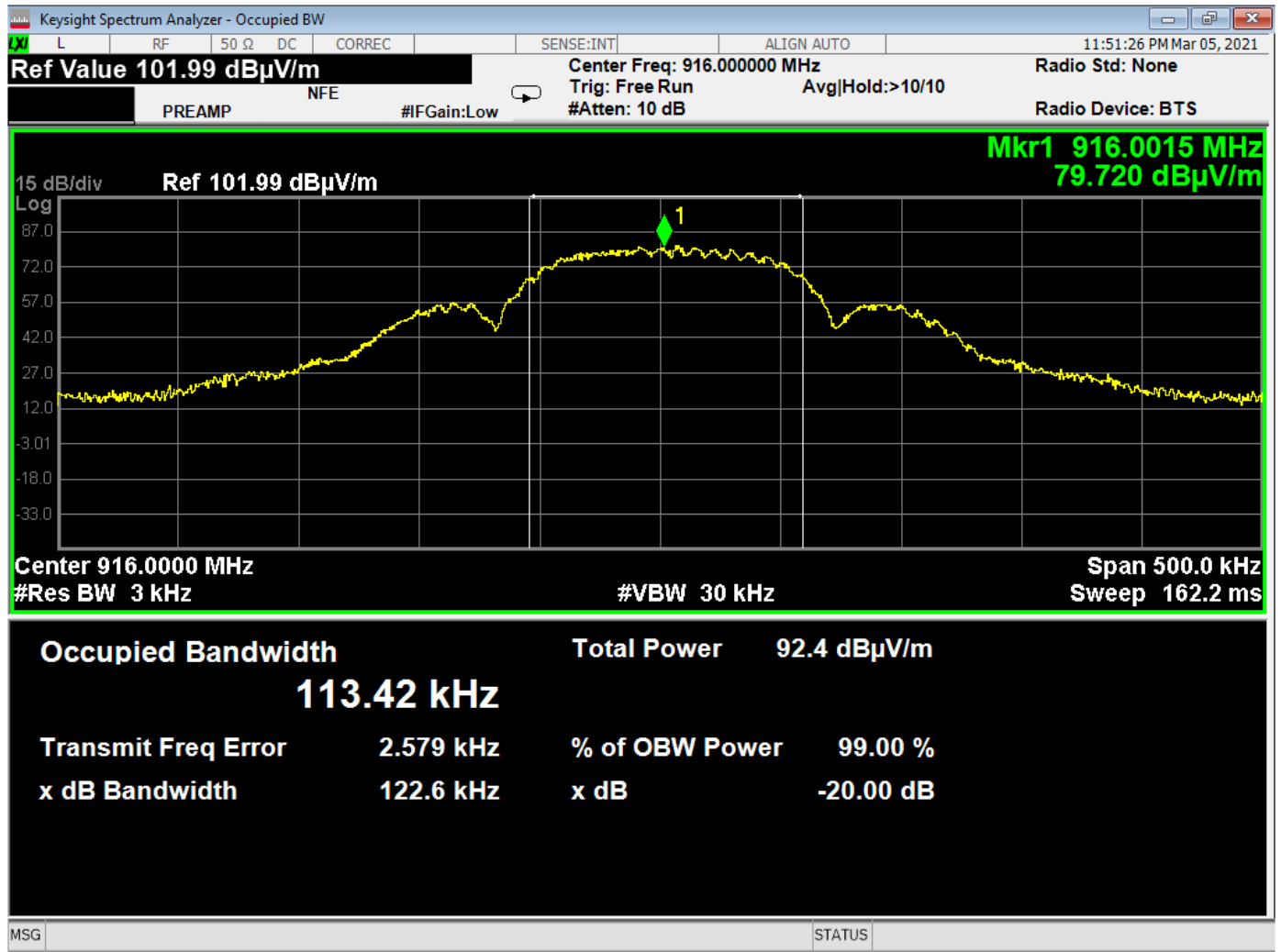
99 Percent Bandwidth Plot – 916.00 MHz
