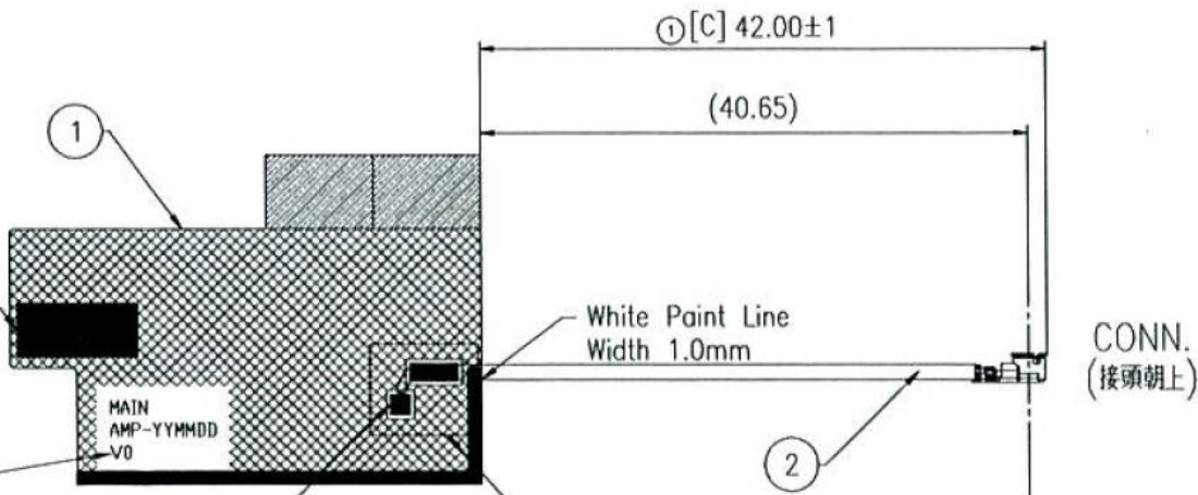
Main Antenna Dimensioned Drawing:
