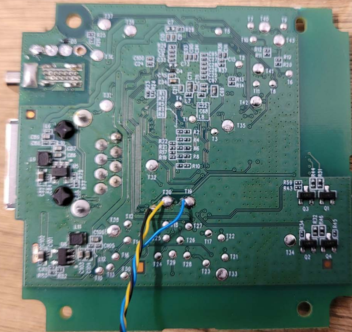
Top View of the PCB - View #2
