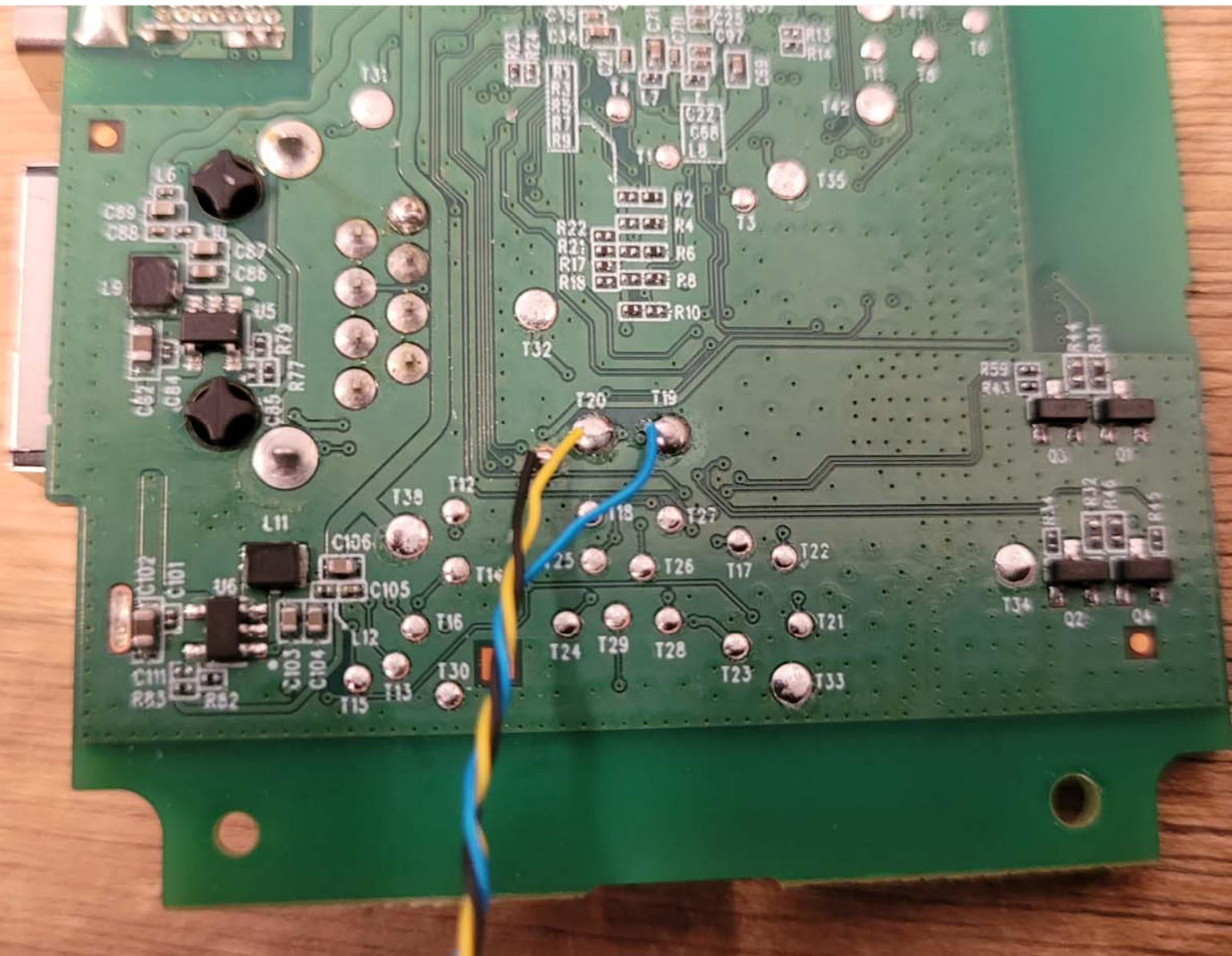
Top View of the PCB - Closeup #2
