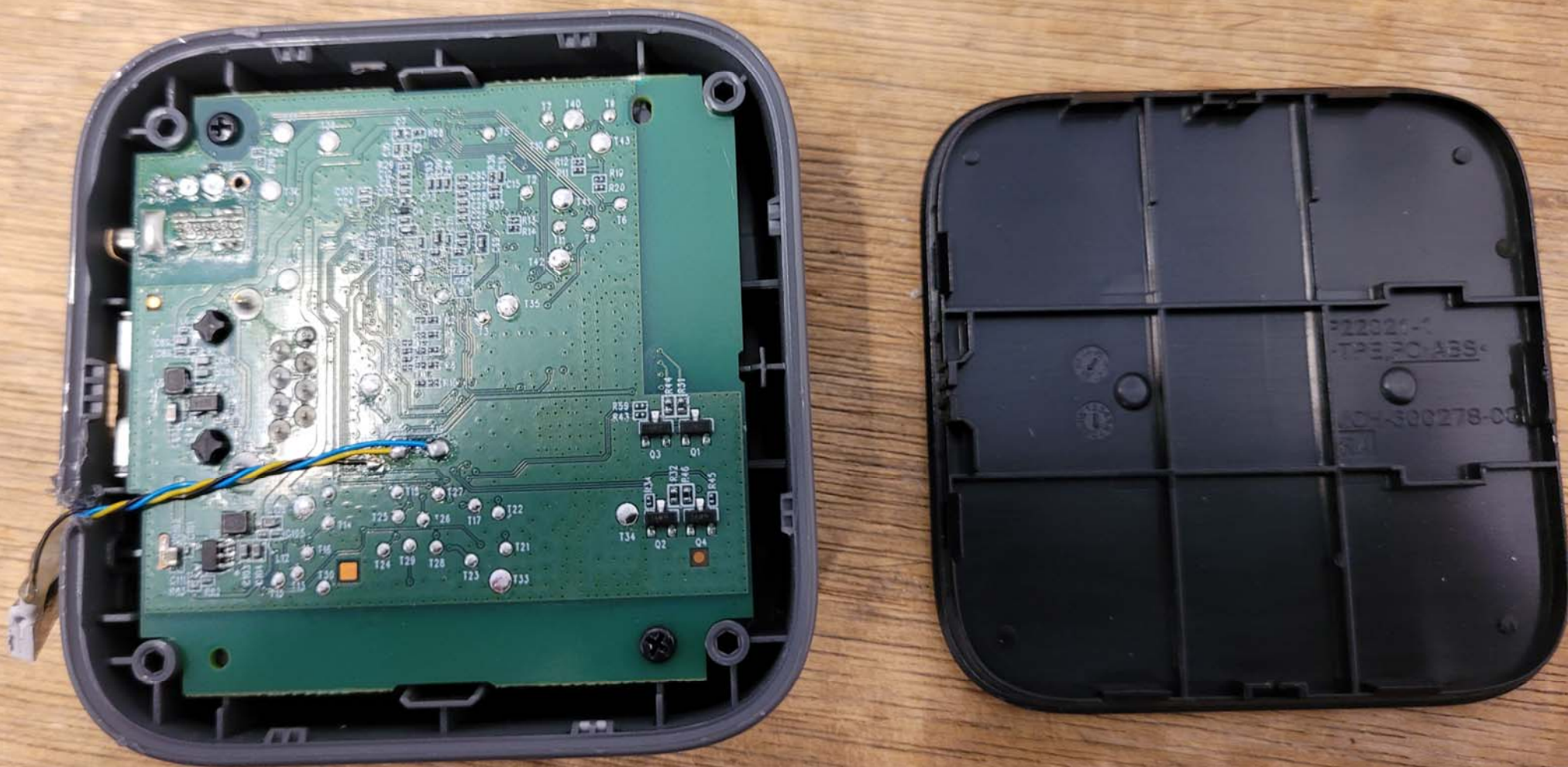
Inside View of the EUT #1
