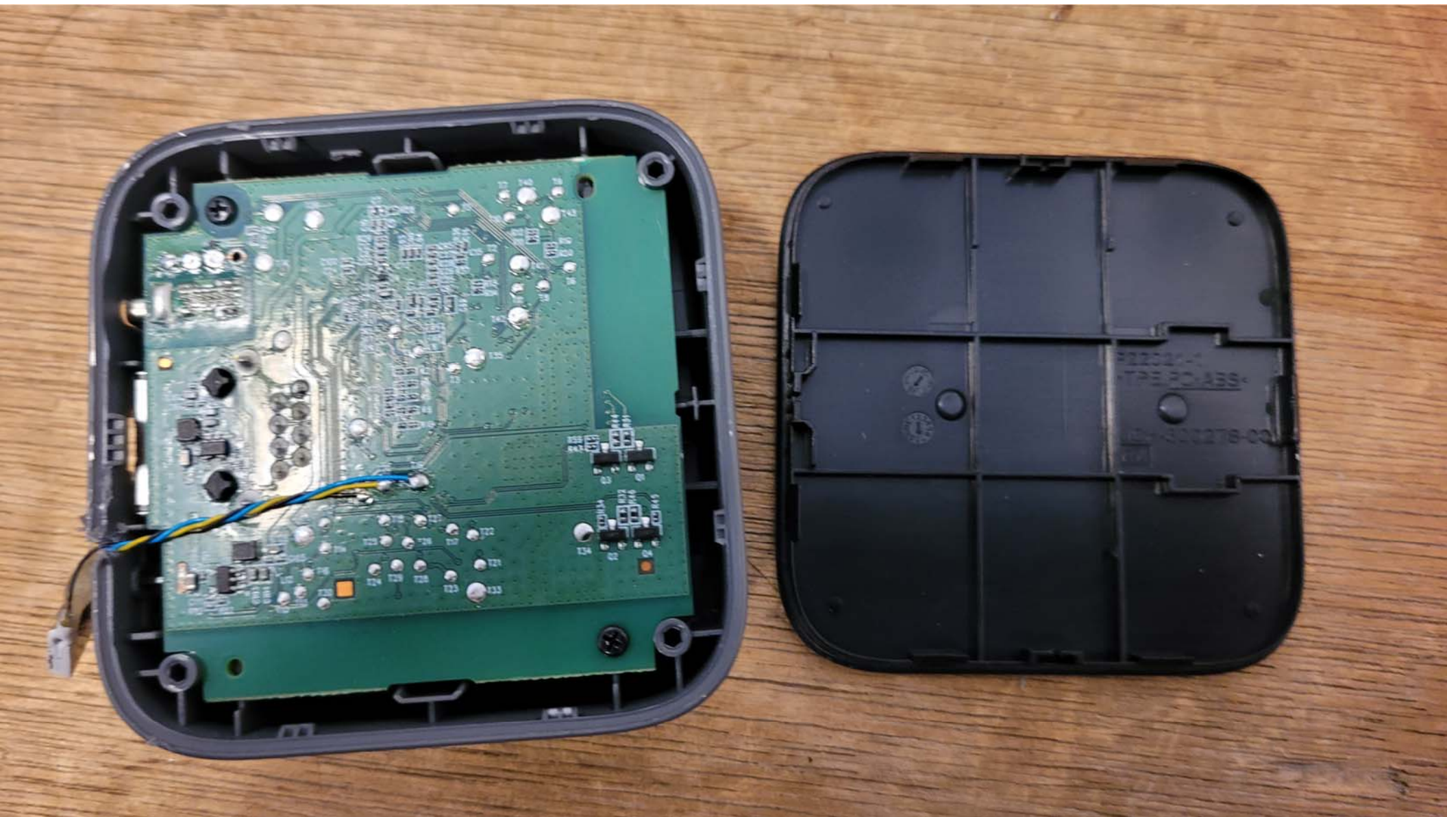
Inside View of the EUT #2
