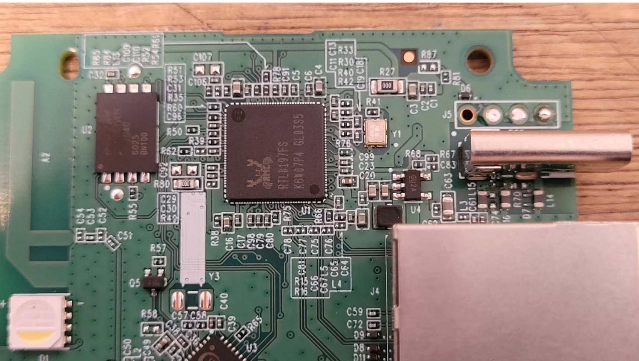
Bottom View of the PCB - Closeup #8
