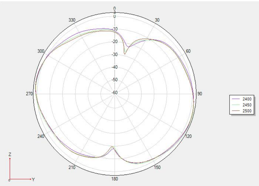
Phi 90 2D
