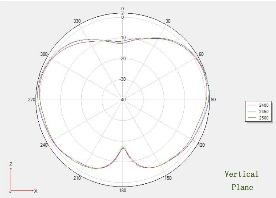
Phi 0 2D
