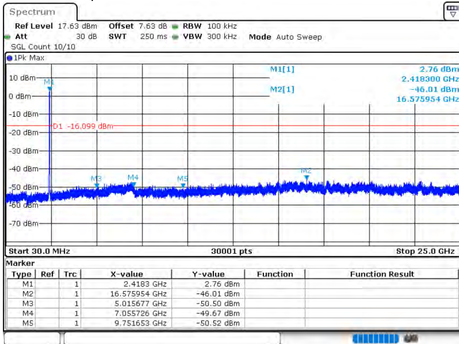
Tx. Spurious NVNT 802.11ax20 2412MHz Ant 2 Emission
