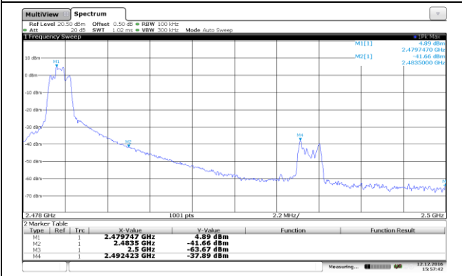
Bandedge- no hopping mode (CH78)
