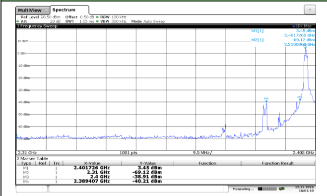
Bandedge- no hopping mode (CH00)
