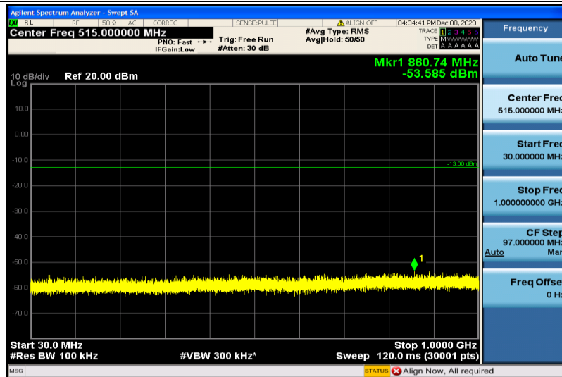
Band66-5MHz-16QAM-131997-1RB#0-30~1000MHz
