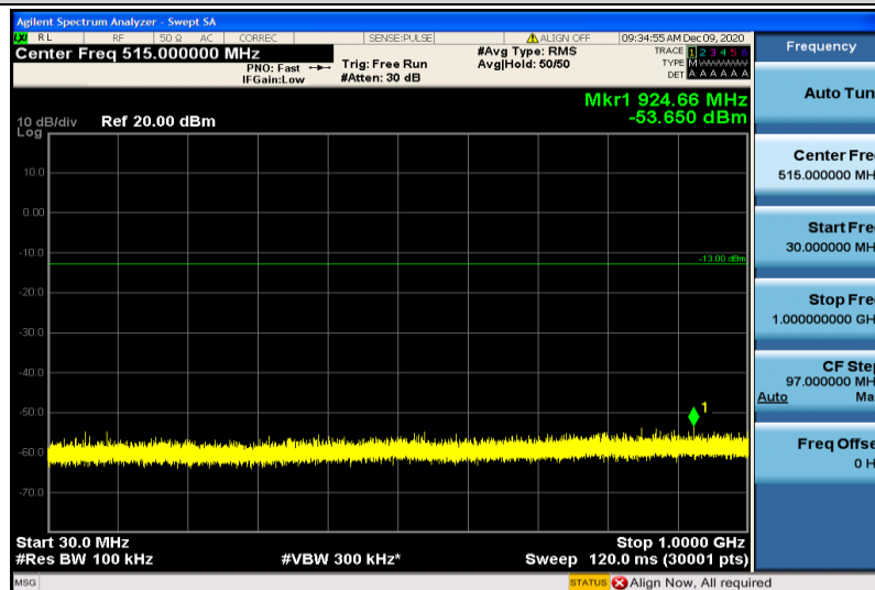
Band66-20MHz-16QAM-132572-1RB#0-30~1000MHz
