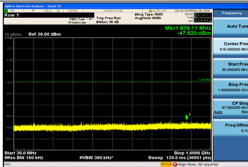
Band2-5MHz-16QAM-19175-1RB#0-30~1000MHz
