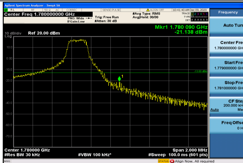
Band66-3MHz-16QAM-132657-1RB#14
