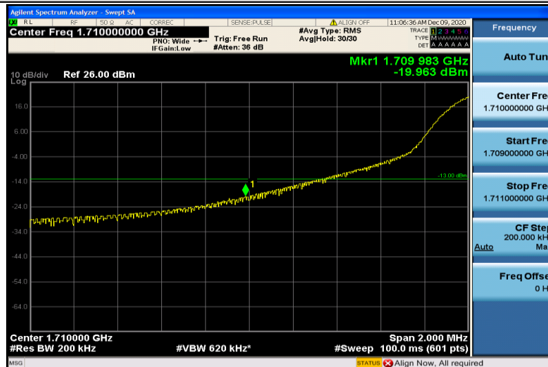
Band66-20MHz-16QAM-132072-1RB#0
