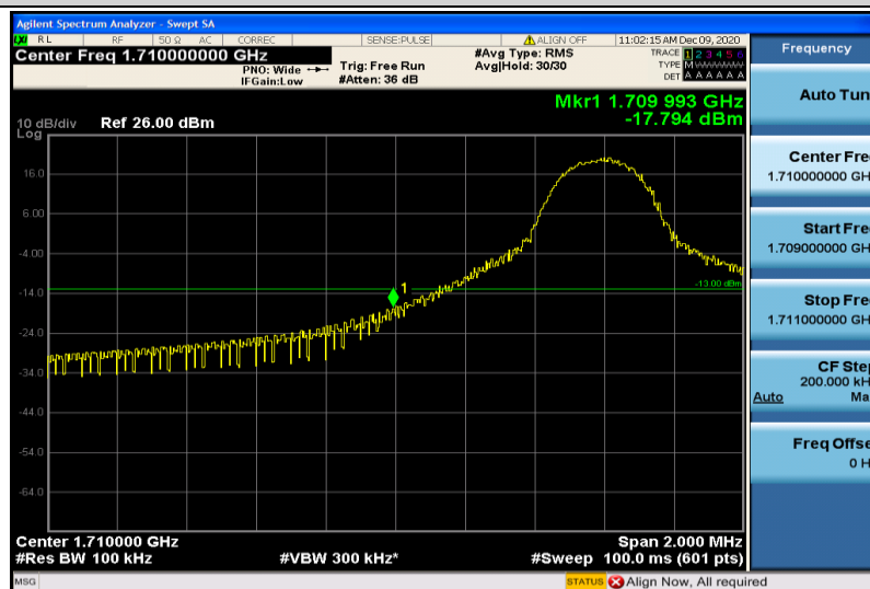
Band66-10MHz-16QAM-132022-1RB#0
