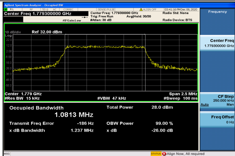
Band66-1.4MHz-16QAM-132665-6RB#0-1.0813
