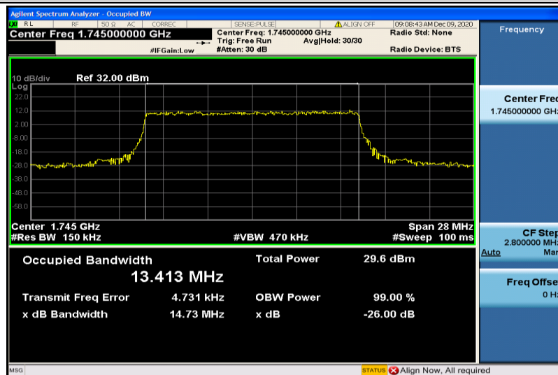
Band66-15MHz-QPSK-132322-75RB#0-13.413
