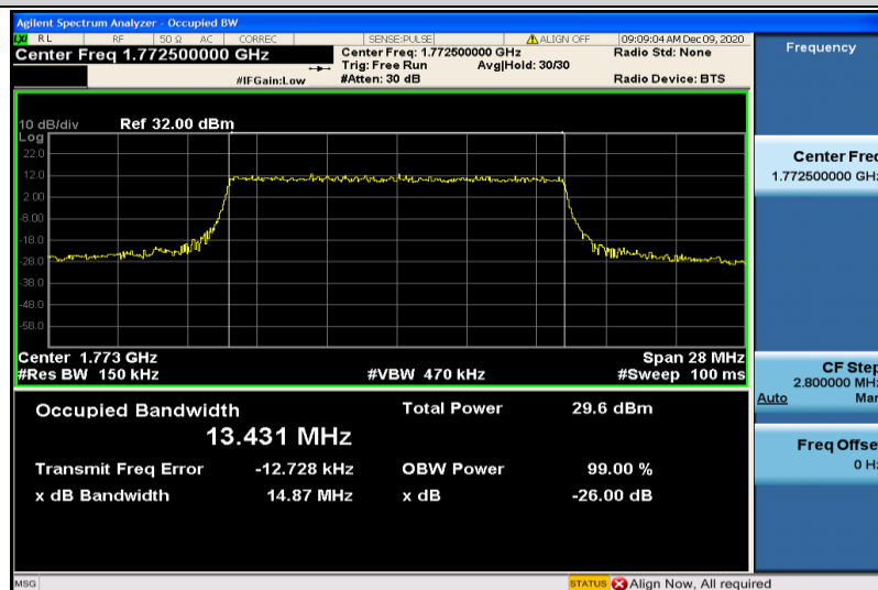
Band66-15MHz-QPSK-132597-75RB#0-13.431
