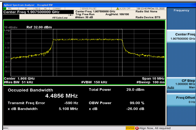
Band2-5MHz-QPSK-19175-25RB#0-4.4856
