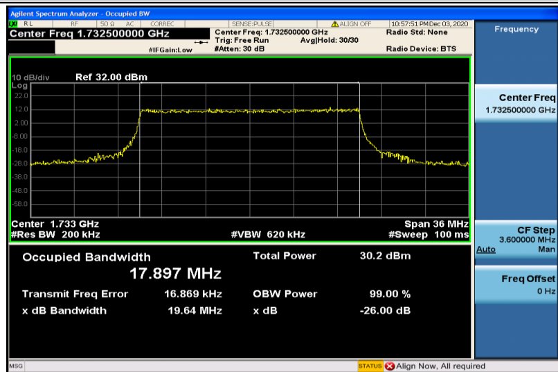
Band4-20MHz-QPSK-20175-100RB#0-17.897
