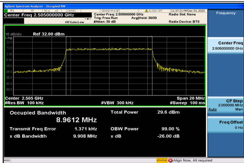
Band7-10MHz-QPSK-20800-50RB#0-8.9612
