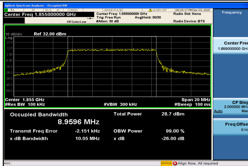
Band2-10MHz-16QAM-18650-50RB#0-8.9596
