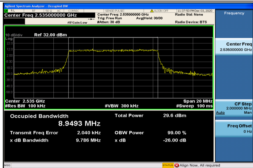
Band7-10MHz-QPSK-21100-50RB#0-8.9493
