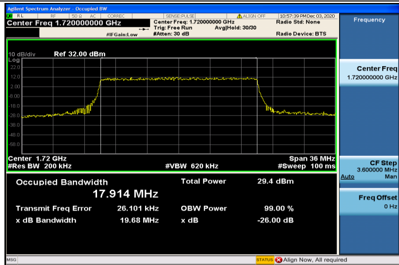
Band4-20MHz-16QAM-20050-100RB#0-17.914
