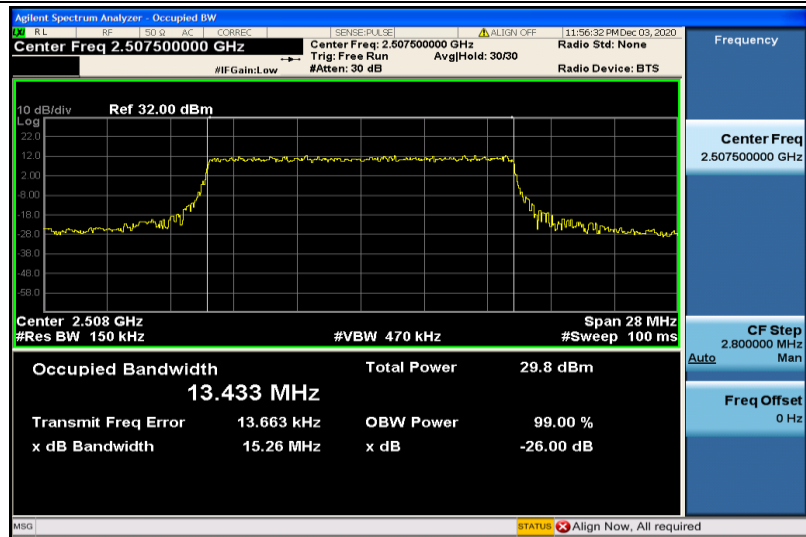
Band7-15MHz-QPSK-20825-75RB#0-13.433
