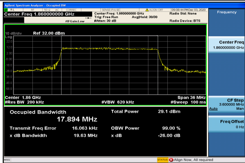
Band2-20MHz-16QAM-18700-100RB#0-17.894
