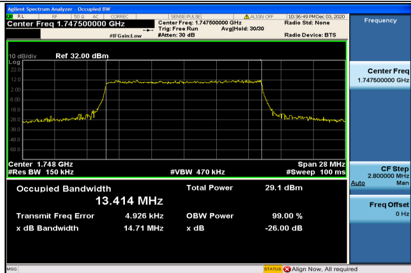
Band4-15MHz-16QAM-20325-75RB#0-13.414
