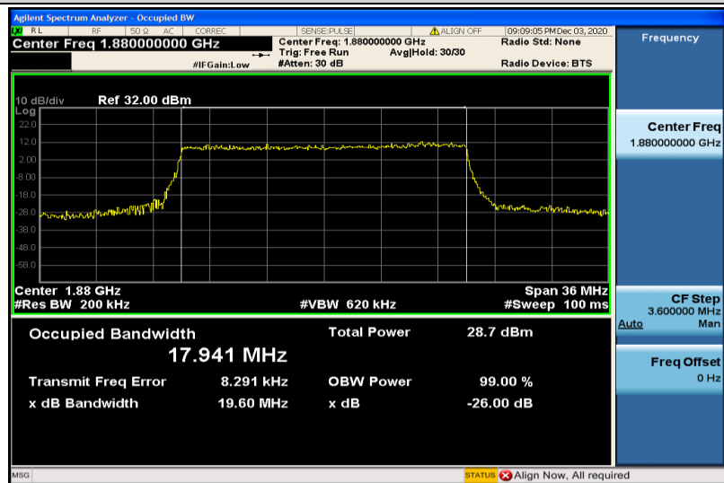
Band2-20MHz-16QAM-18900-100RB#0-17.941
