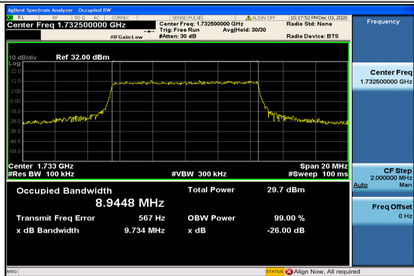
Band4-10MHz-QPSK-20175-50RB#0-8.9448
