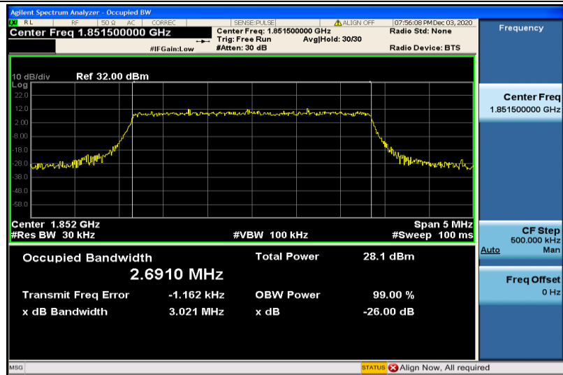
Band2-3MHz-16QAM-18615-15RB#0-2.6910
