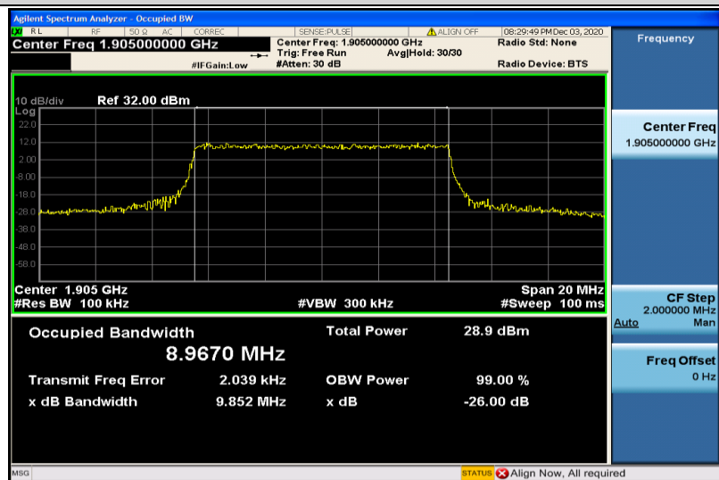
Band2-10MHz-QPSK-19150-50RB#0-8.9670
