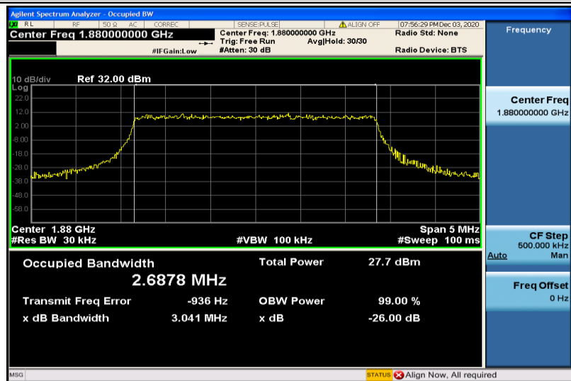
Band2-3MHz-16QAM-18900-15RB#0-2.6878
