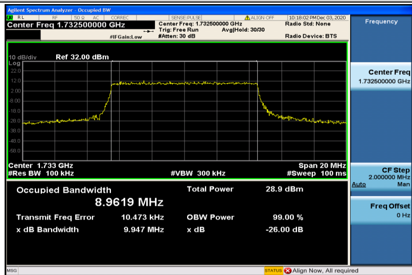
Band4-10MHz-16QAM-20175-50RB#0-8.9619
