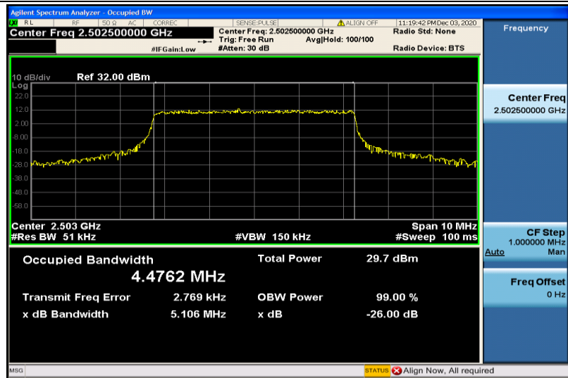
Band7-5MHz-QPSK-20775-25RB#0-4.4762
