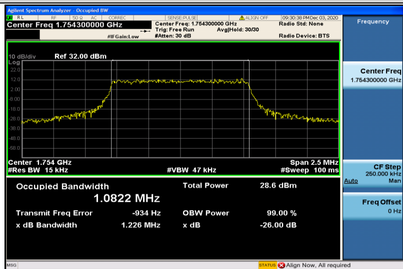
Band4-1.4MHz-QPSK-20393-6RB#0-1.0822
