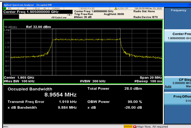
Band2-10MHz-16QAM-19150-50RB#0-8.9554
