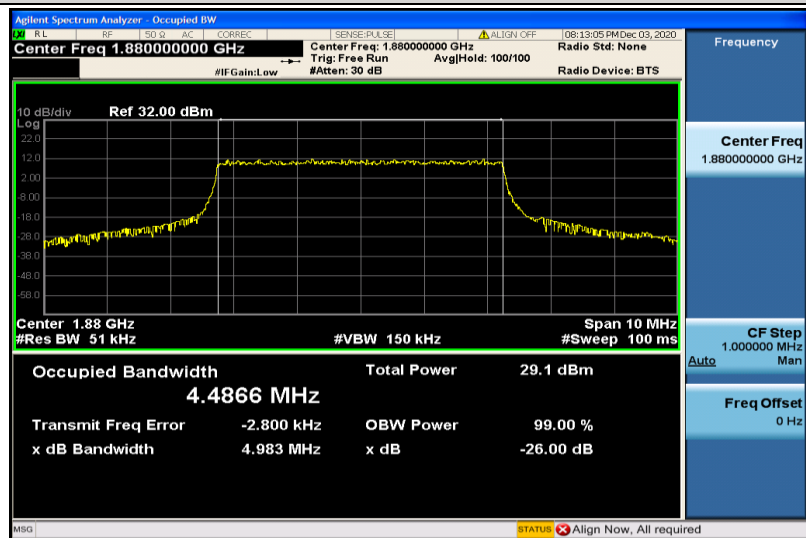
Band2-5MHz-QPSK-18900-25RB#0-4.4866
