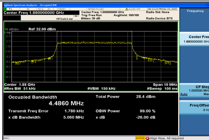
Band2-5MHz-16QAM-18900-25RB#0-4.4860
