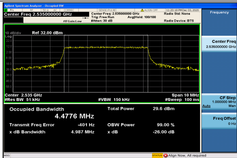
Band7-5MHz-QPSK-21100-25RB#0-4.4776
