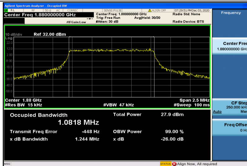
Band2-1.4MHz-QPSK-18900-6RB#0-1.0818
