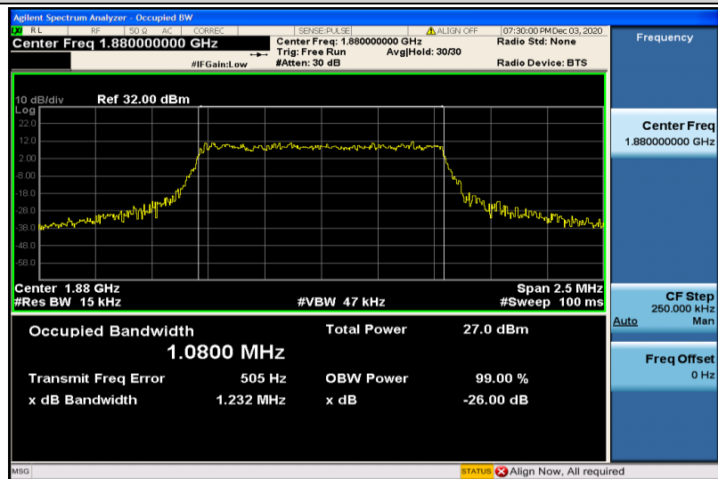
Band2-1.4MHz-16QAM-18900-6RB#0-1.0800
