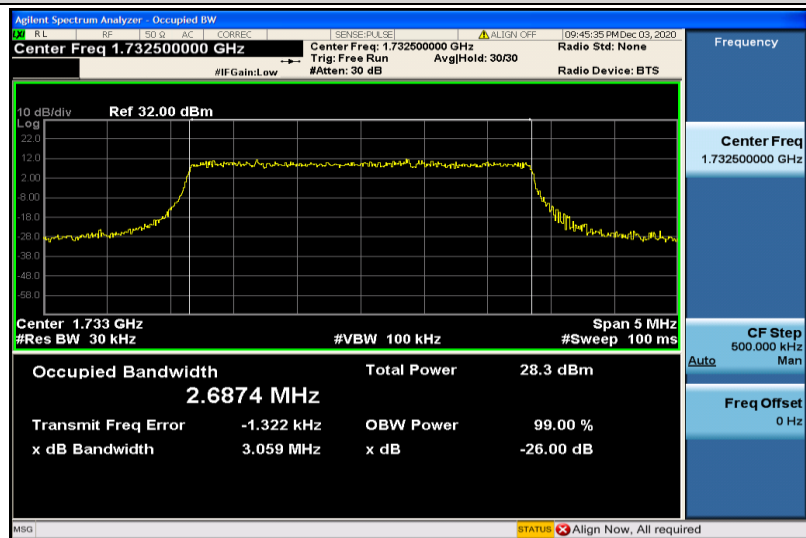
Band4-3MHz-16QAM-20175-15RB#0-2.6874
