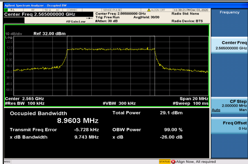
Band7-10MHz-16QAM-21400-50RB#0-8.9603
