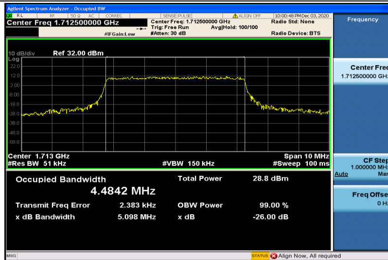
Band4-5MHz-16QAM-19975-25RB#0-4.4842
