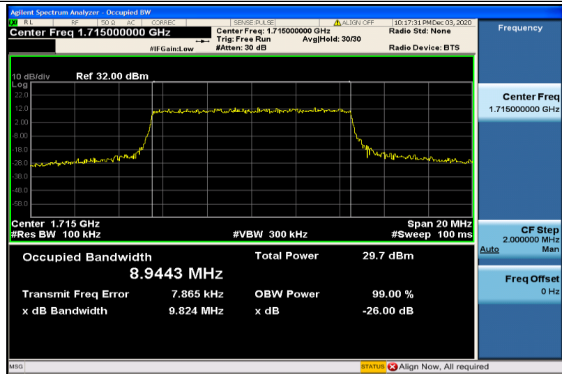
Band4-10MHz-QPSK-20000-50RB#0-8.9443
