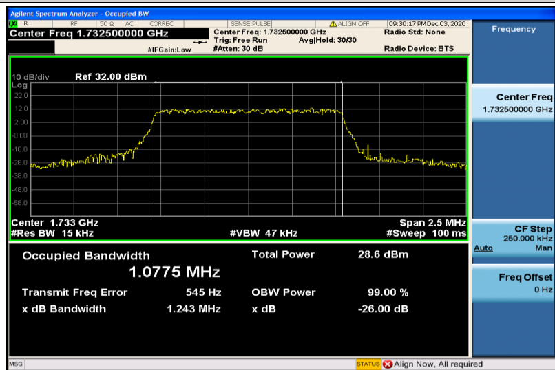
Band4-1.4MHz-QPSK-20175-6RB#0-1.0775
