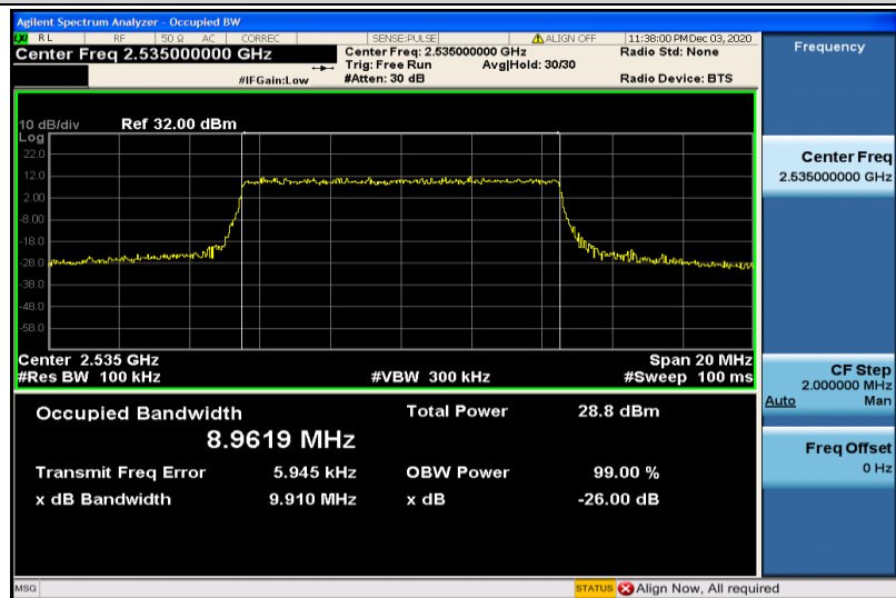
Band7-10MHz-16QAM-21100-50RB#0-8.9619
