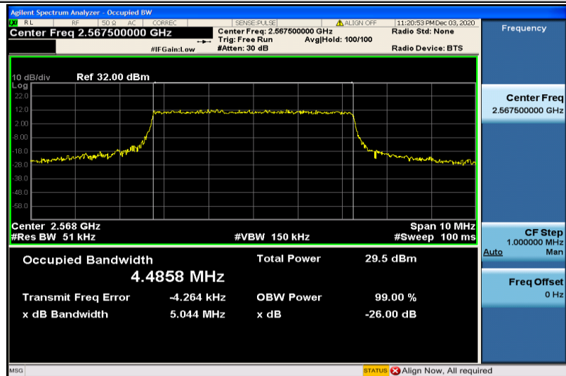
Band7-5MHz-QPSK-21425-25RB#0-4.4858
