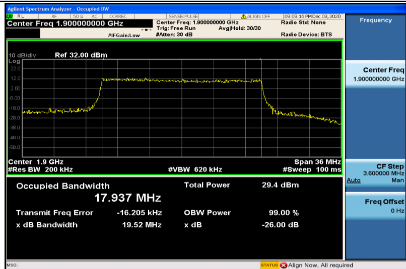
Band2-20MHz-QPSK-19100-100RB#0-17.937
