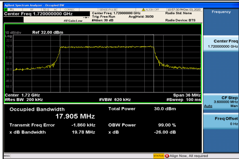
Band4-20MHz-QPSK-20050-100RB#0-17.905
