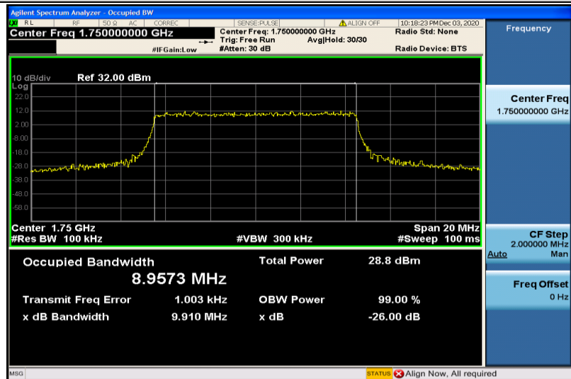
Band4-10MHz-16QAM-20350-50RB#0-8.9573
