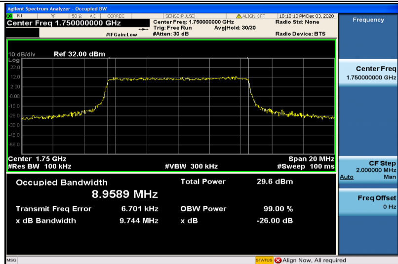
Band4-10MHz-QPSK-20350-50RB#0-8.9589
