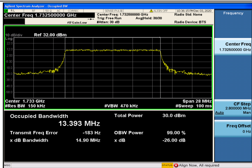
Band4-15MHz-QPSK-20175-75RB#0-13.393
