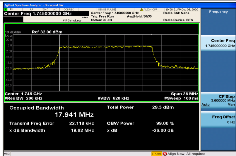
Band4-20MHz-16QAM-20300-100RB#0-17.941
