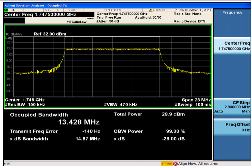
Band4-15MHz-QPSK-20325-75RB#0-13.428
