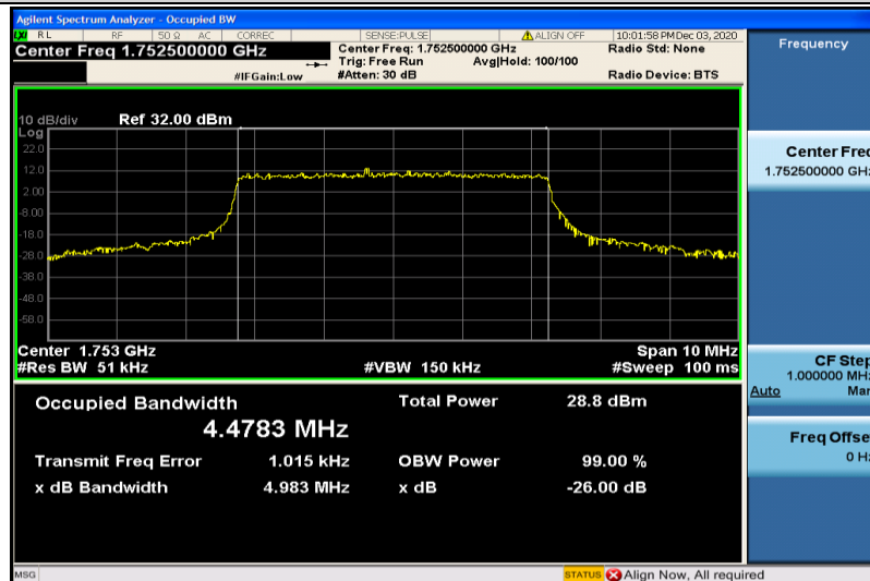
Band4-5MHz-16QAM-20375-25RB#0-4.4783
