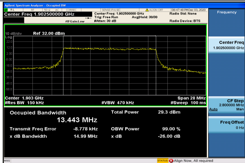
Band2-15MHz-QPSK-19125-75RB#0-13.443
