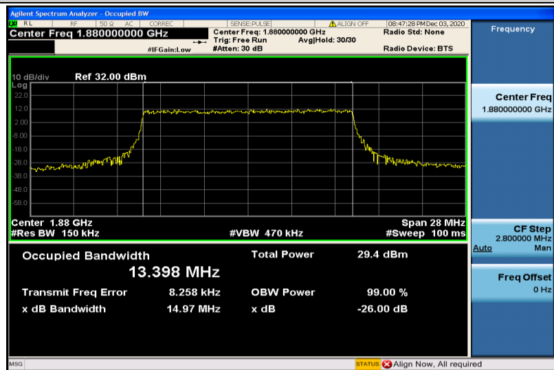
Band2-15MHz-QPSK-18900-75RB#0-13.398
