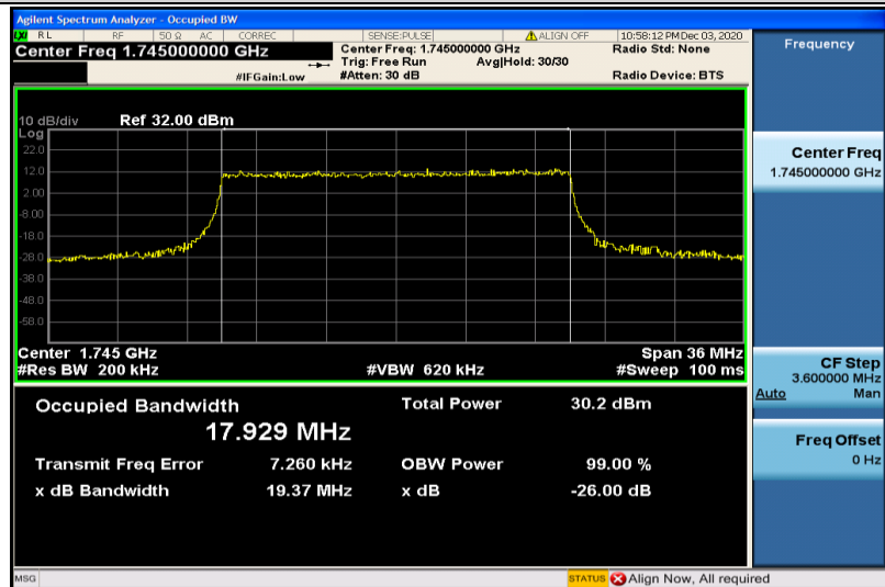
Band4-20MHz-QPSK-20300-100RB#0-17.929
