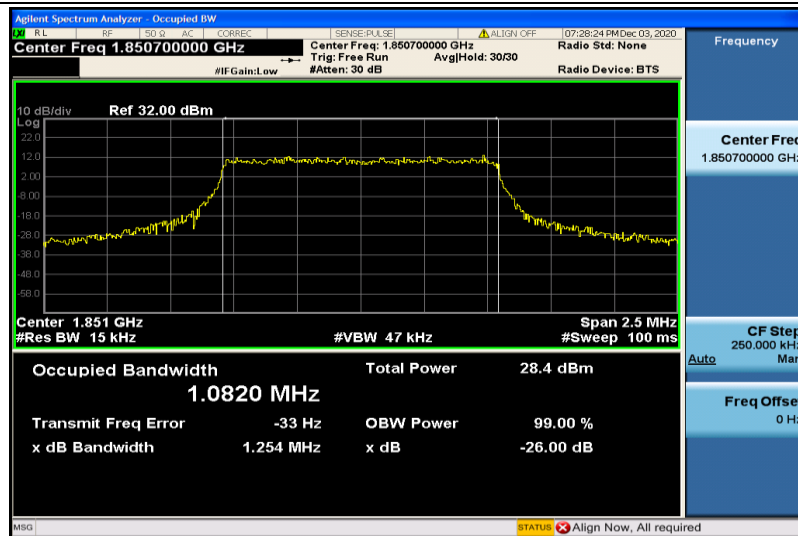
Band2-1.4MHz-QPSK-18607-6RB#0-1.0820
