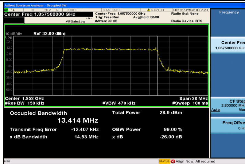
Band2-15MHz-16QAM-18675-75RB#0-13.414
