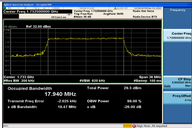
Band4-20MHz-16QAM-20175-100RB#0-17.940
