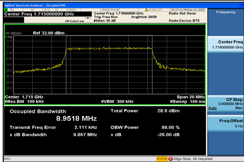
Band4-10MHz-16QAM-20000-50RB#0-8.9518
