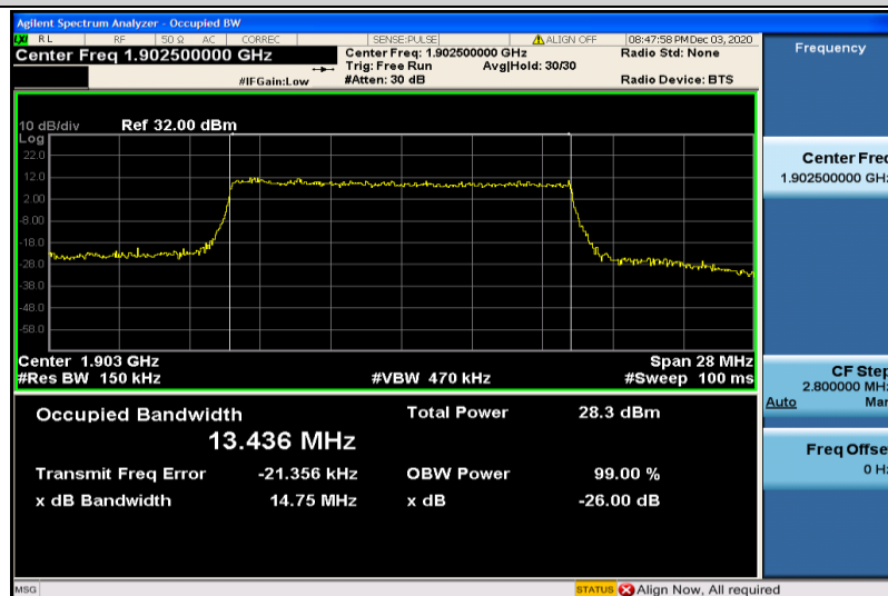
Band2-15MHz-16QAM-19125-75RB#0-13.436
