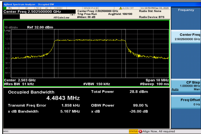
Band7-5MHz-16QAM-20775-25RB#0-4.4843
