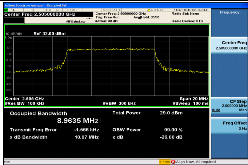
Band7-10MHz-16QAM-20800-50RB#0-8.9635
