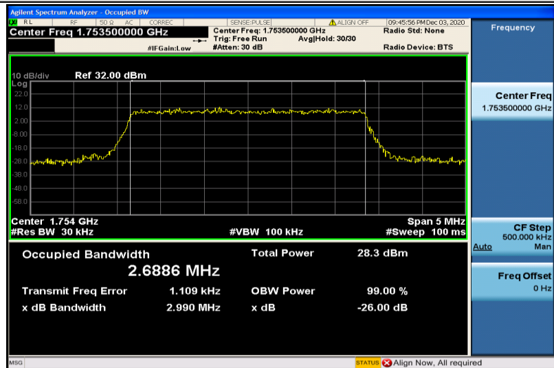
Band4-3MHz-16QAM-20385-15RB#0-2.6886
