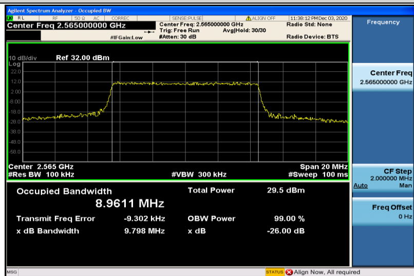
Band7-10MHz-QPSK-21400-50RB#0-8.9611
