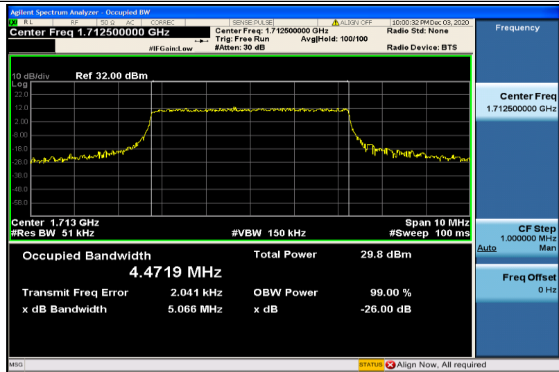
Band4-5MHz-QPSK-19975-25RB#0-4.4719
