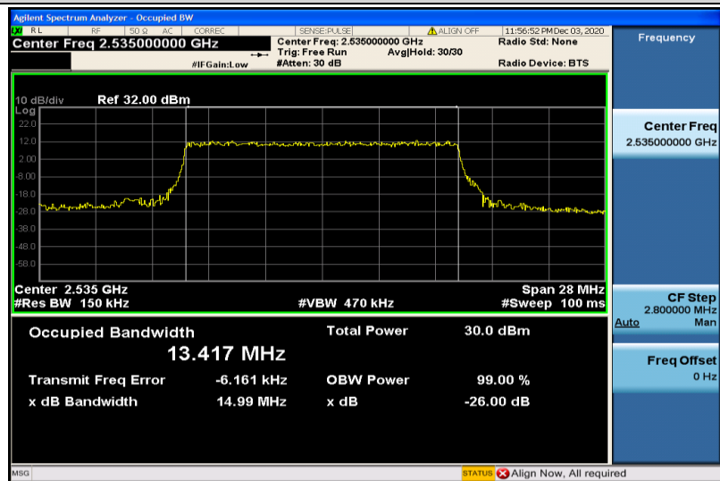
Band7-15MHz-QPSK-21100-75RB#0-13.417
