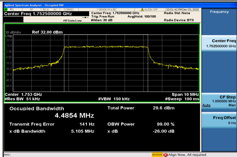
Band4-5MHz-QPSK-20375-25RB#0-4.4854
