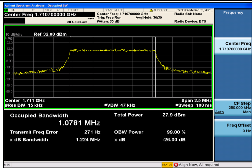
Band4-1.4MHz-16QAM-19957-6RB#0-1.0781
