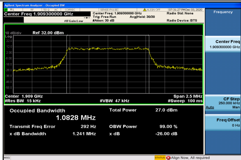
Band2-1.4MHz-16QAM-19193-6RB#0-1.0828
