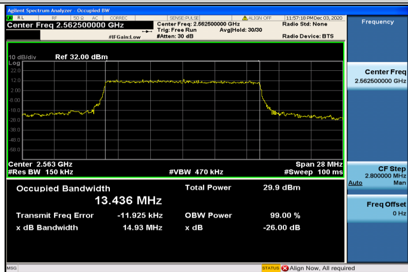
Band7-15MHz-QPSK-21375-75RB#0-13.436
