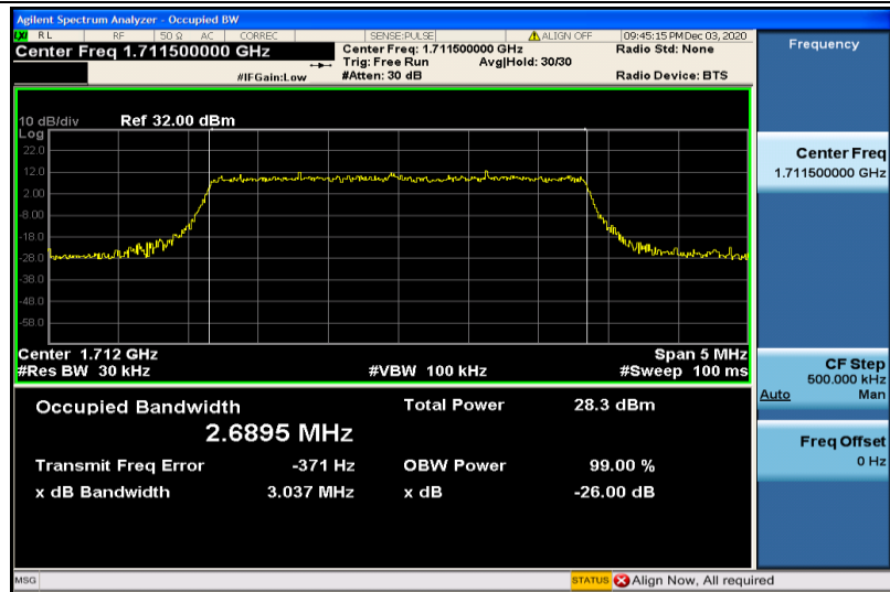
Band4-3MHz-16QAM-19965-15RB#0-2.6895
