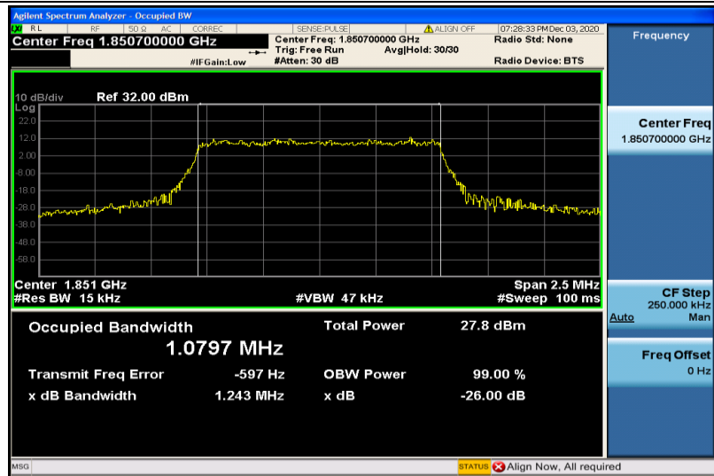
Band2-1.4MHz-16QAM-18607-6RB#0-1.0797
