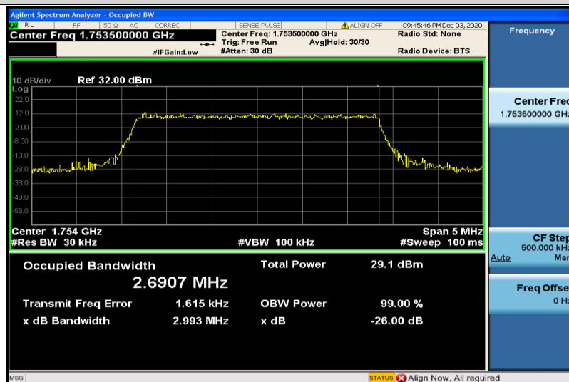
Band4-3MHz-QPSK-20385-15RB#0-2.6907
