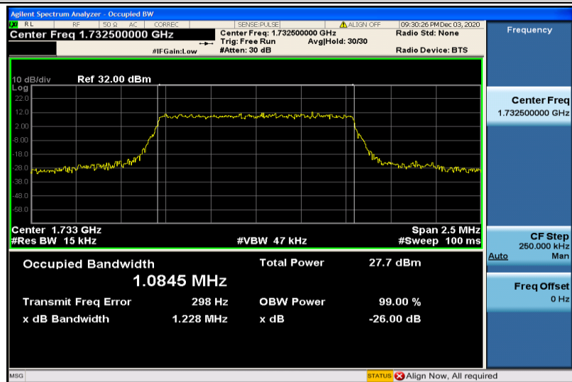
Band4-1.4MHz-16QAM-20175-6RB#0-1.0845
