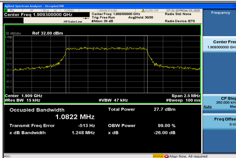
Band2-1.4MHz-QPSK-19193-6RB#0-1.0822
