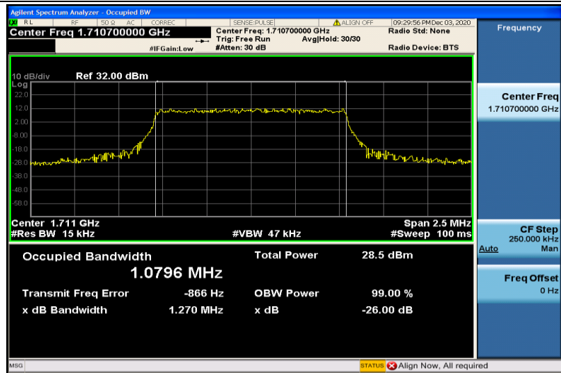
Band4-1.4MHz-QPSK-19957-6RB#0-1.0796
