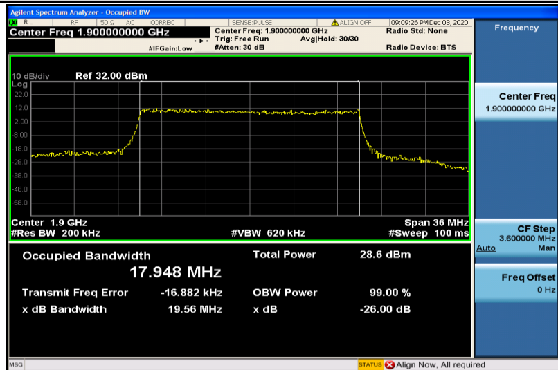
Band2-20MHz-16QAM-19100-100RB#0-17.948
