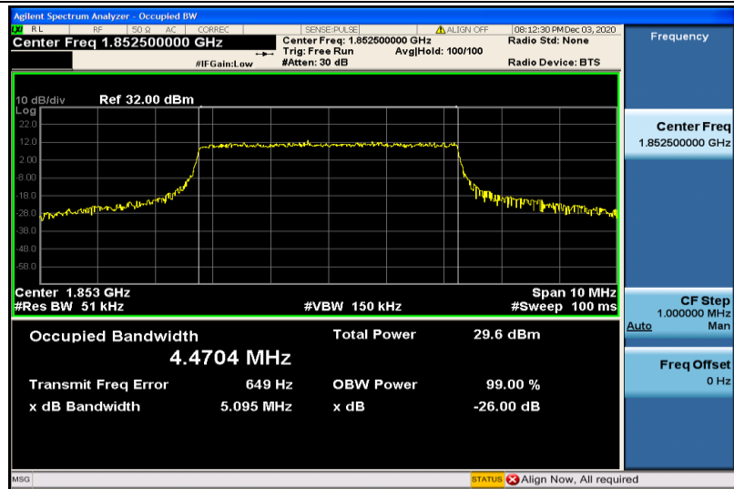
Band2-5MHz-QPSK-18625-25RB#0-4.4704
