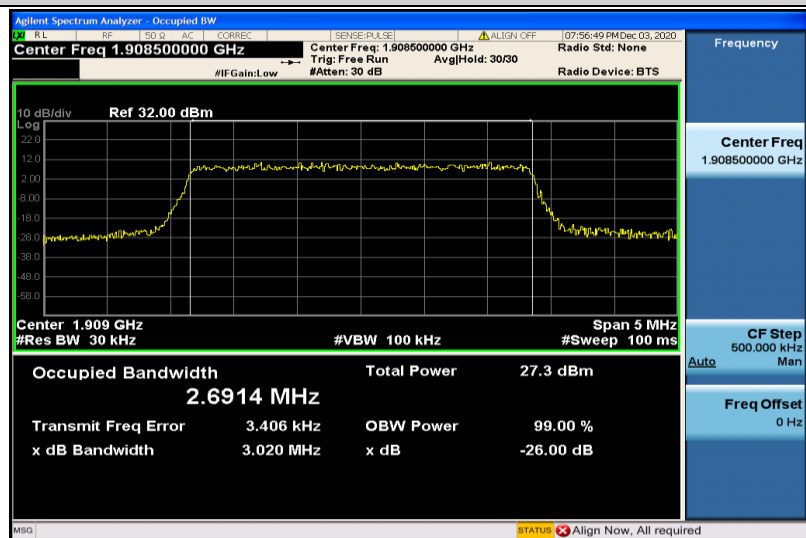
Band2-3MHz-16QAM-19185-15RB#0-2.6914
