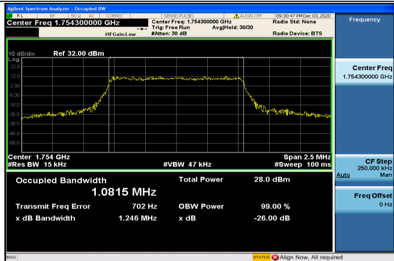
Band4-1.4MHz-16QAM-20393-6RB#0-1.0815
