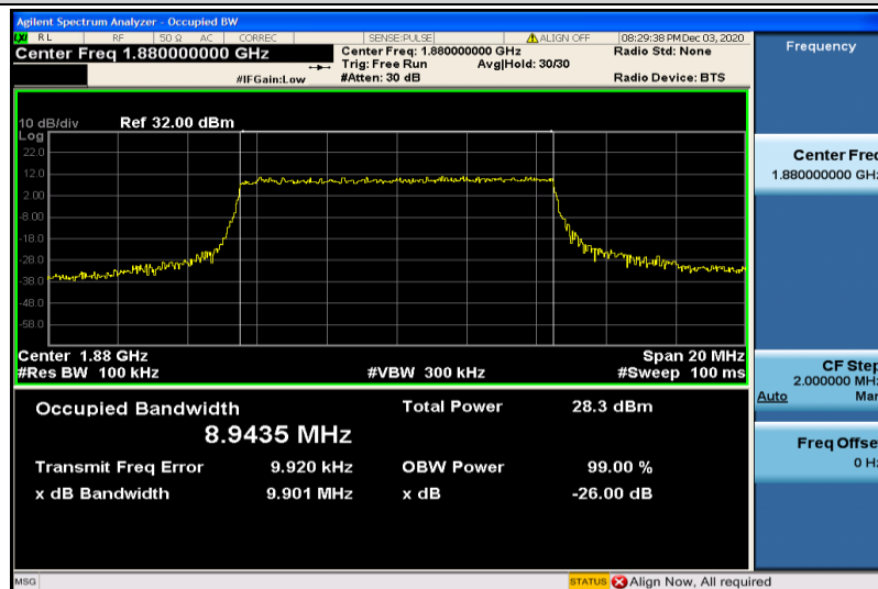
Band2-10MHz-16QAM-18900-50RB#0-8.9435
