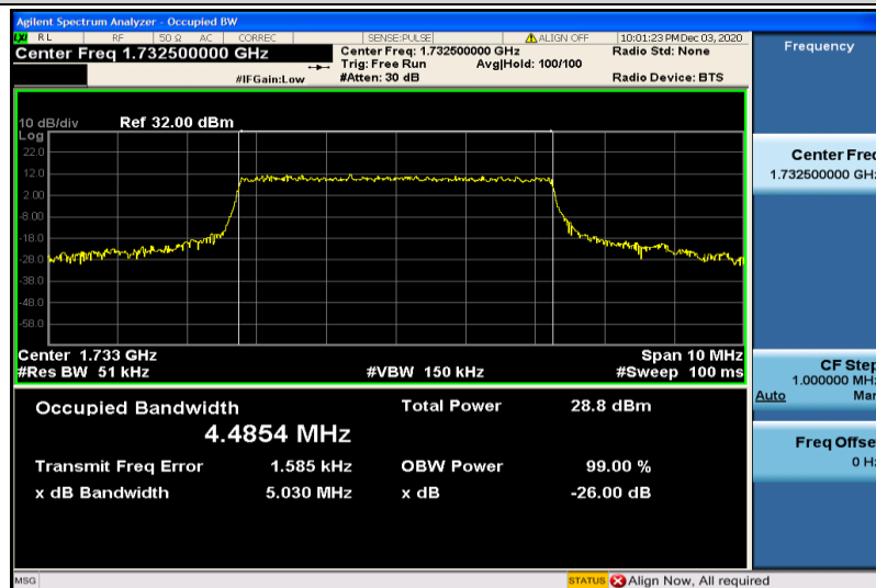
Band4-5MHz-16QAM-20175-25RB#0-4.4854
