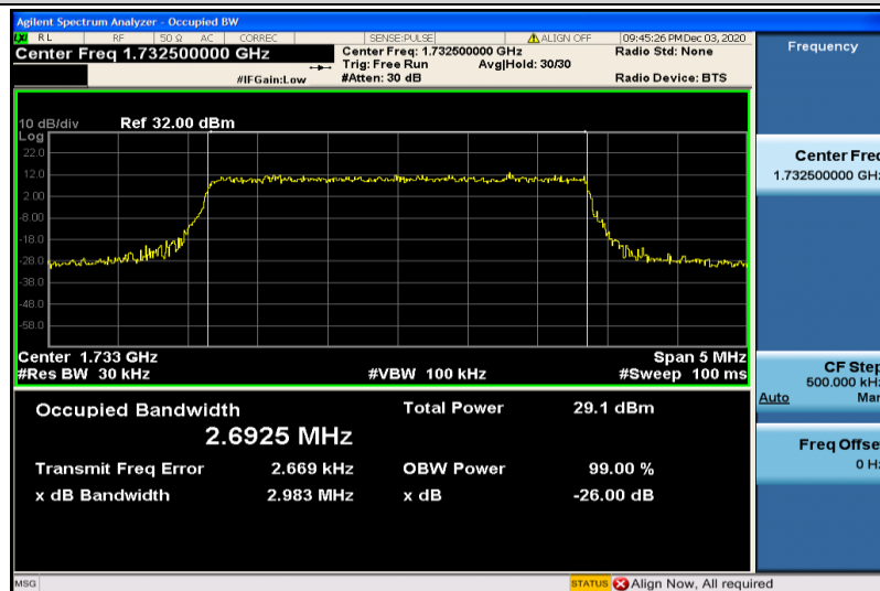
Band4-3MHz-QPSK-20175-15RB#0-2.6925
