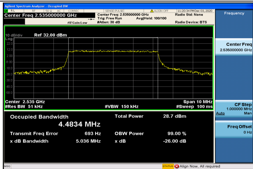
Band7-5MHz-16QAM-21100-25RB#0-4.4834
