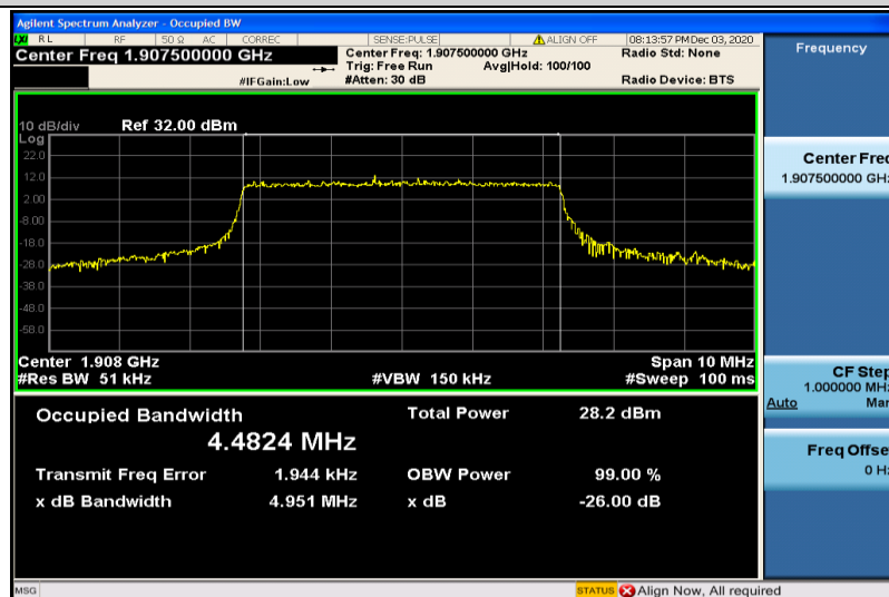
Band2-5MHz-16QAM-19175-25RB#0-4.4824
