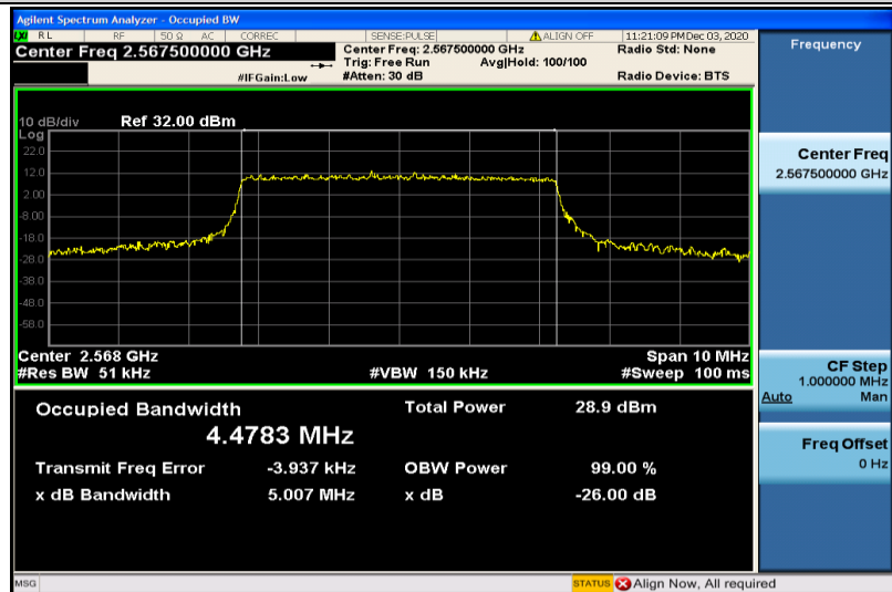
Band7-5MHz-16QAM-21425-25RB#0-4.4783
