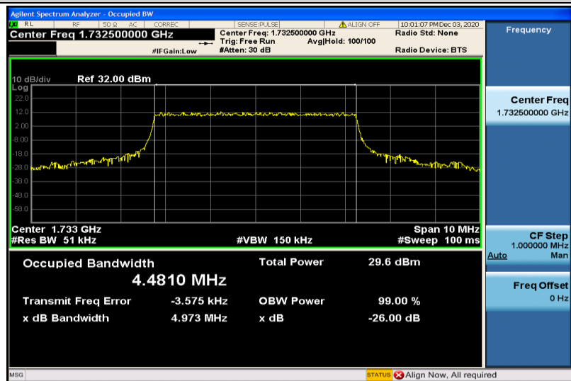
Band4-5MHz-QPSK-20175-25RB#0-4.4810
