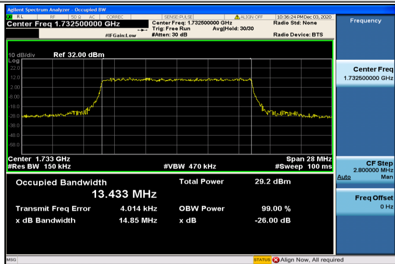
Band4-15MHz-16QAM-20175-75RB#0-13.433
