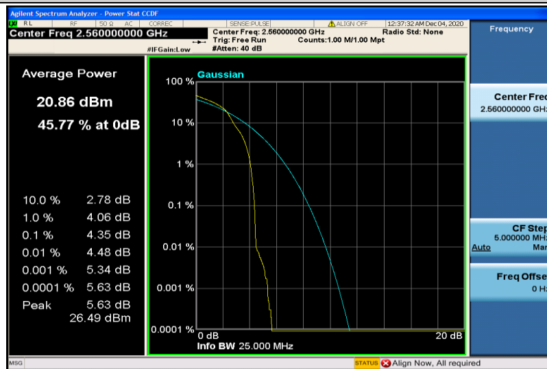
Band7-20MHz-16QAM-21350-1R#0
