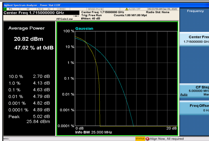
Band66-10MHz-16QAM-132022-1RB#0
