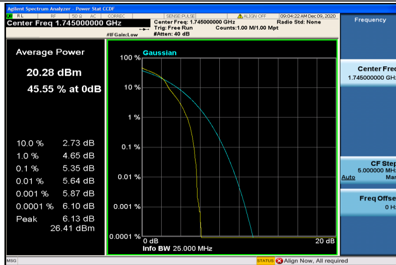
Band66-10MHz-16QAM-132322-1RB#0
