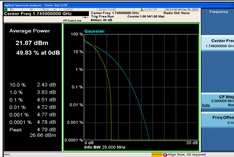
Band66-15MHz-QPSK-132322-1RB#0
