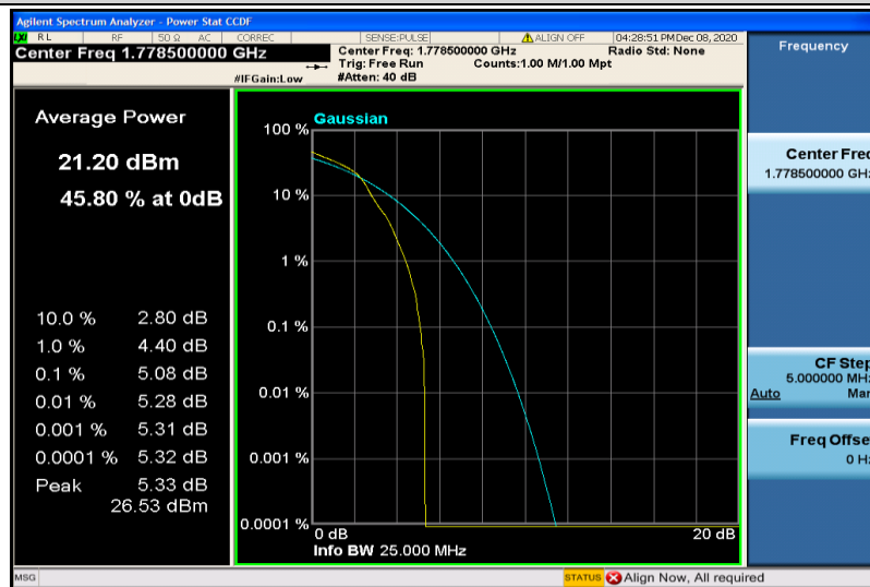
Band66-3MHz-16QAM-132657-1RB#0
