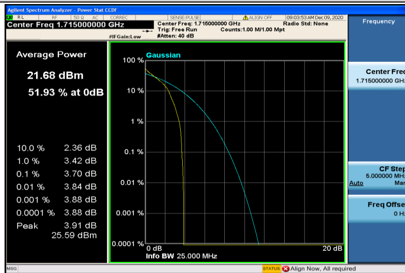
Band66-10MHz-QPSK-132022-1RB#0
