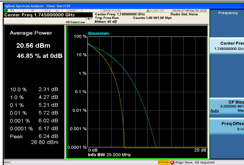
Band66-10MHz-QPSK-132322-50RB#0
