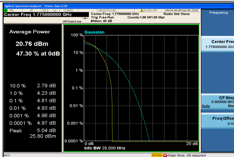
Band66-10MHz-16QAM-132622-1RB#0
