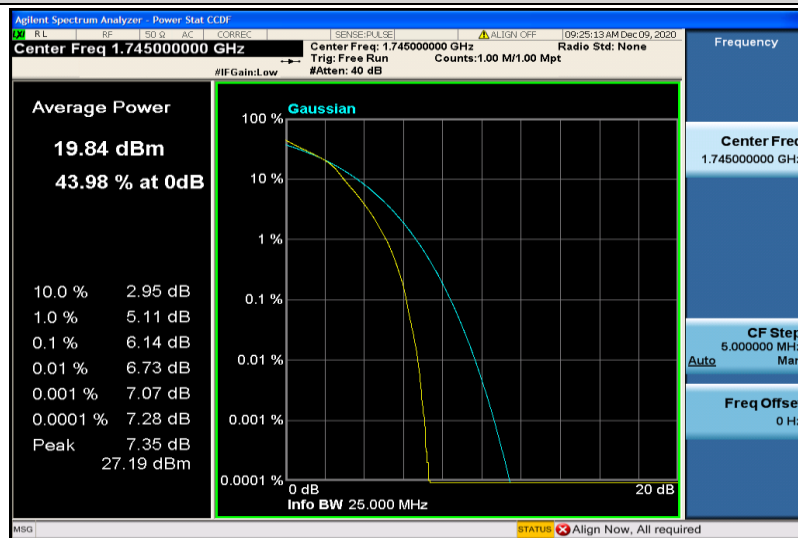
Band66-15MHz-16QAM-132322-75RB#0
