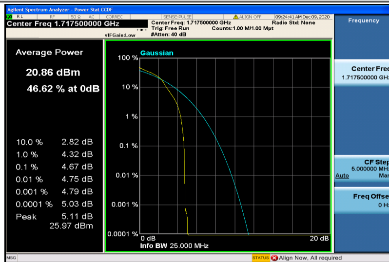
Band66-15MHz-16QAM-132047-1RB#0
