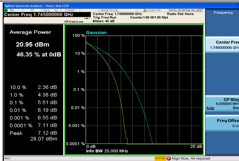
Band66-20MHz-QPSK-132322-100RB#0
