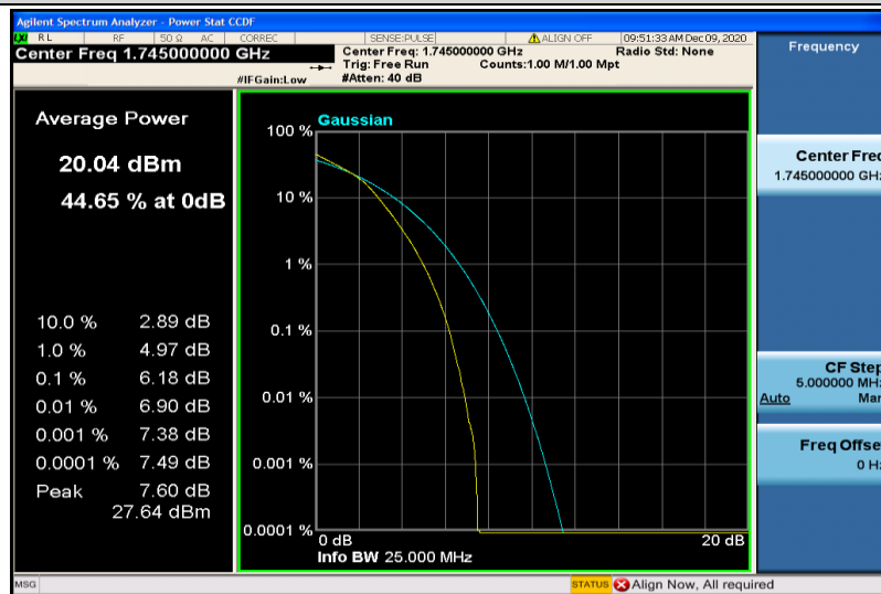
Band66-20MHz-16QAM-132322-100RB#0
