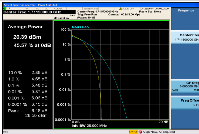
Band66-3MHz-16QAM-131987-15RB#0
