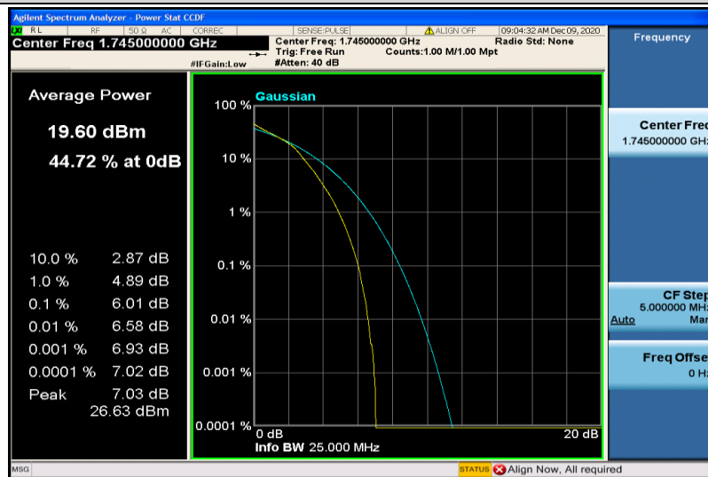
Band66-10MHz-16QAM-132322-50RB#0
