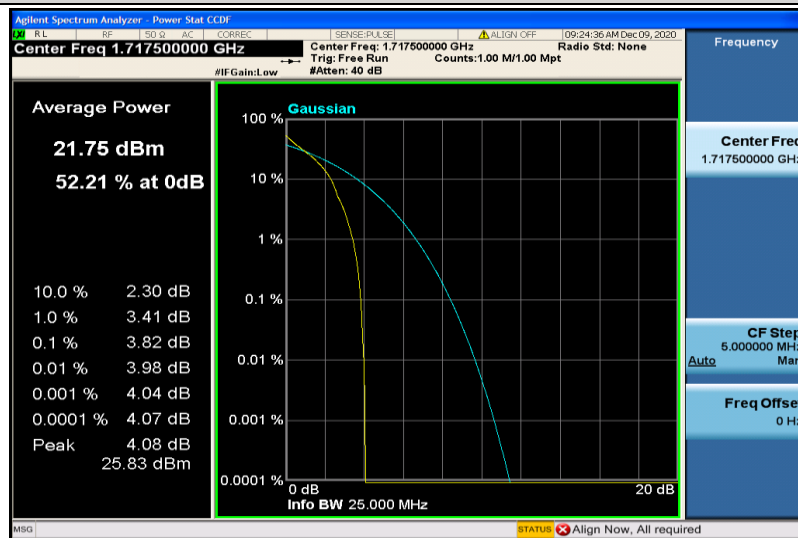
Band66-15MHz-QPSK-132047-1RB#0
