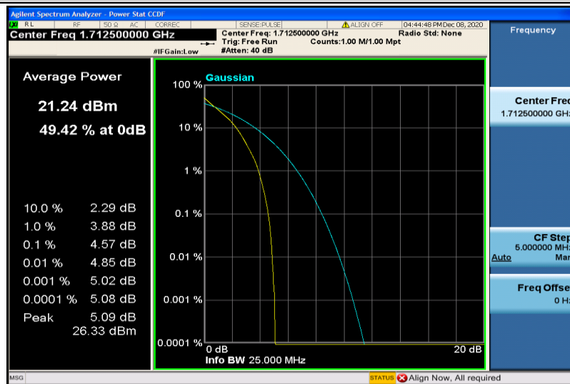
Band66-5MHz-QPSK-131997-25RB#0
