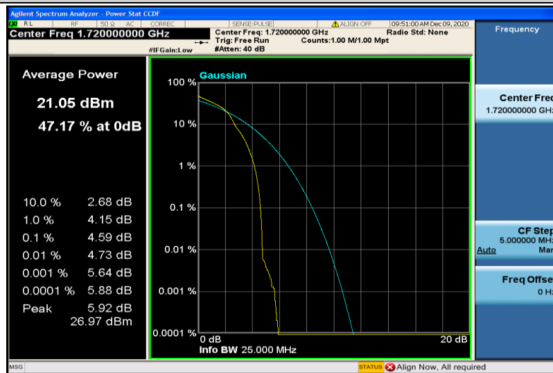
Band66-20MHz-16QAM-132072-1RB#0
