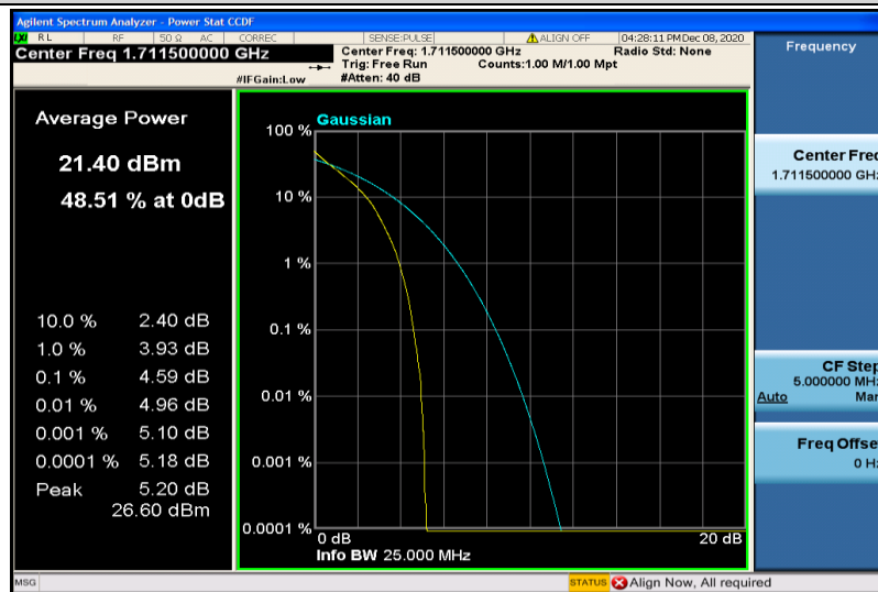
Band66-3MHz-QPSK-131987-15RB#0
