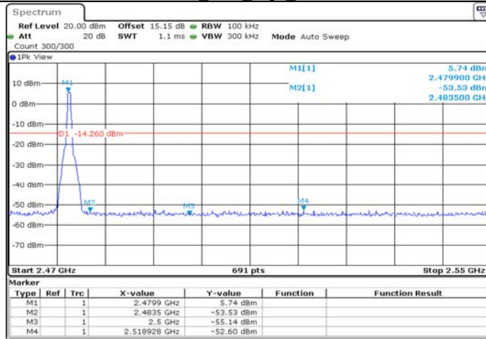
DH1_Ant1_High_2480
