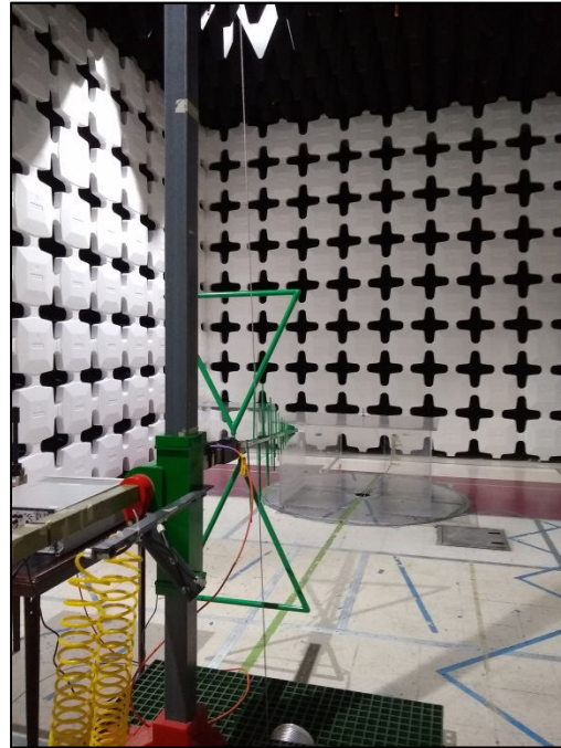
Photograph 1: Radiated Spurious Emissions, Below 1GHz, Whip Antenna Test Setup
