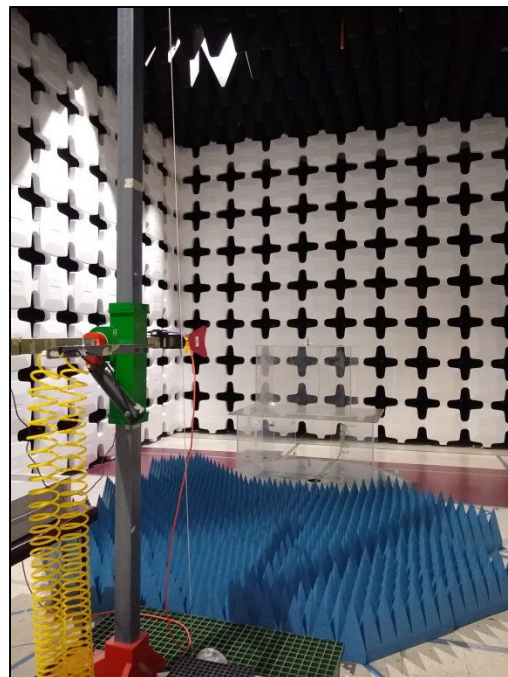
Photograph 2: Radiated Spurious Emissions, Above 1GHz, Whip Antenna Test Setup
