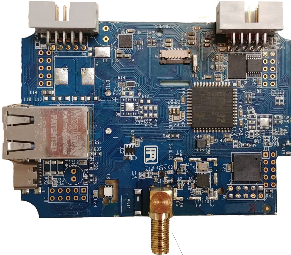
Whip Antenna
